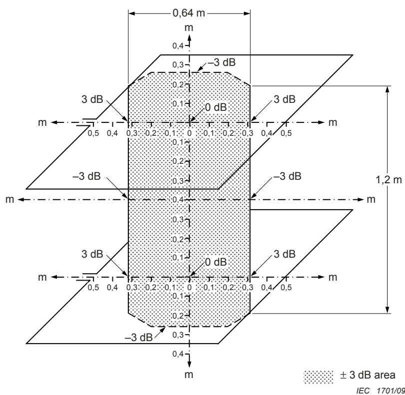
Figure B.5 – 3 dB area of the field generated by two square inductive coils (1 m side) 0,8 m spaced, in the mean orthogonal plane (component orthogonal to the plane of the coils)
