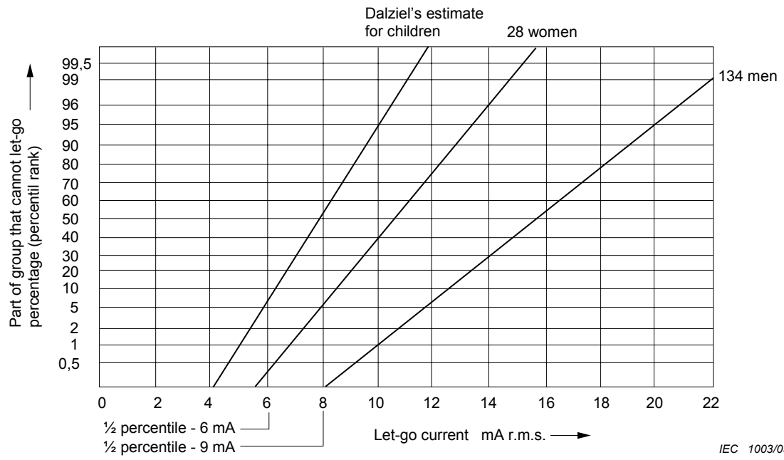
Figure 23 – Let-go currents for 60 Hz sinusoidal current
