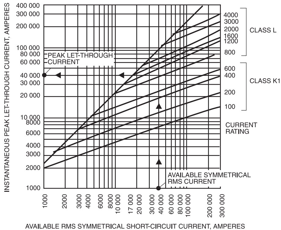
Figure 9-24—Typical 60 Hz peak let-through current as a function of available rms symmetrical current; power factor below 20%
