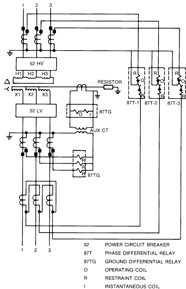
Figure 11-24—Transformer phase and ground differential relay CT and current coil connections
