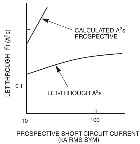
Figure 7-9b—Limited let-through I^2t characteristics
