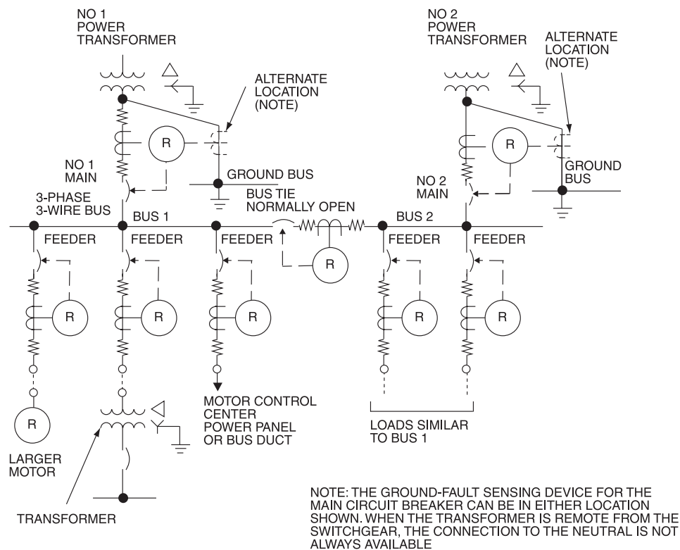
Figure 8-19—Three-wire solidly grounded secondary selective system
