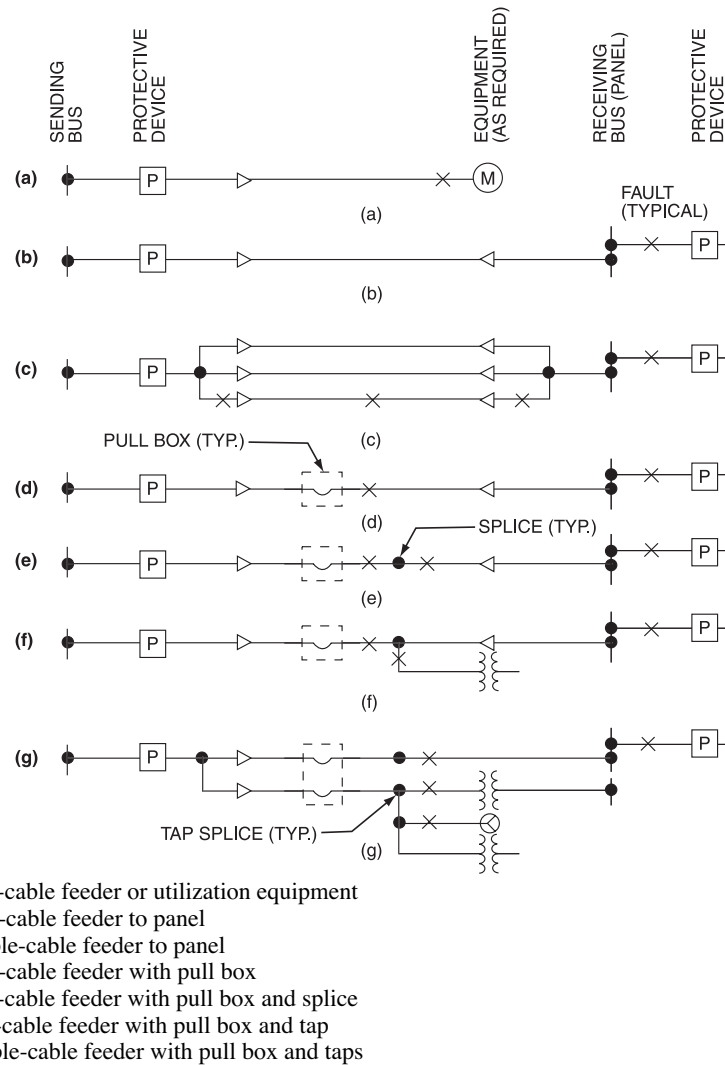
Figure 9-8—Application of protective devices
