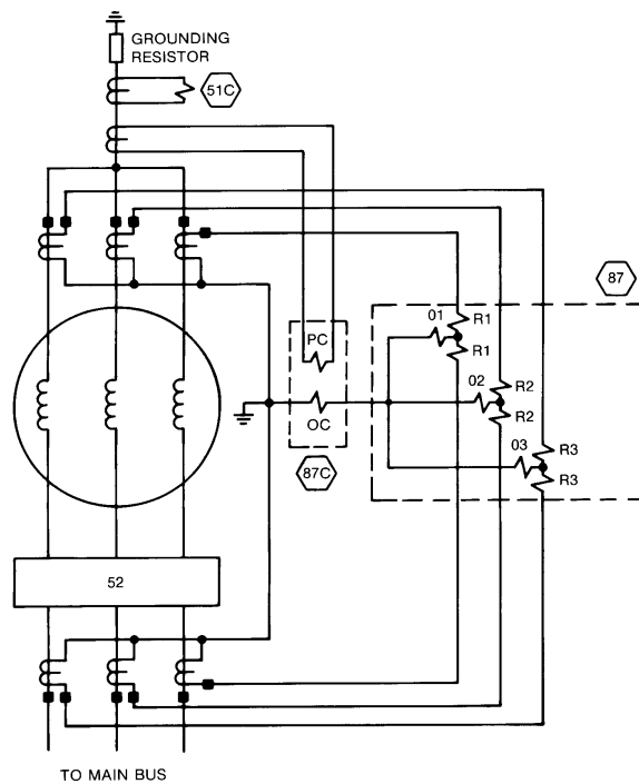
Figure 12-10—Generator percentage differential relay (phase scheme) and ground differential scheme using a directional relay
