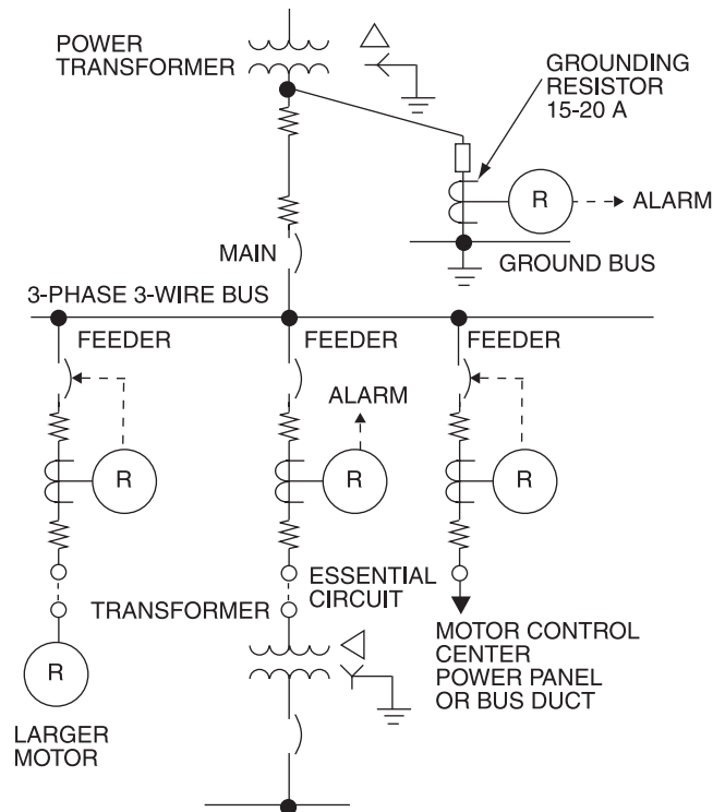
Figure 8-20—Three-wire high-resistance-grounded system
