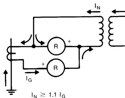
Figure 11-30—Relay current during external fault when auxiliary CT ratio is selected to restrain
