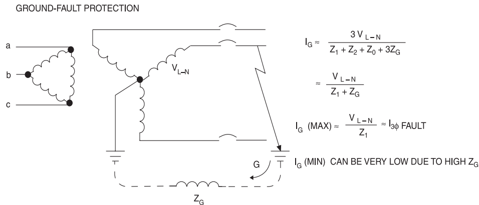
Figure 8-2—Direct or solid grounding (uses ground relays to trip)
