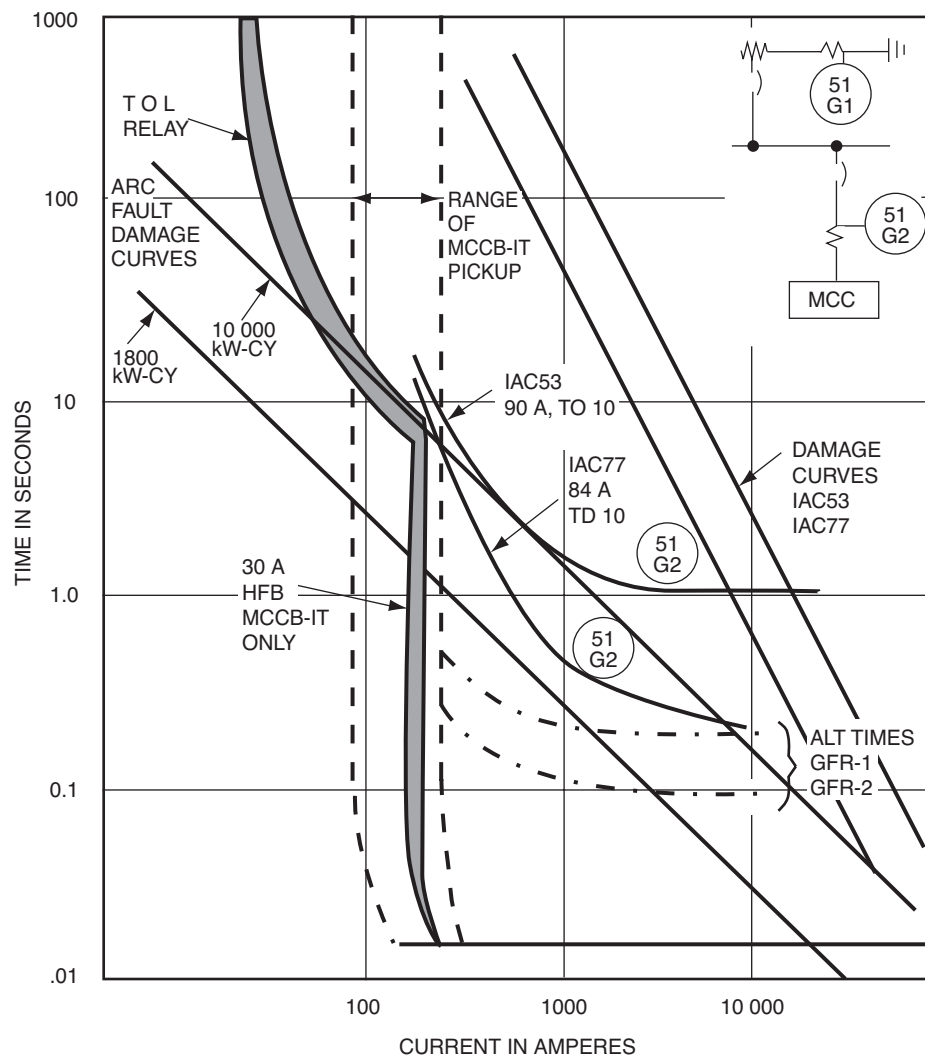
Figure 8-15d—Ground-fault protection for an 11 kW motor load
