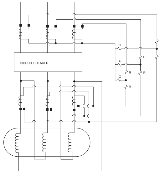
Figure 12-13—Percentage differential relay connection for delta-connected generator
