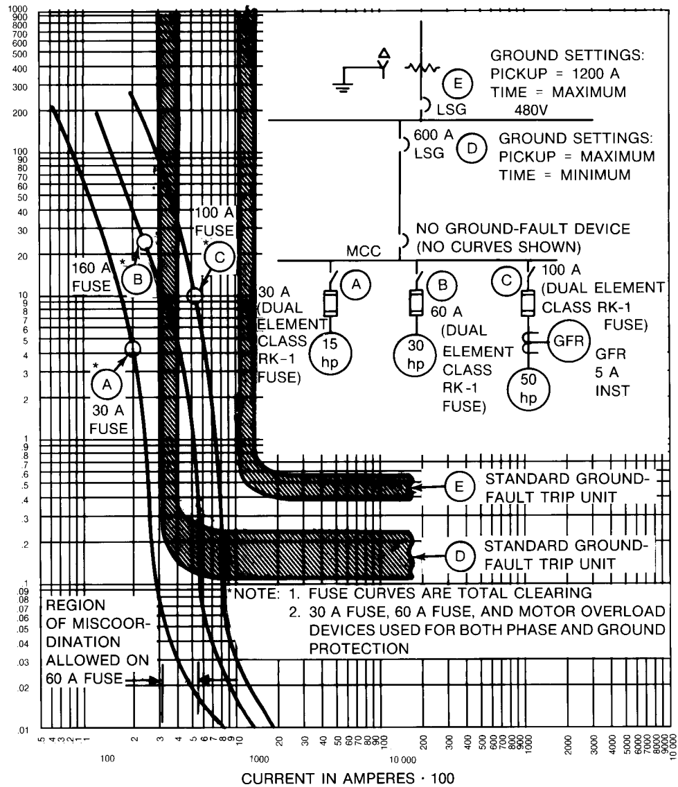
Figure 15-25—Ground-fault TCC curves Example 1
