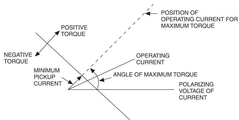
Figure 4-24—Characteristics of a directional element
