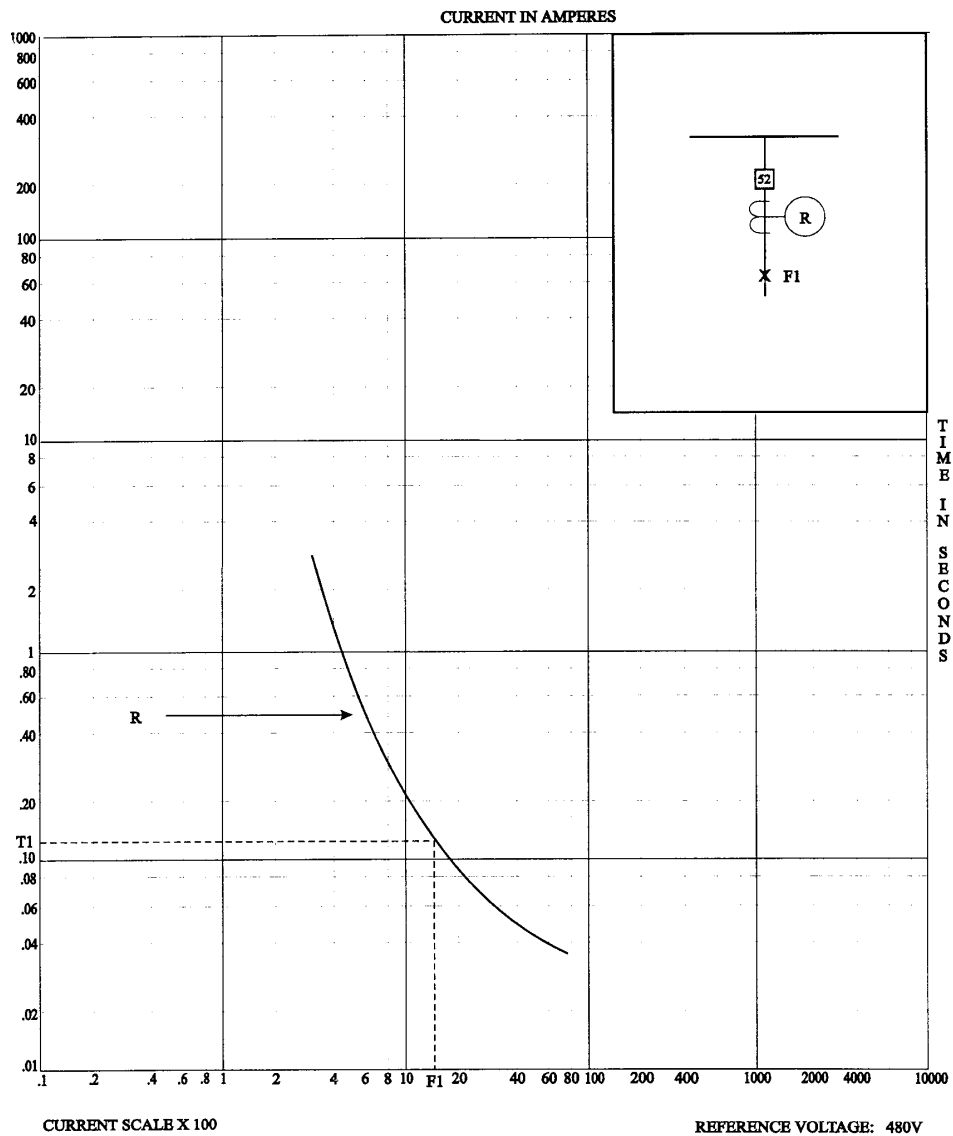
Figure 15-5a—Overcurrent trip time characteristic for a given fault for a protective relay
