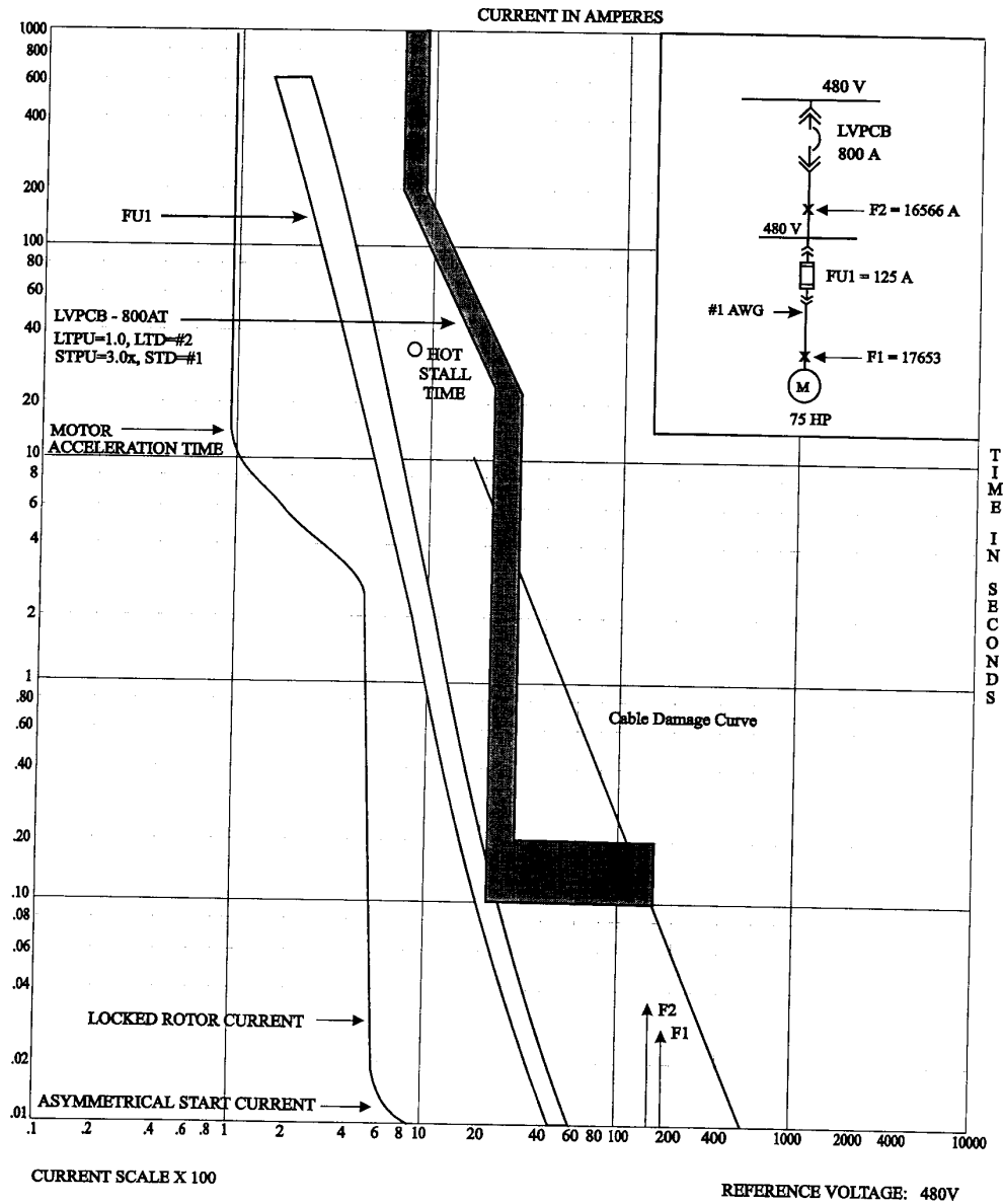
Figure 15-15—480 V feeder circuit breaker coordination plot
