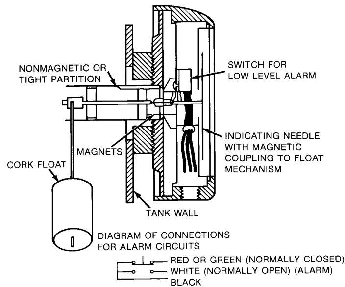
Figure 11-6—Liquid-level-indicating needle, driven by a magnetic coupling to the float mechanism
