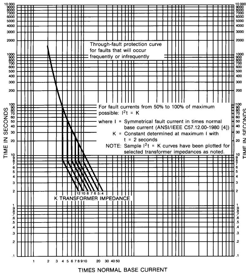
Figure 11-22—Through-fault protection curve for liquid-immersed Category IV transformers (above 10 000 kVA single-phase, above 30 000 kVA three-phase)
