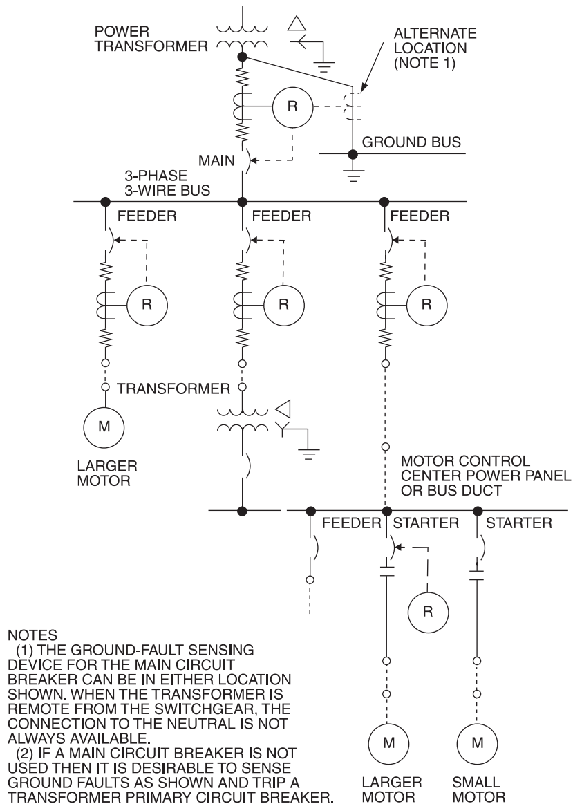
Figure 8-17—Three-wire solidly grounded system with single supply
