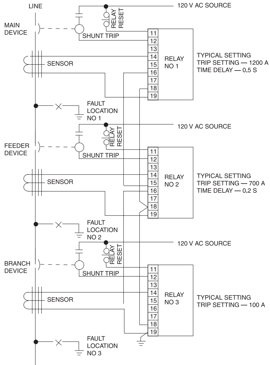
Figure 8-15a—Typical zone selective interlocking (ZSI) system
