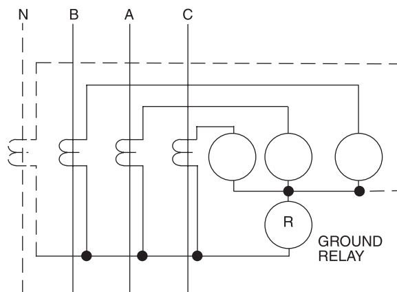
Figure 8-8—Residually connected ground relay
