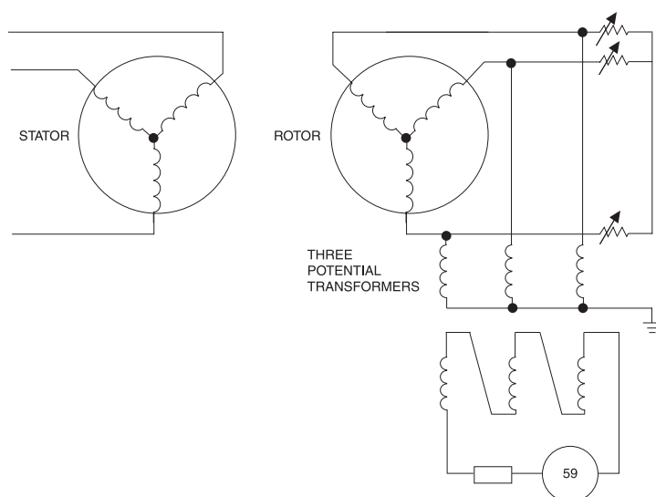
Figure 10-19—Rotor ground protection of wound-rotor motor
