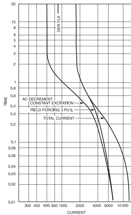
Figure 12-9—Generator decrement curve for a 19 000 kVA generator
