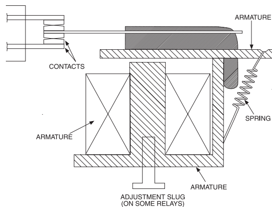
Figure 4-20—Clapper (or hinged-armature) instantaneous relay
