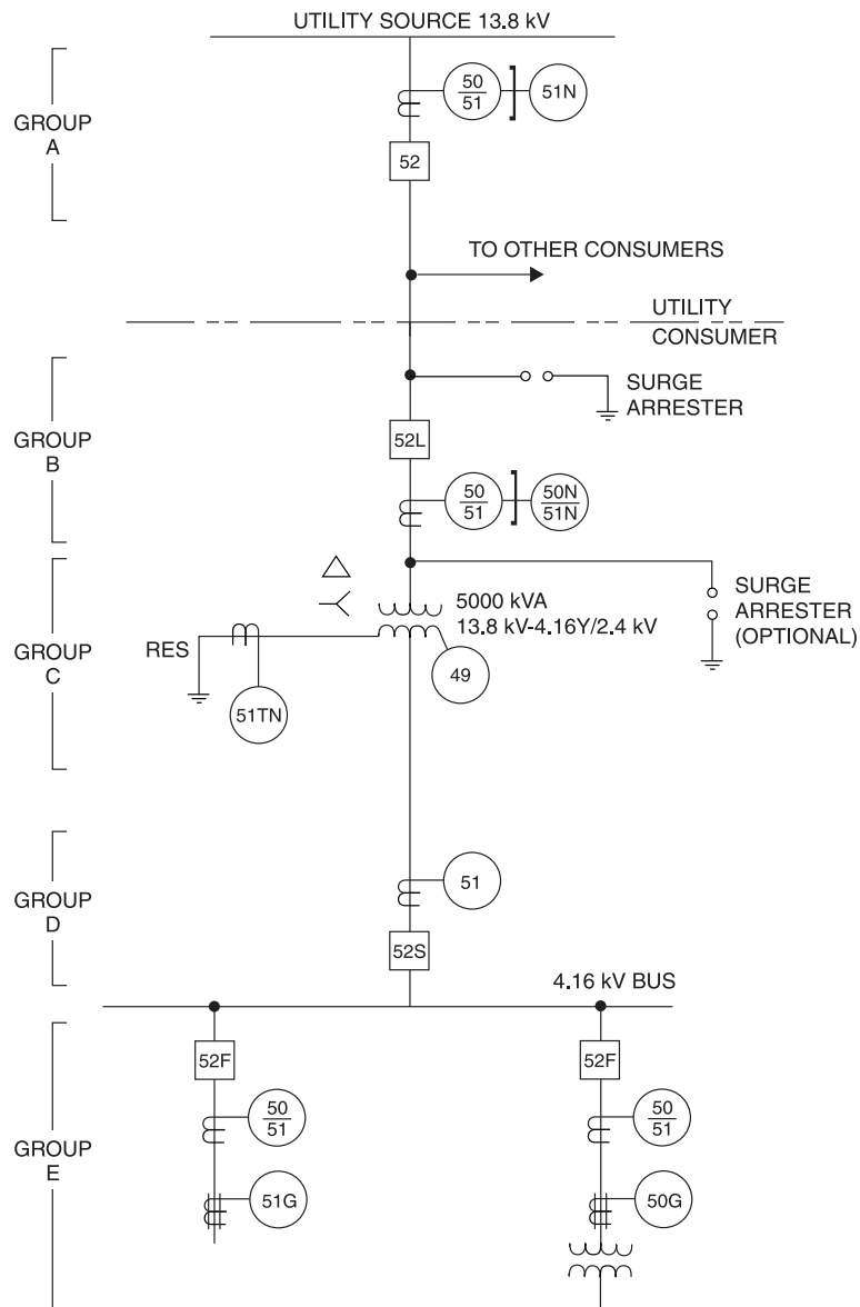
Figure 14-7—Single-service supply with transformer primary circuit breaker
