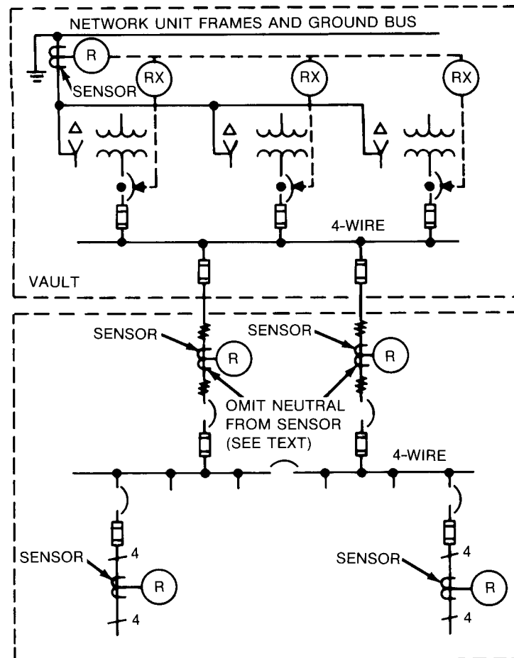
Figure 8-30—Ground-fault protection for spot network when user switchgear is secondary selective
