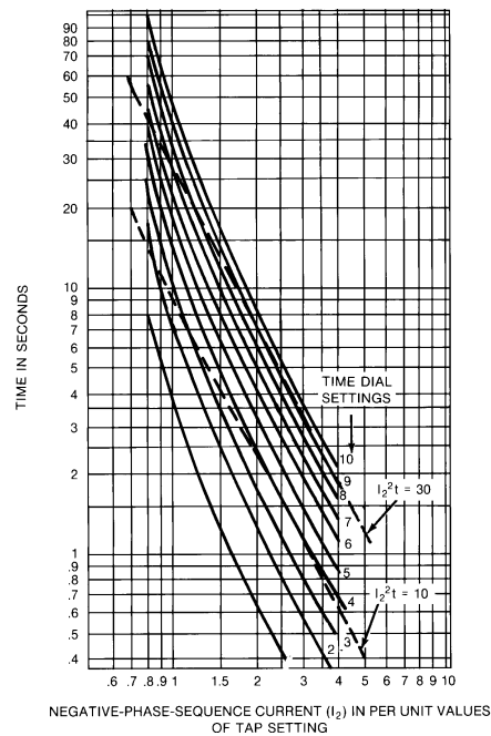
Figure 12-28—Characteristics of electromechanical negative-sequence overcurrent relay showing generator I_2^2 t limits
