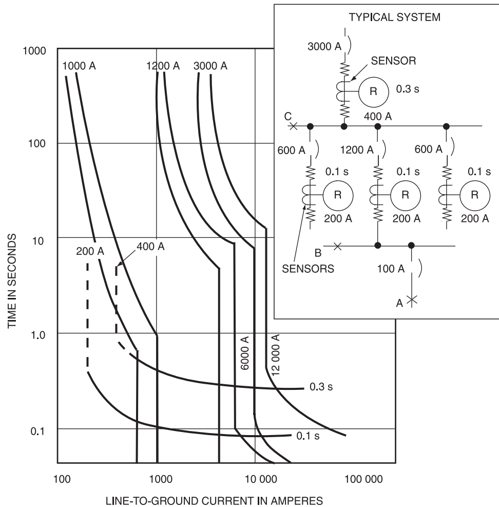
Figure 8-13—Ground relays on both main and feeder circuits
