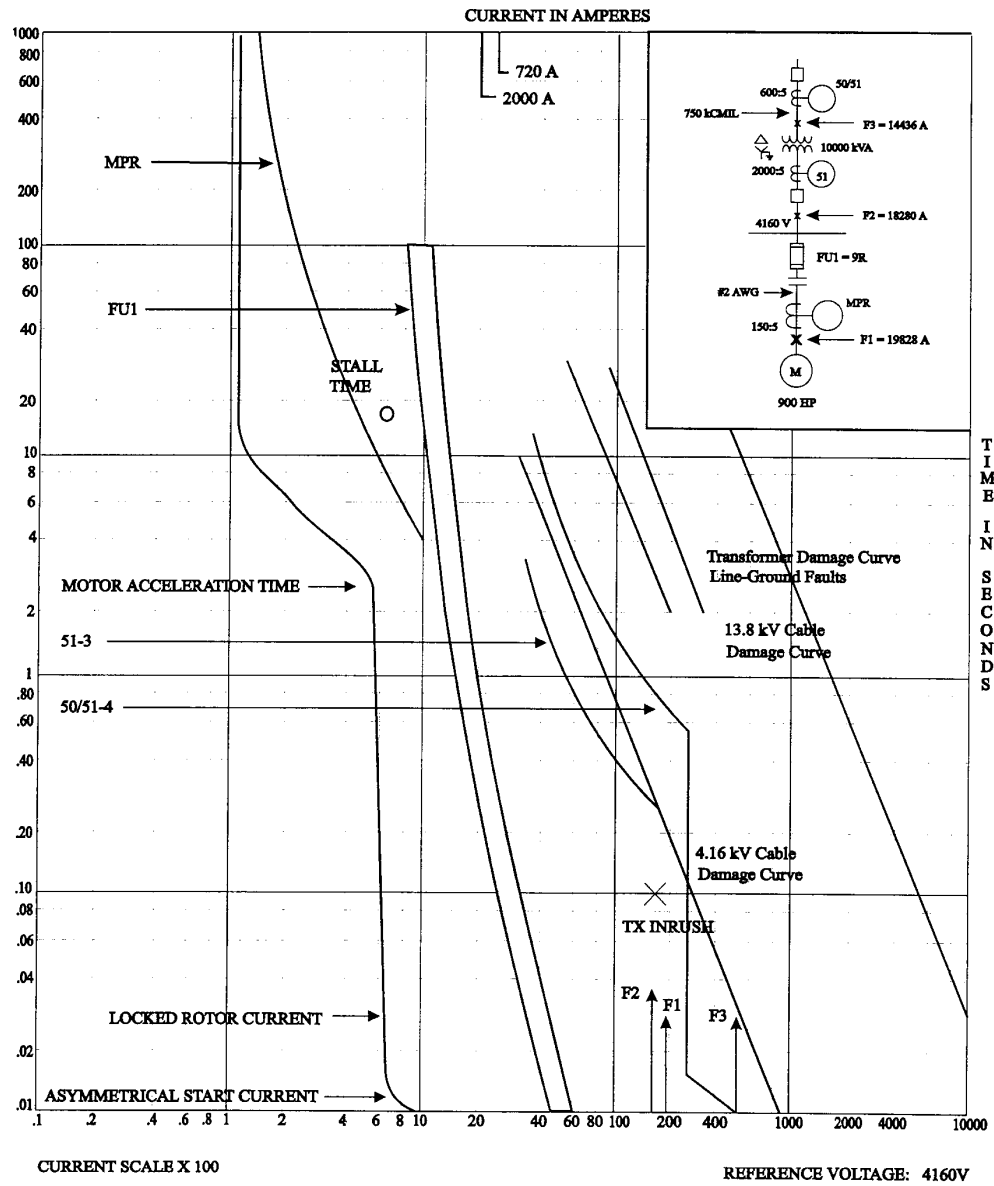
Figure 15-20—10 000 kVA transformer primary relay coordination plot
