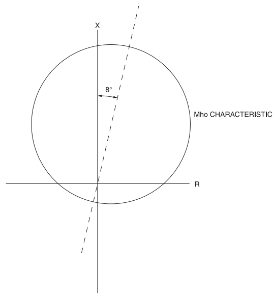
Figure 4-12—Var relay operating characteristic converted to the impedance plane
