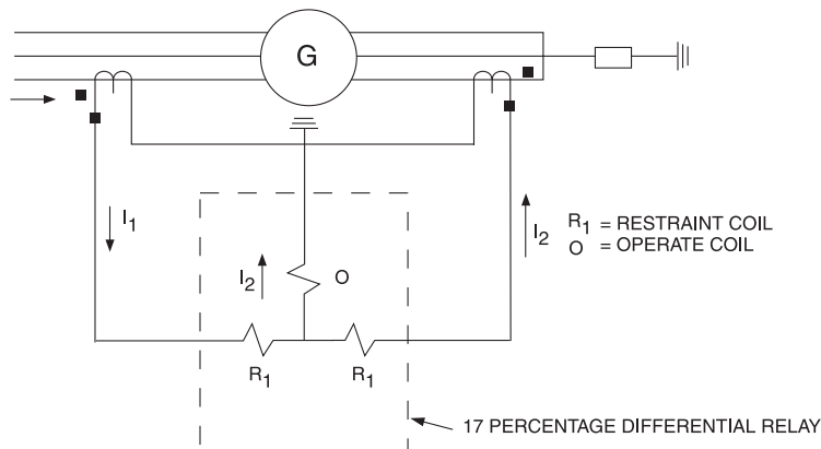
Figure 4-30—Basic relay connections (one phase) for fixed percentage restraint differential relay
