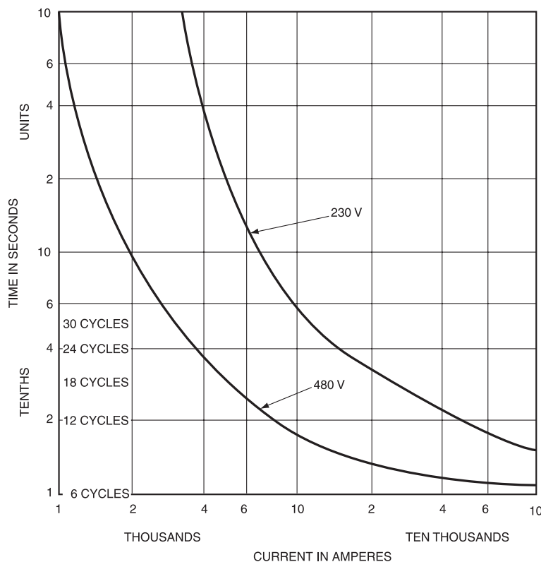
Figure 9-22—TCC for a power arc to burn a 6-mm-x-51-mm copper bar halfway
