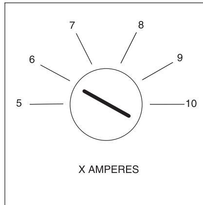
Figure 7-4—Instantaneous (magnetic) current adjustment provided on thermal-magnetic circuit breakers
