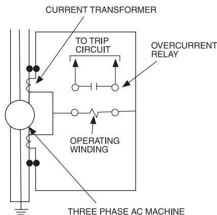
Figure 4-28a—Overcurrent relay used for differential protection, one phase shown
