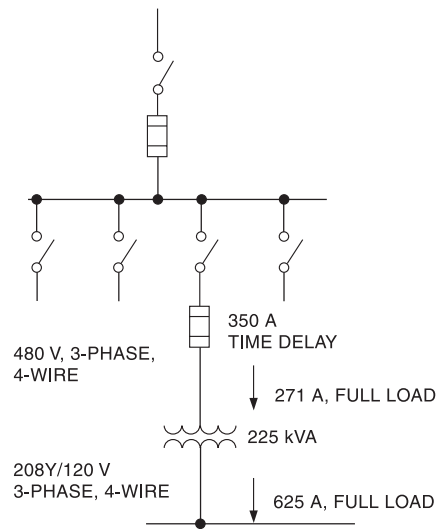
Figure 5-23—Application of time-delay fuses for transformer protection
