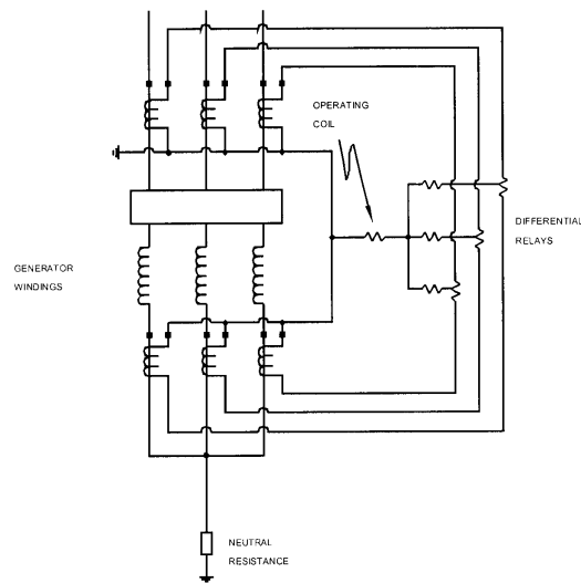
Figure 12-20—Generator ground differential protection using overcurrent relays
