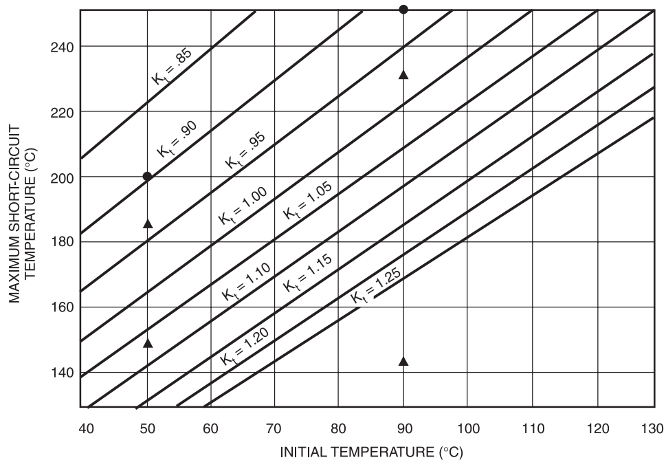
Figure 9-4—Correction factors K_t for initial and maximum short-circuit temperatures
