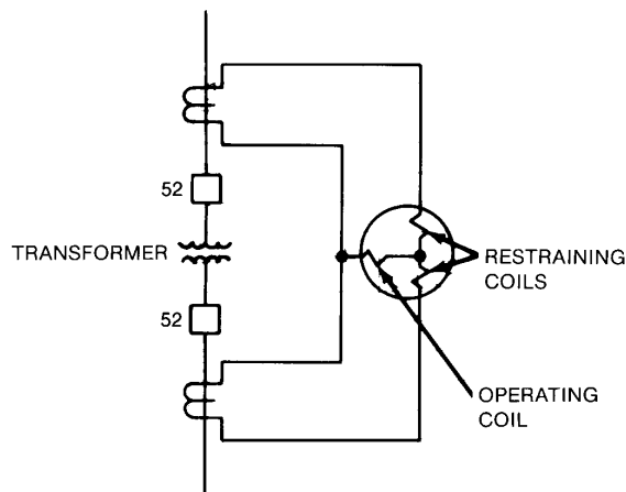
Figure 11-25—Percentage differential relays, which provide increased sensitivity while minimizing false operation as a result of CT mismatch errors for heavy through faults
