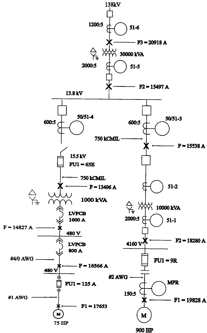
Figure 15-13—One-line diagram for coordination study
