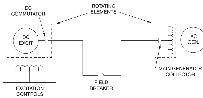
Figure 12-4—System with dc generator-commutator exciter
