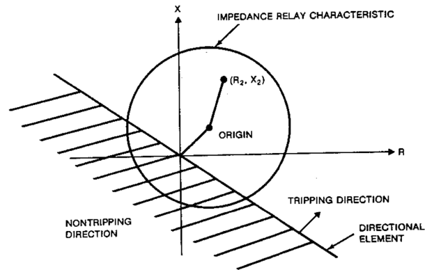
Figure 4-5—R-X diagram for a directional impedance relay
