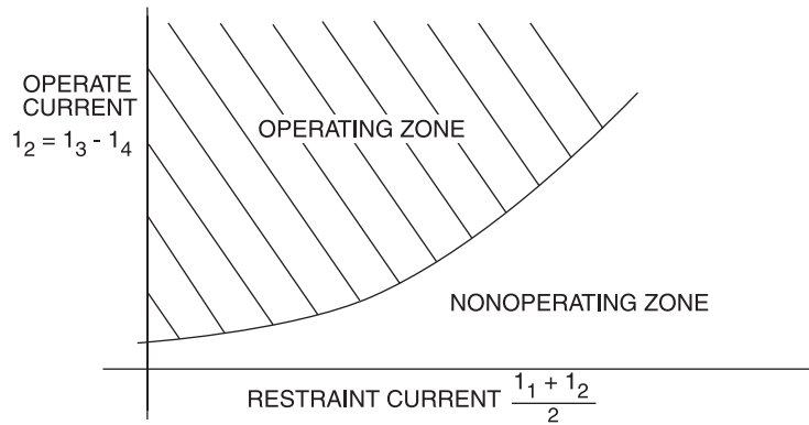
Figure 4-31a—Typical operating characteristic of a fixed percentage restraint differential relay
