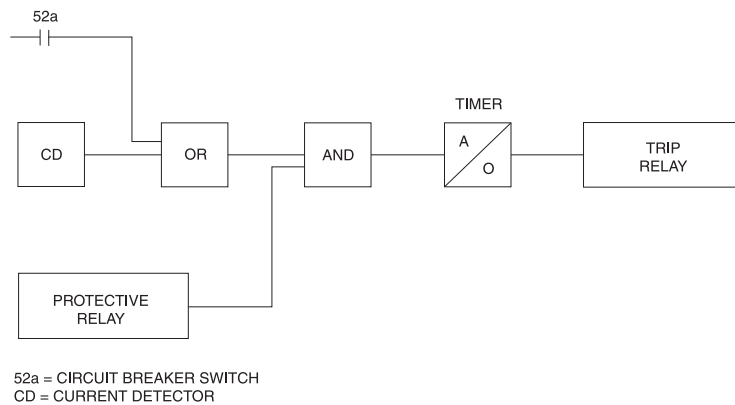
Figure 12-34— Functional diagram of a generator zone breaker failure scheme
