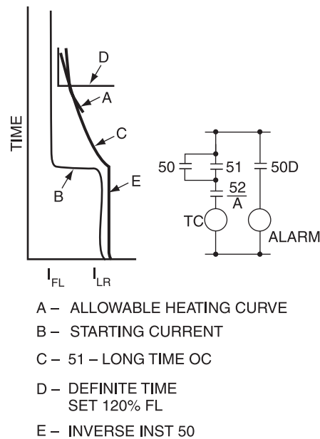
Figure 10-7—Alternative method of protecting a high-inertia motor
