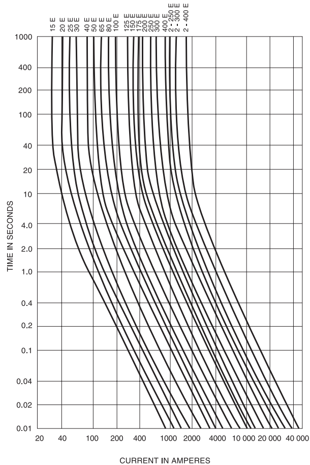
Figure 6-9—Typical minimum-melting TCC curves for medium and high-voltage solid-material power fuses
