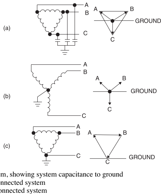
Figure 8-1 — Voltages to ground under steady-state conditions
