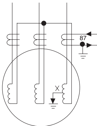
Figure 10-11—Self-balancing differential protection (one relay shown)
