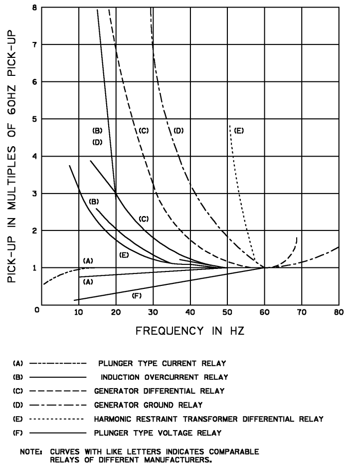
Figure 12-36—Relay pickup versus frequency
