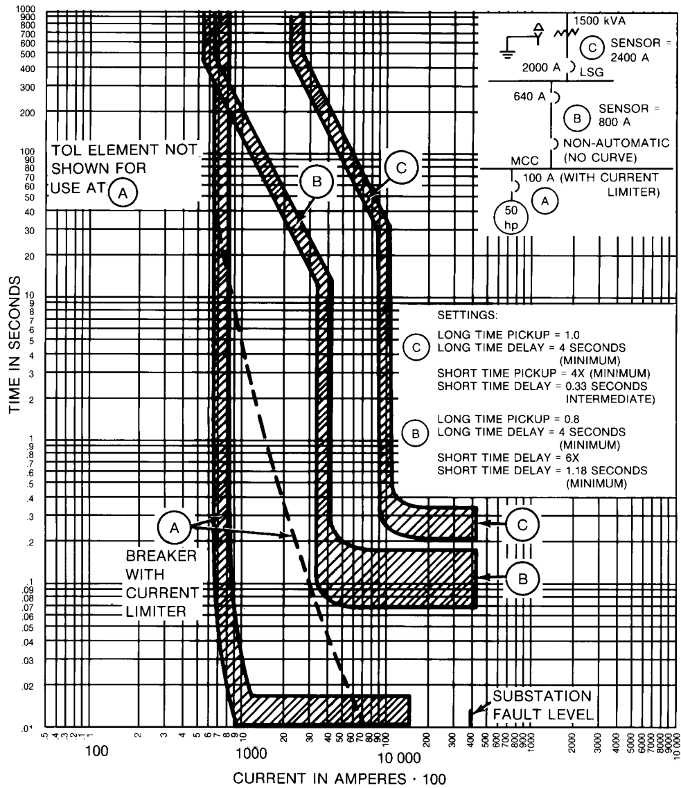
Figure 15-30—Phase TCC curves Example 3
