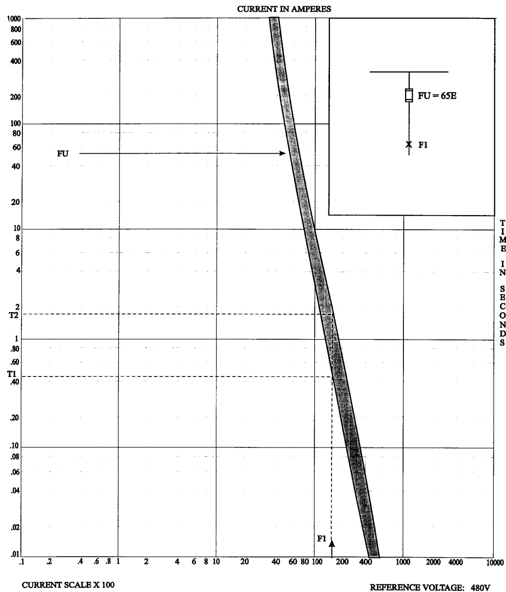
Figure 15-5b—Overcurrent trip time characteristic for a given fault for a fuse
