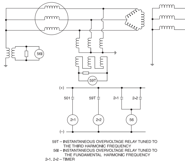
Figure 12-18—Third-harmonic overvoltage scheme for generator ground-fault protection
