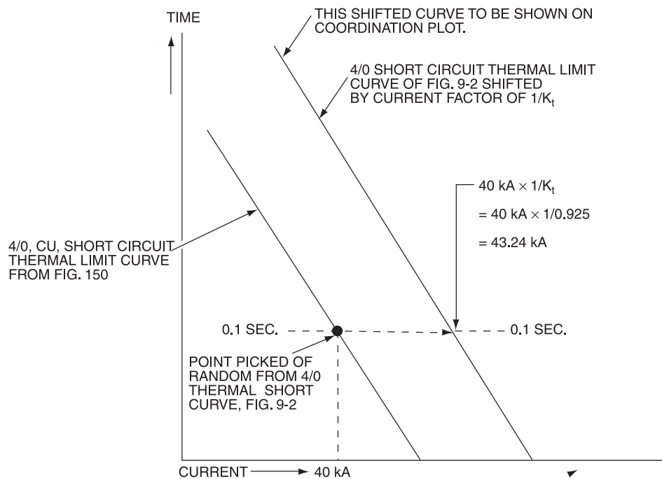
Figure 9-13—Shifting of thermal limit curve for use with coordination plot of Example 1
