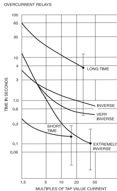
Figure 4-18—Comparison of typical curve shapes for overcurrent relays
