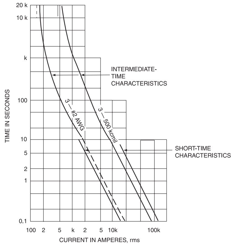
Figure 9-17b—Ratings of small and large cable in conduit in air, intermediate and short-time, EPR and XLP
