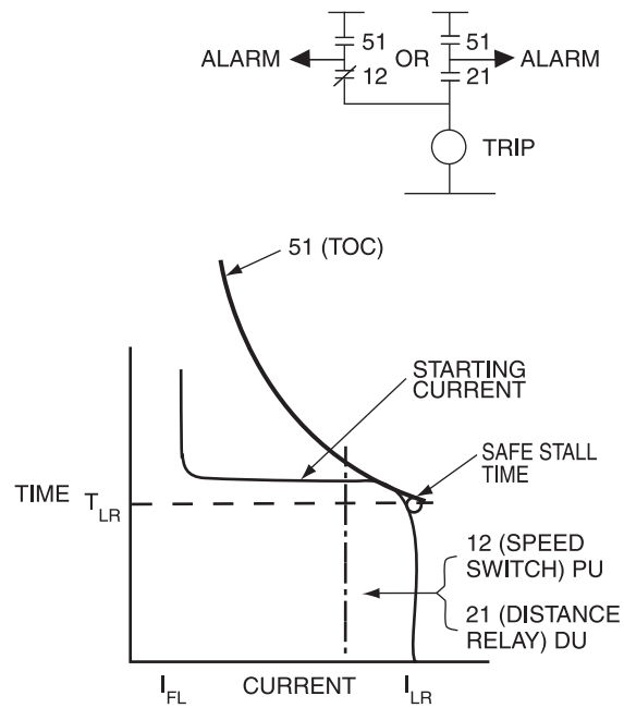
Figure 10-9—Schematic of locked-rotor protection of Figure 10-8
