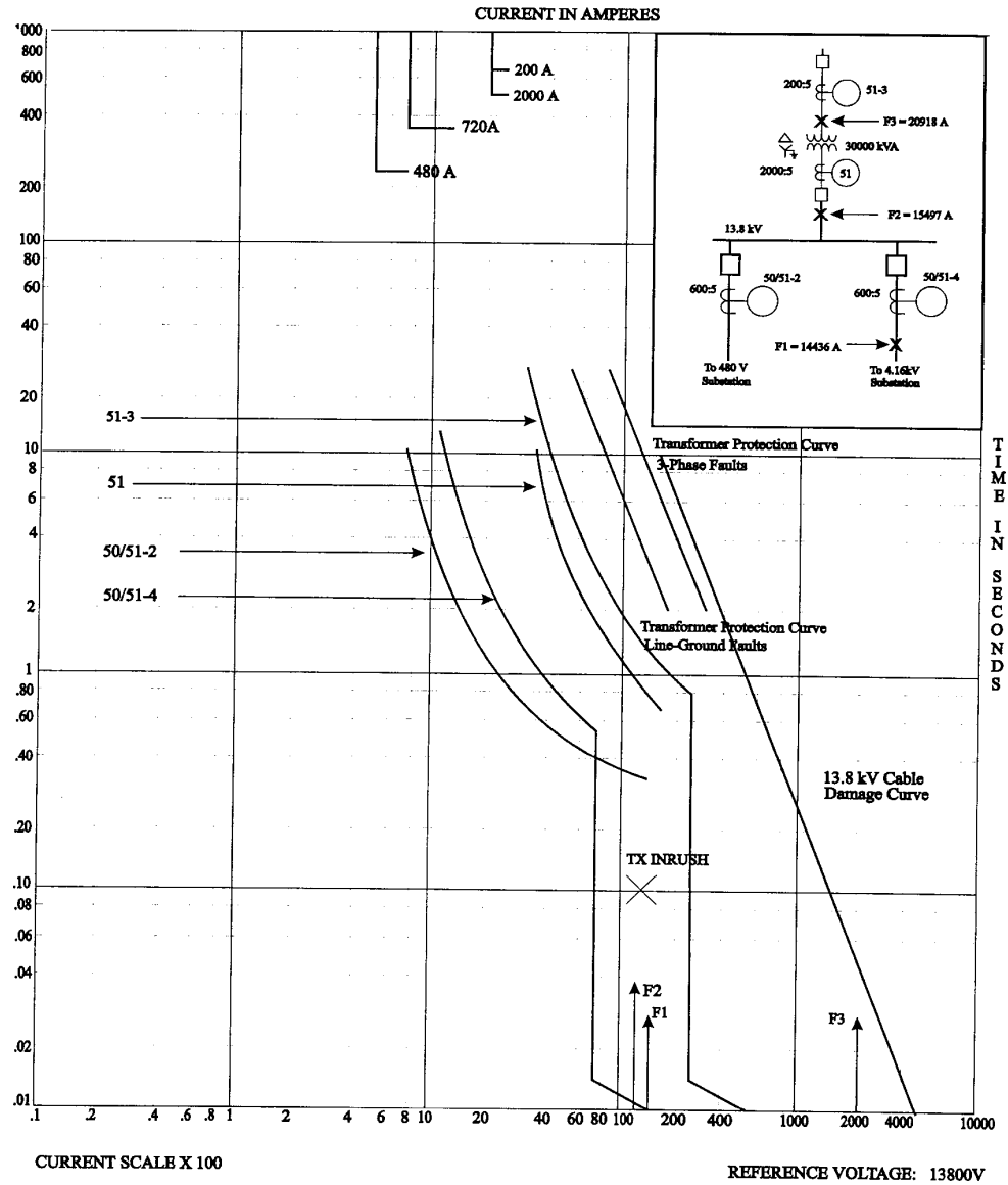
Figure 15-23—30 000 kVA transformer primary relay coordination plot
