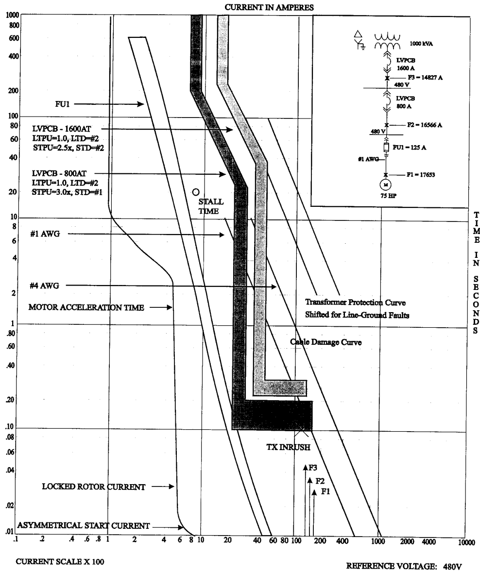
Figure 15-16—1000 kVA transformer secondary main coordination plot
