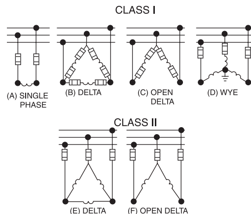
Figure 6-12—Various methods of connecting VTs to bus, showing fuse positions
