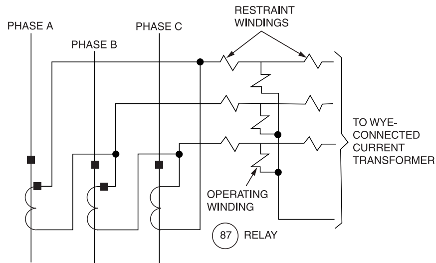
Figure 3-9—Delta-connected CTs
