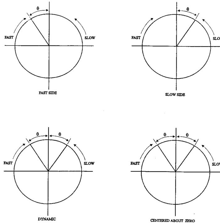
Figure 4-6c—Application of synchronizing relay dynamic characteristic
