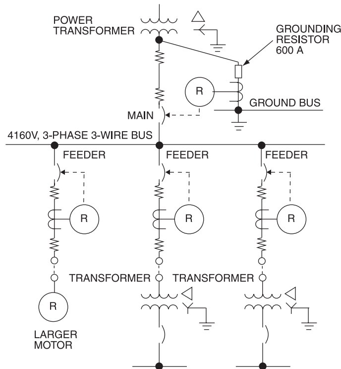
Figure 8-21 — Three-wire low-resistance-grounded system
