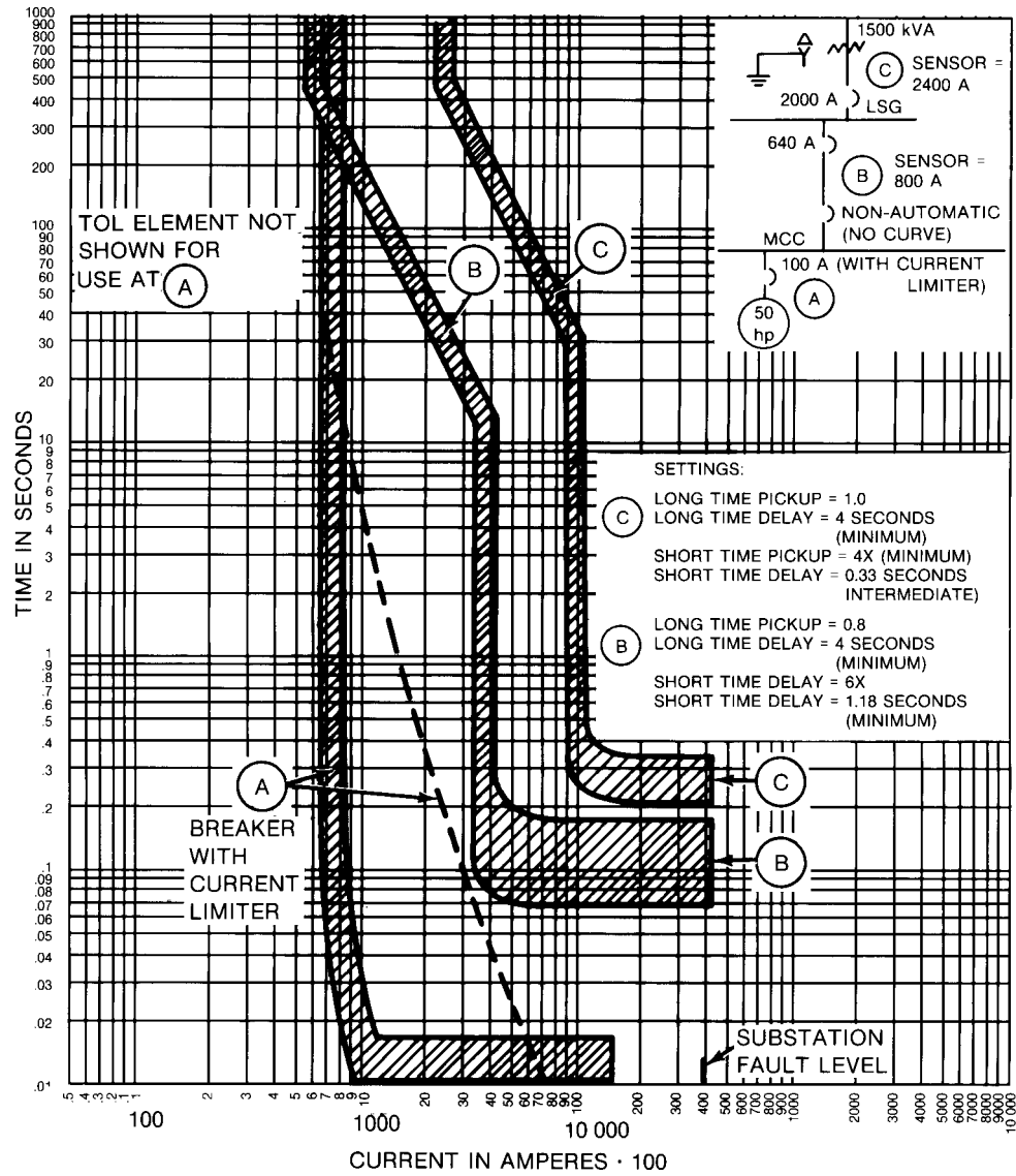
Figure 15-29—Phase-fault TCC curves Example 2
