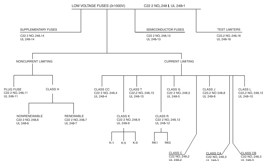
Figure 5-3—Low-voltage fuses covered by UL and CSA
