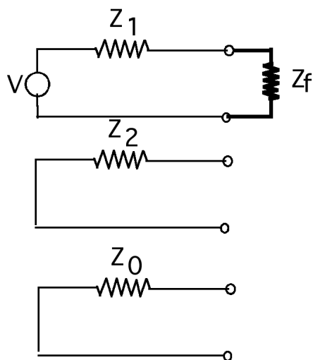
Figure 2-9—Sequence interconnections for a balanced three-phase fault, which involve only positive-sequence quantities
