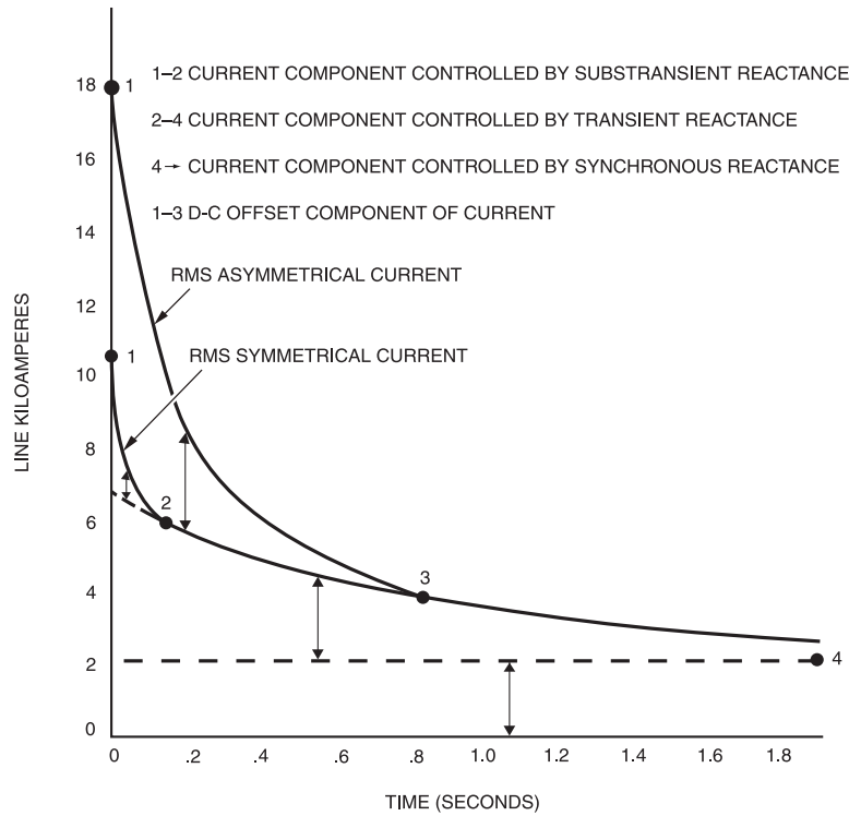
Figure 12-8—Typical generator decrement curve
