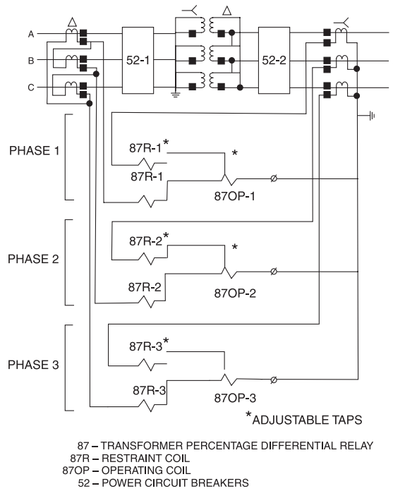
Figure 4-29—Basic relay connections (one phase) for fixed percentage restraint differential relay
