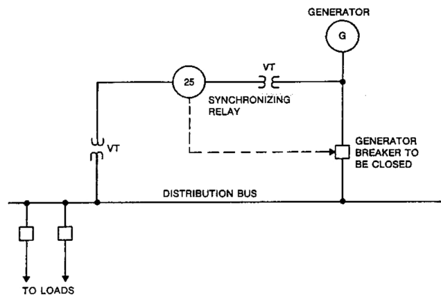
Figure 4-6b—Application of synchronizing relay to connect a generator onto a system bus
