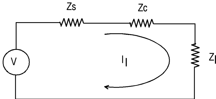
Figure 2-1—Equivalent circuit used to calculate load current in a normal circuit
