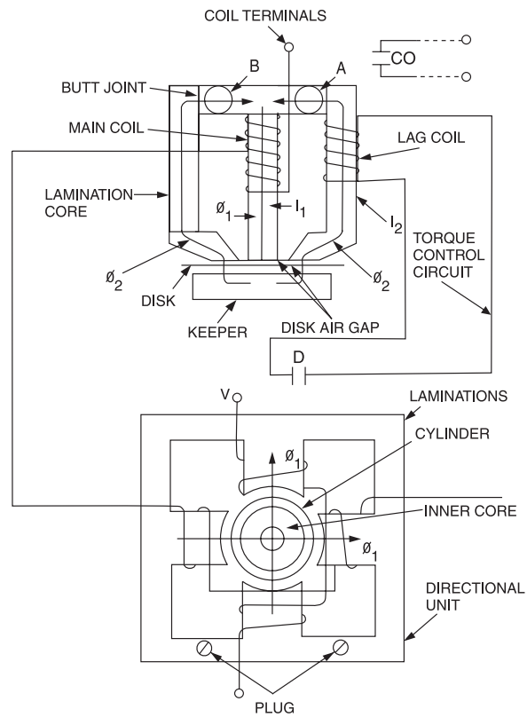
Figure 4-23—Directionally controlled overcurrent relay
