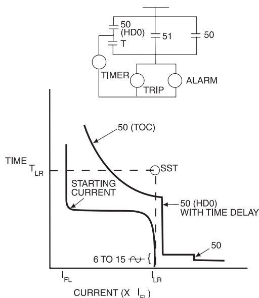
Figure 10-6—Protection of high-inertia motor
