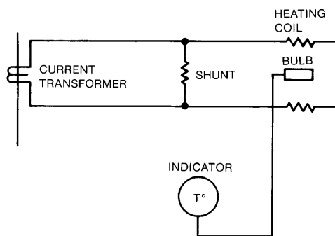
Figure 11-15—Thermal (or winding temperature) relay, which uses a heating element to duplicate effects of current in transformer
