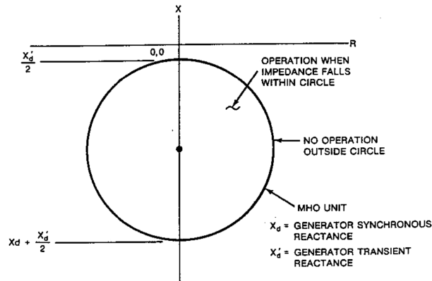
Figure 4-4b—R-X diagram for the mho-supervised reactance relay
