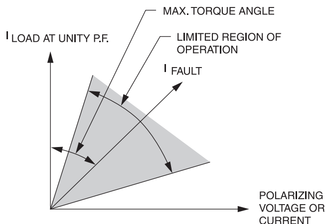
Figure 4-26—Region of operation characteristic for a static direction overcurrent relay
