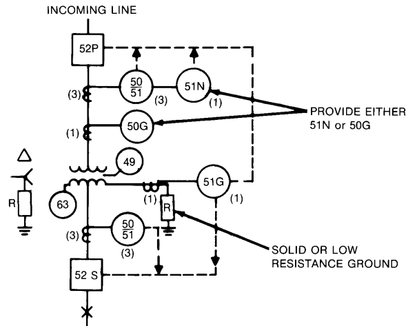
Figure 11-18—Overcurrent relays, frequently used to provide transformer protection in combination with primary circuit breaker or circuit switcher
