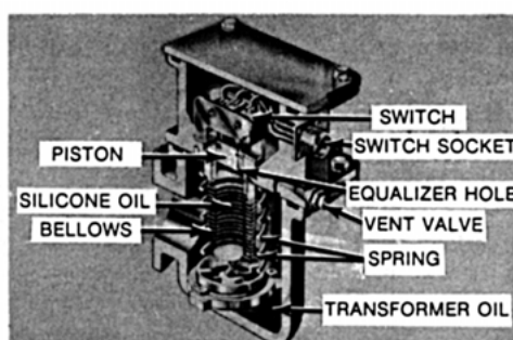
Figure 11-10—Sudden oil-pressure-rise relay mounted on transformer tank below normal oil level
