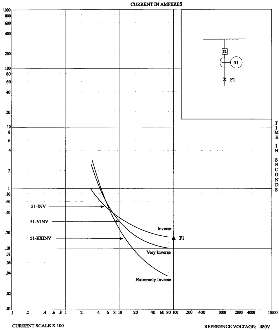
Figure 15-7—Relative shape and inversivity of typical relay time-current curves
