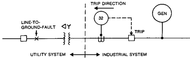
Figure 4-8—Application of directional power relay used to detect line-to-ground faults (Example 1)
