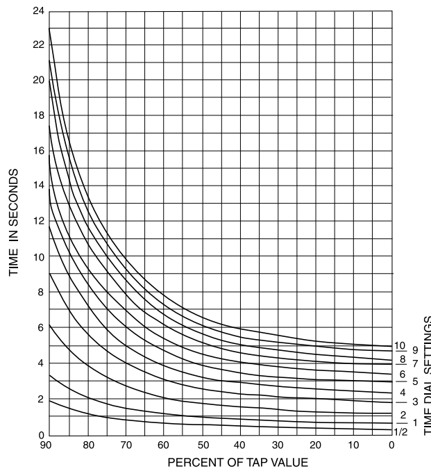
Figure 4-7—Typical time-voltage characteristic of an undervoltage relay
