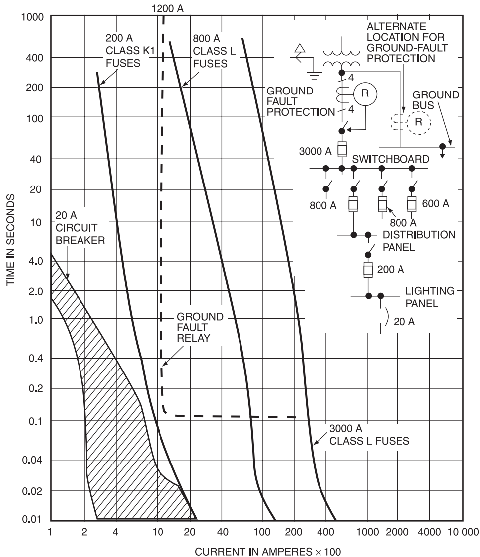
Figure 8-14—Fused system using ground-fault relays on main circuit only, showing coordination with 200 A fuses and lack of coordination with 800 A feeder fuses
