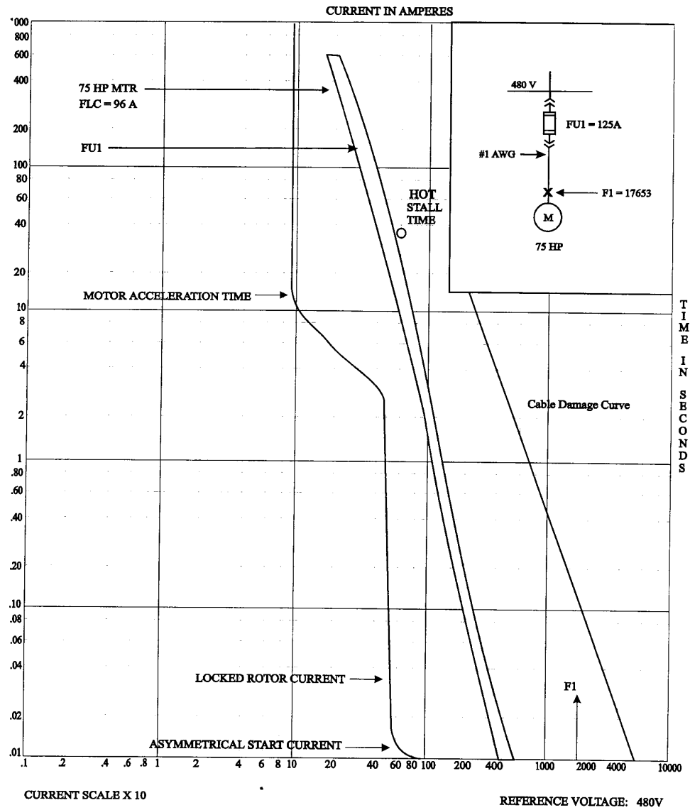
Figure 15-14—480 V fuse coordination plot
