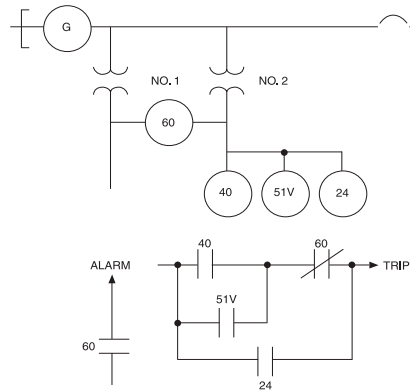
Figure 4-21—Typical application of voltage balance relay
