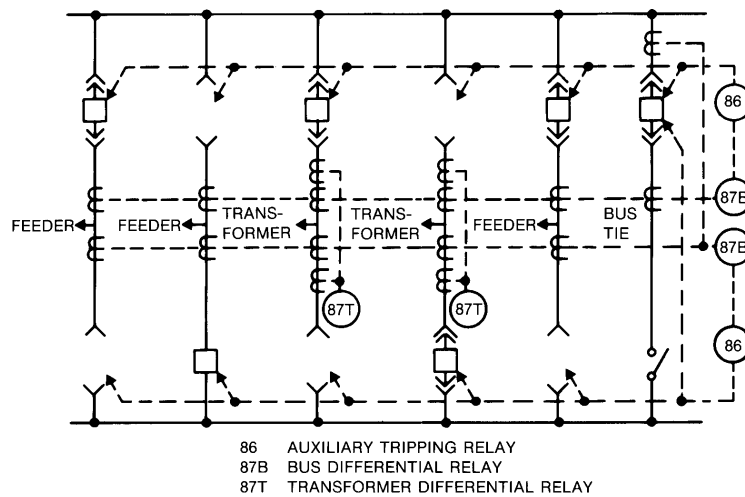
Figure 13-3—Double-bus scheme with bus differential relay
