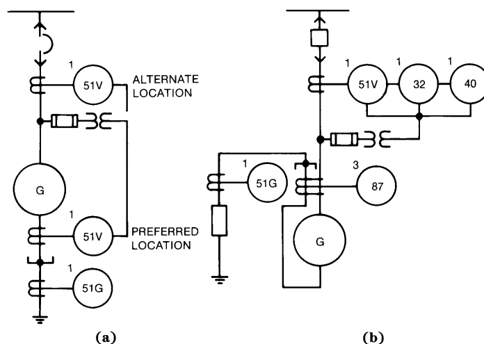
a) Single-isolated generator on low-voltage system b) Multiple-isolated generator on medium-voltage system
