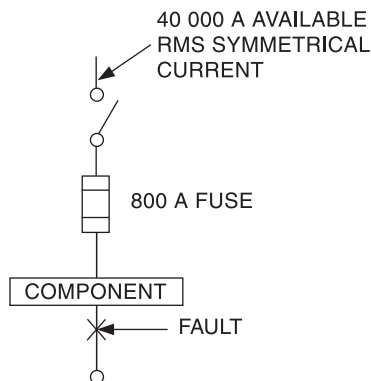
Figure 5-18—Example for applying fuse let-through charts
