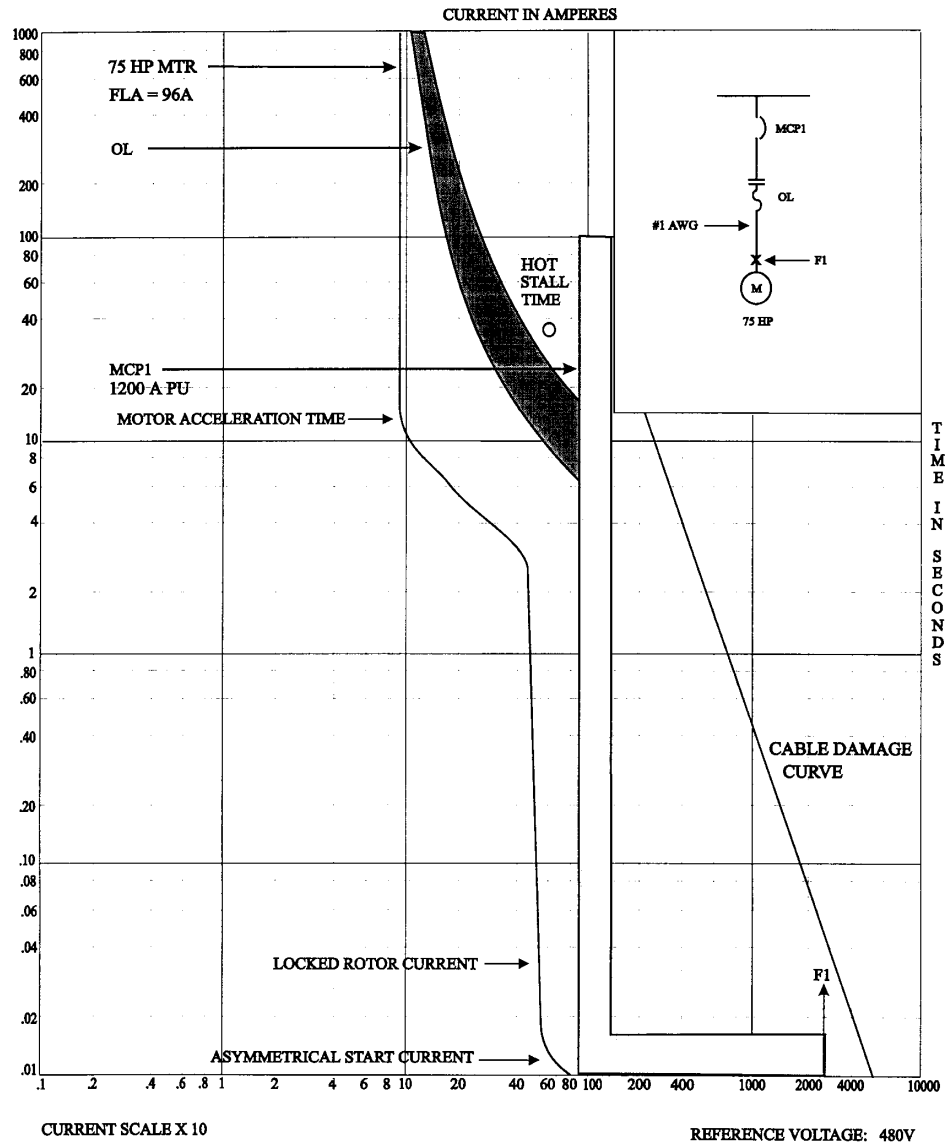
Figure 15-3b—Motor overload coordination plot using combination overload relay and magnetic-only MCCB
