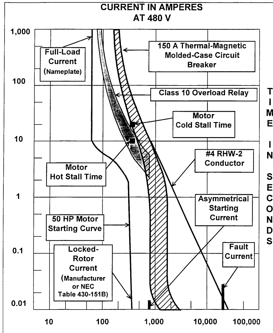
Figure 15-3c—Motor overload coordination plot using combination overload relay and thermal-magnetic MCCB
