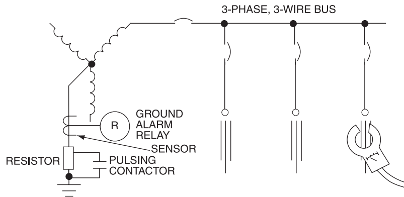
Figure 8-26—High-resistance-grounded system with pulsing contactor to locate faulted feeder
