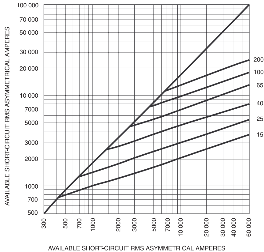
Figure 6-1 — Peak let-through currents for medium-voltage current-limiting fuses
