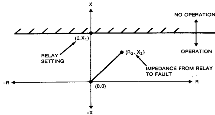
Figure 4-1—R-X diagram for the generic reactance relay
