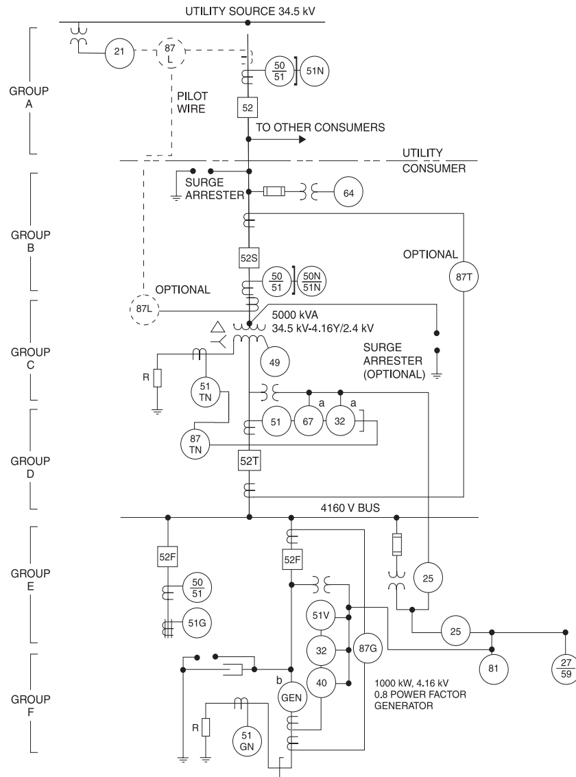
Figure 14-10—Single service with in-plant generation
