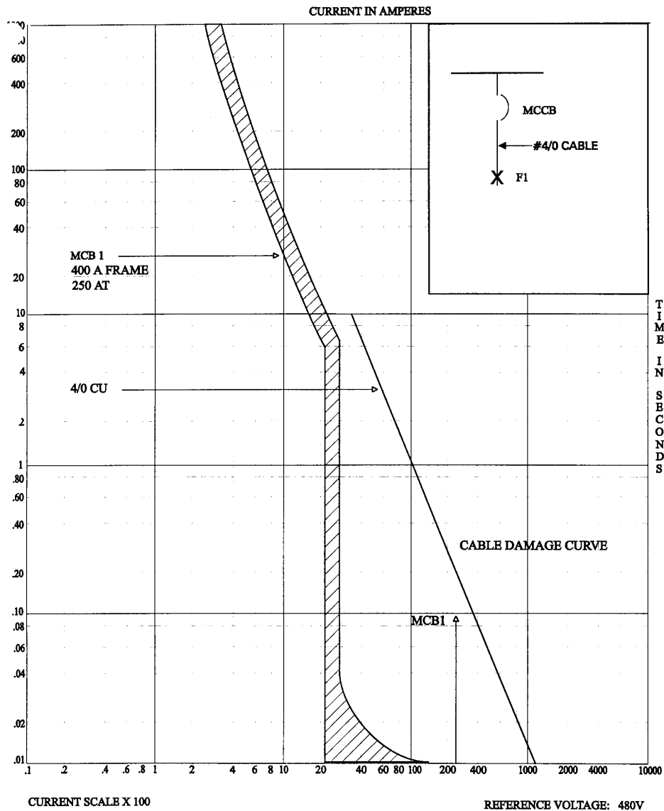
Figure 15-2—Basic criteria for conductor protection using an MCCB
