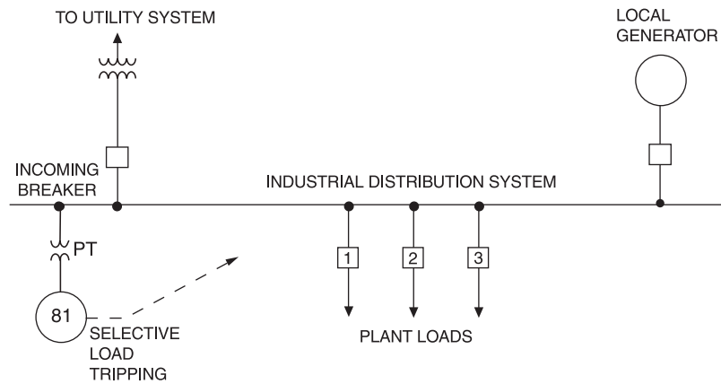
Figure 4-27b—Load-shedding scheme for loss of an external system
