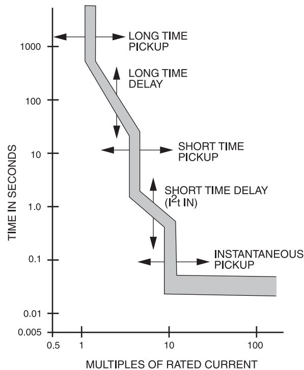
Figure 7-7b—Typical TCC curve for electronic trip circuit breaker ( I^2t IN); adjustable functions identified
