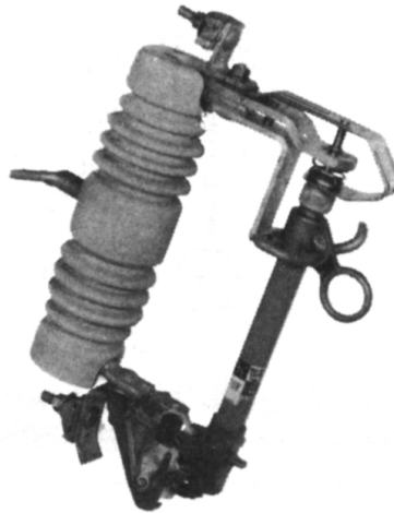
Figure 6-4—Open distribution fuse cutout, rated 100 A
