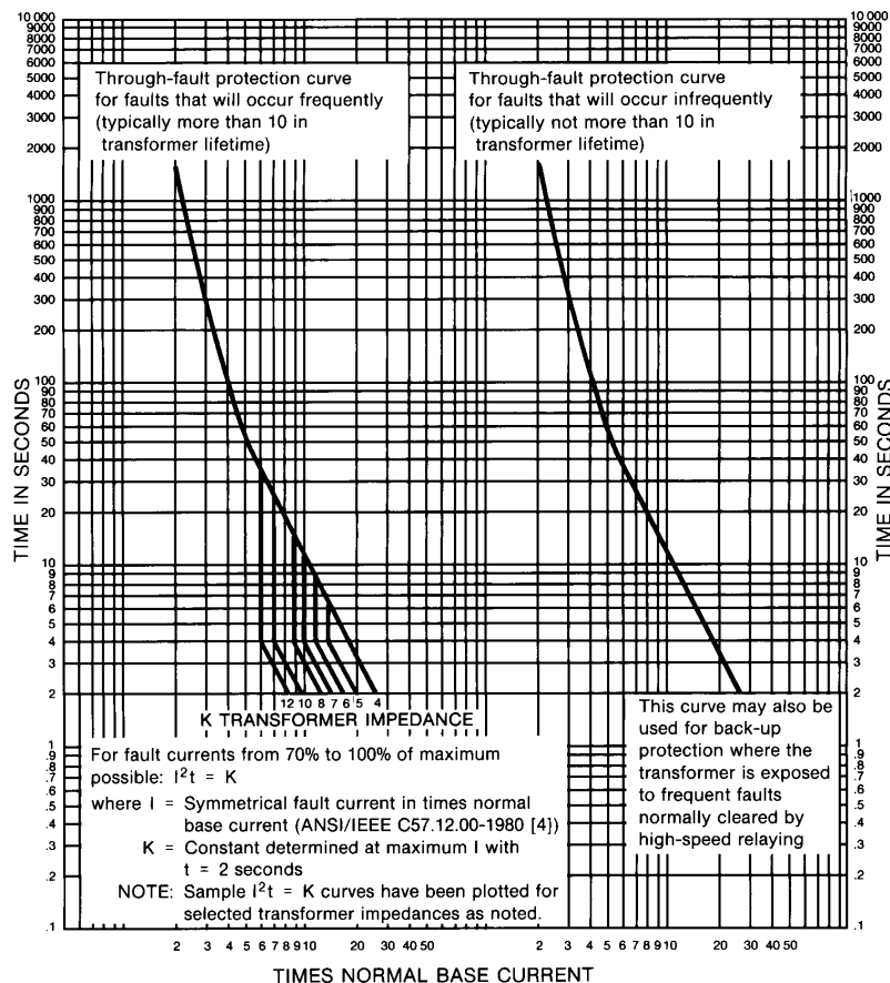
Figure 11-20—Through-fault protection curves for liquid-immersed Category II transformers (501–1667 kVA single-phase, 501–5000 kVA three-phase)
