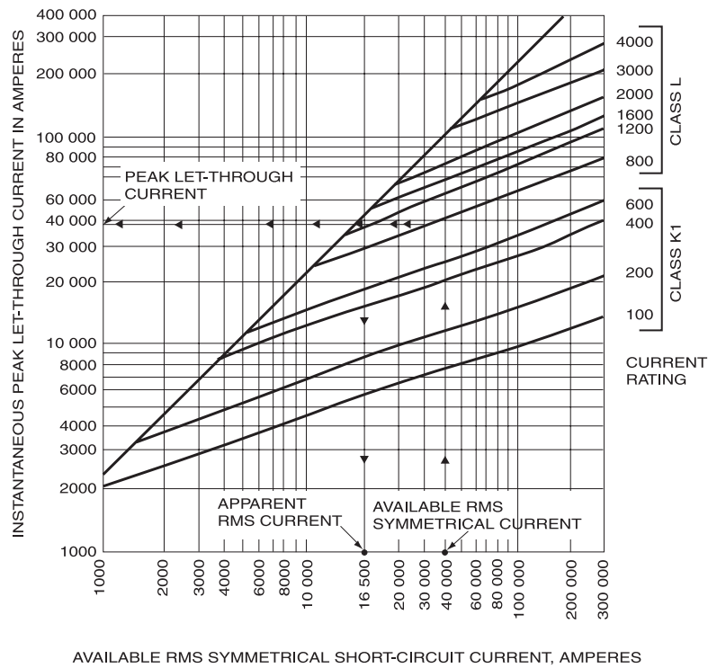
Figure 5-17—Typical 60 Hz peak let-through current as a function of available rms symmetrical current (15% power factor)
