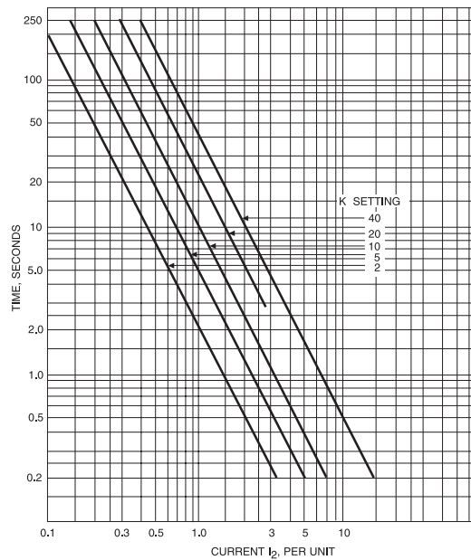
Figure 4-15—Typical n-s overcurrent relay operating characteristic
