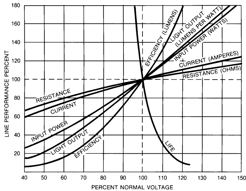
Figure 14-1—Incandescent lamp performance as affected by voltage
