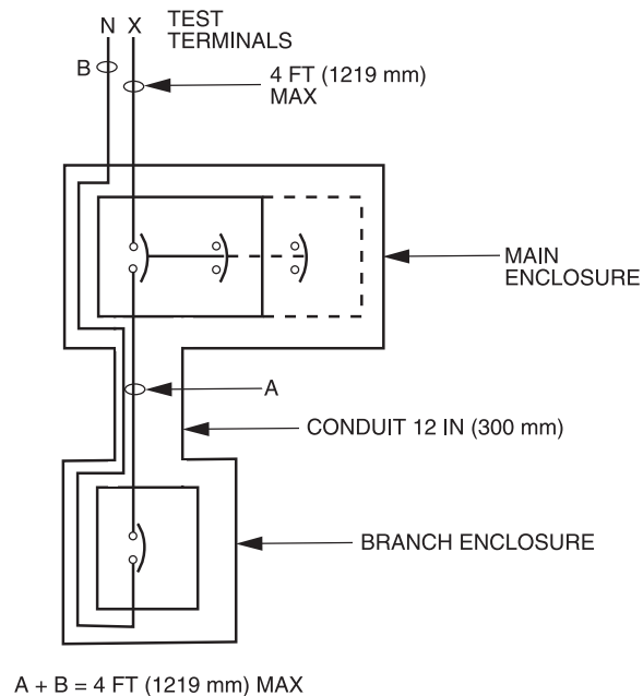
Figure 7-10—Series connection test circuit from UL 489-1996
