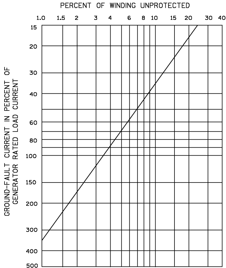
Figure 12-16—Percent of stator winding unprotected by differential relay for phase-to-ground fault
