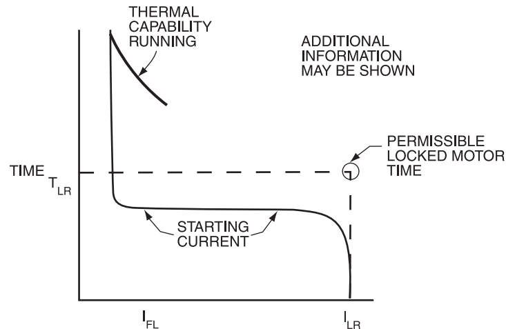
Figure 10-1—Typical motor-starting and capability curves (specific motor terminal voltage and for cold start)
