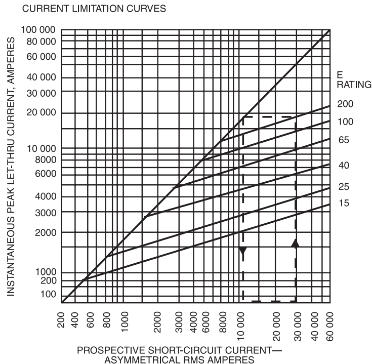
Figure 9-11—Current-limiting fuse let-through for use with Example 1
