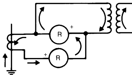
Figure 11-29—Relay current during transformer internal faults
