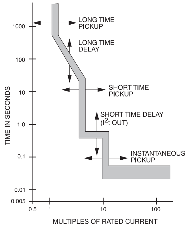
Figure 7-7a—Typical TCC curve for electronic trip circuit breaker ( I^2t \text{ OUT} ); adjustable functions identified
