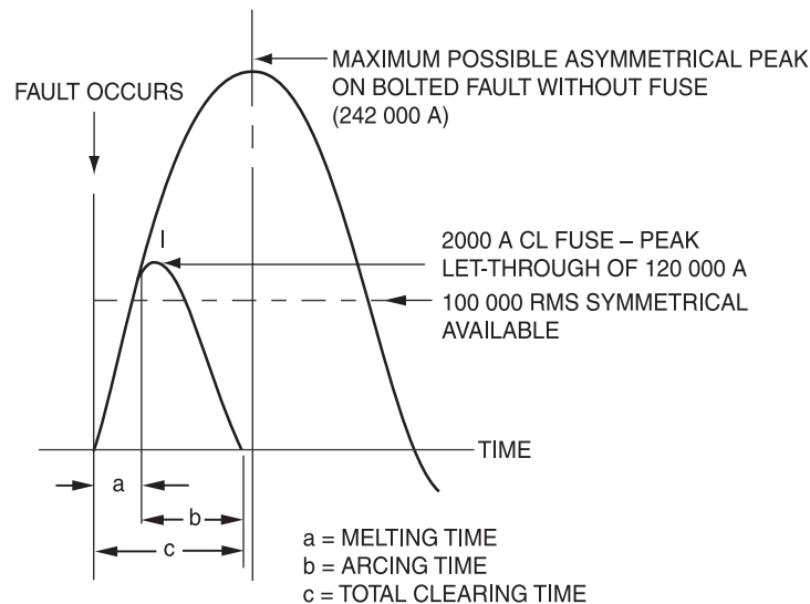
Figure 5-1—Typical current limitation showing peak let-through current and total clearing time
