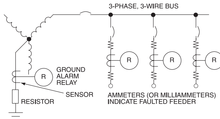
Figure 8-25—High-resistance-grounded system using core-balance CTs and fault-indicating ammeters
