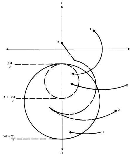
Figure 12-26—Loss-of-field impedance relay characteristics using offset mho distance relays
