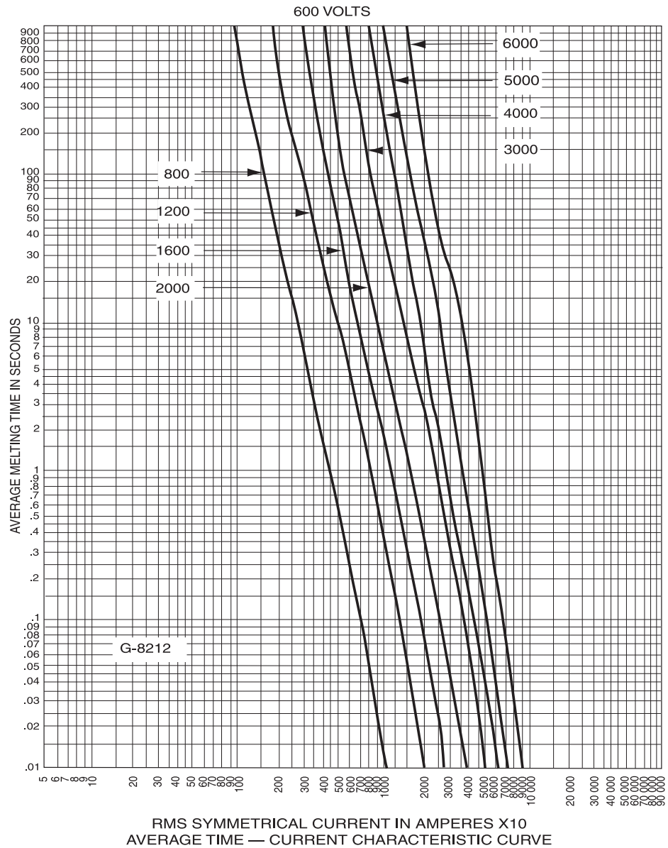
Figure 5-14—Current-limiting fuse, Class L
