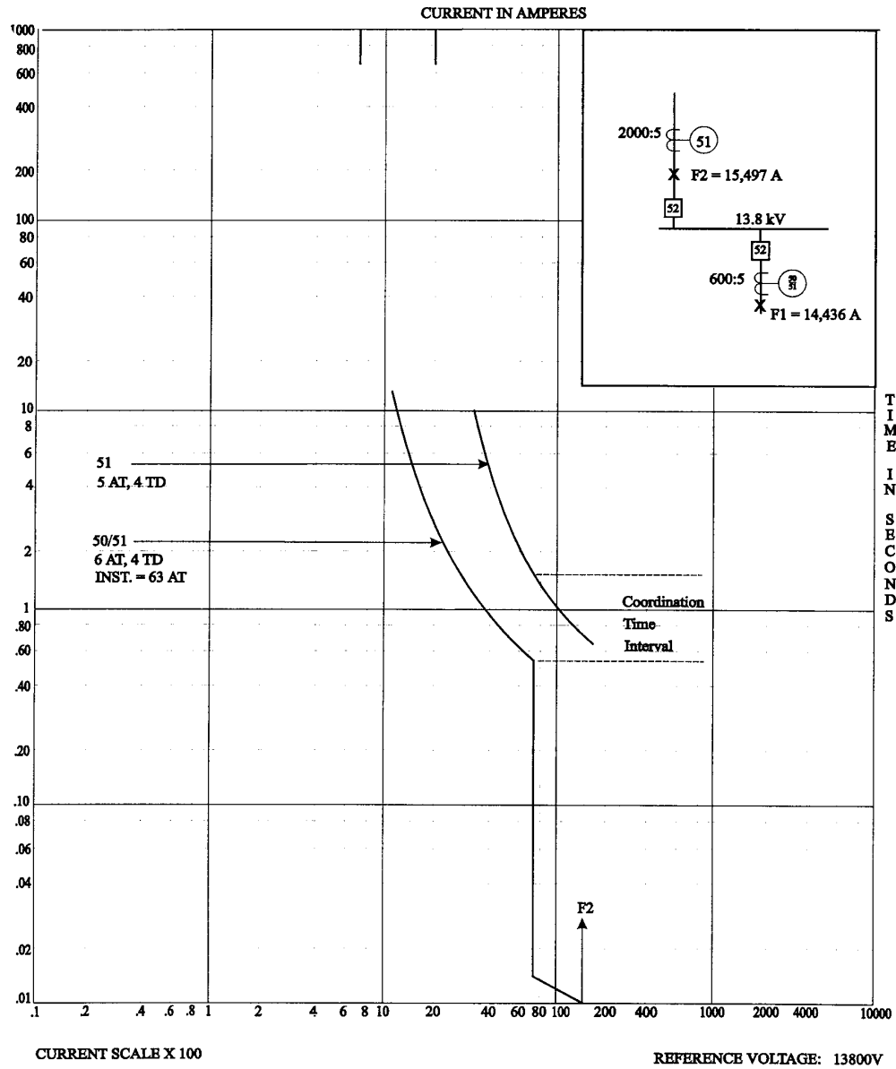
Figure 15-12—Example of CTI between two relays
