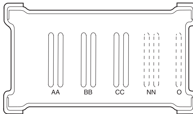
Figure 9-19—High-impedance busway where wide phase-to-phase spacings result in increased reactance
