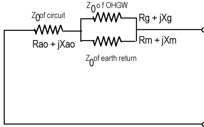
Figure 2-6b—Zero-sequence equivalent circuit that accounts for self impedance of transmission line and the impedances of earth and OHGW return paths
