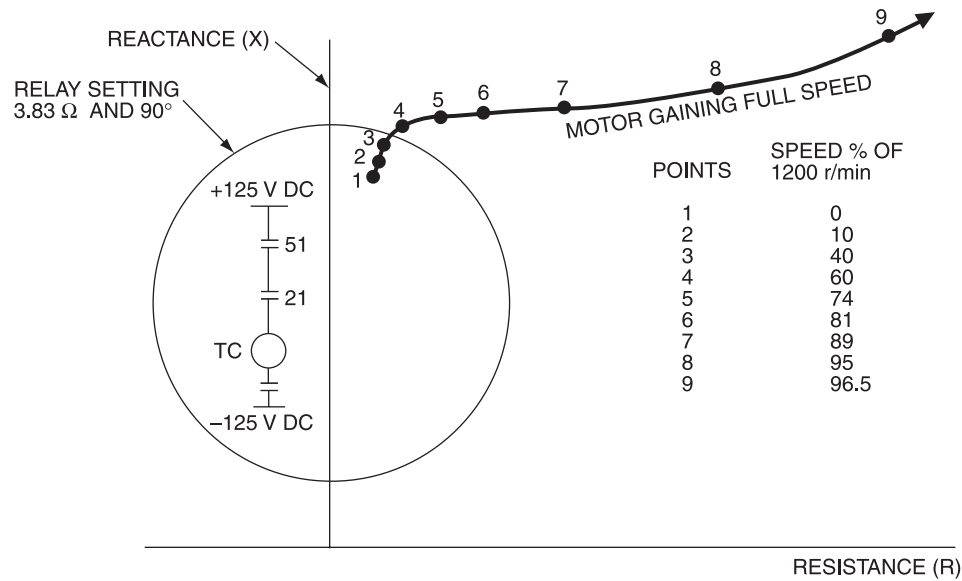
Figure 10-8—Protection of high-inertia motor using an impedance relay
