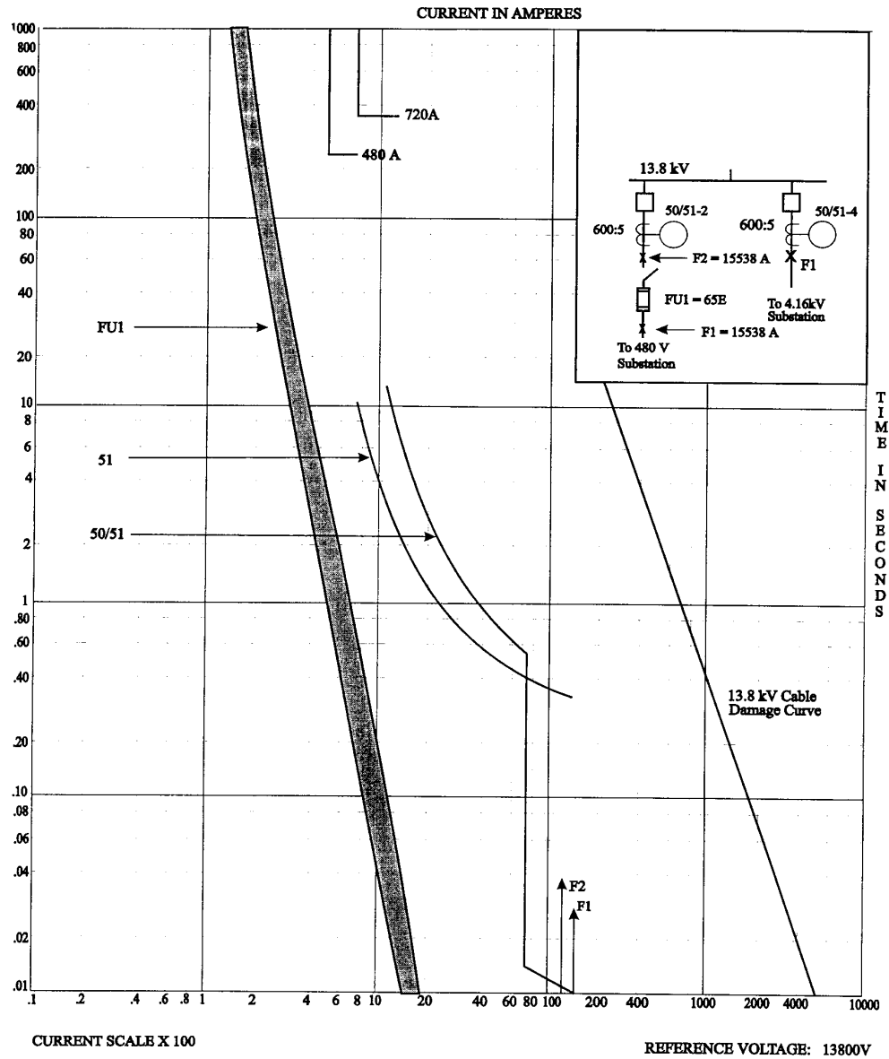
Figure 15-21—13.8 kV feeder relay coordination plot
