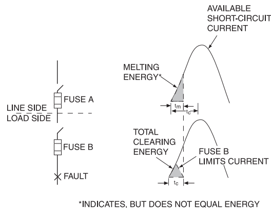
Figure 5-12—Selectivity of current-limiting fuses
