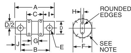
KNIFE-BLADE TYPE FUSES
