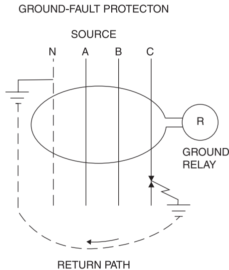
Figure 8-9a—Core-balance CT encircling all phase and neutral conductors
