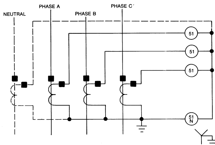
Figure 3-7—Wye-connected CTs
