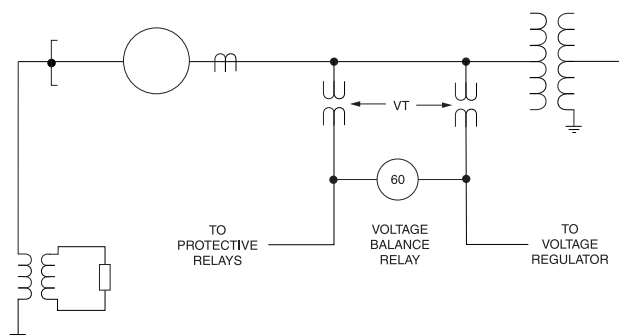
Figure 12-35—Application of voltage-balance relay
