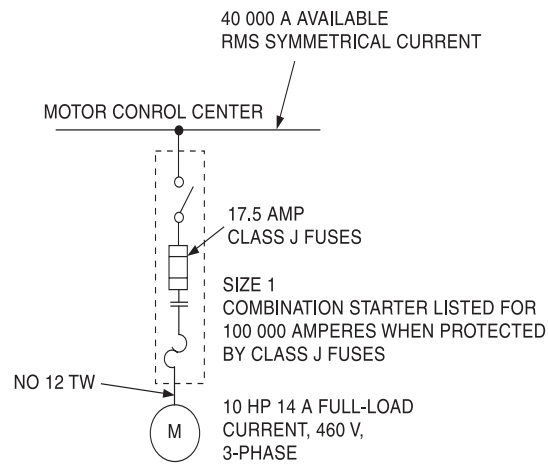
Figure 5-21—Application of fuses to provide short-circuit protection and backup protection for motor starters
