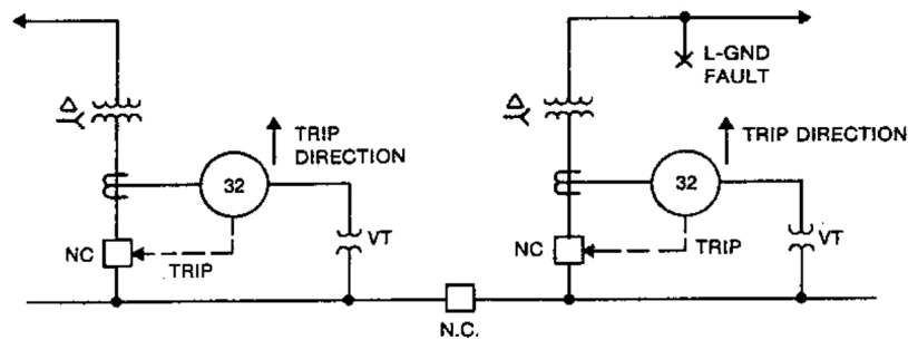
Figure 4-9—Application of directional power relay used to detect line-to-ground faults (Example 2)
