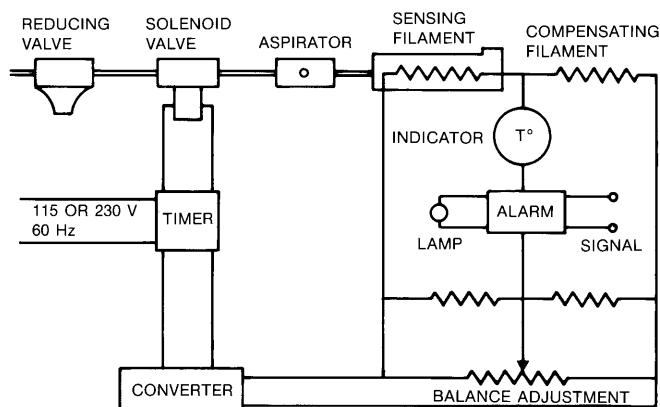
Figure 11-13—Combustible gas relay, which periodically samples gas in transformer to detect any minor internal fault before it can develop into a serious fault
