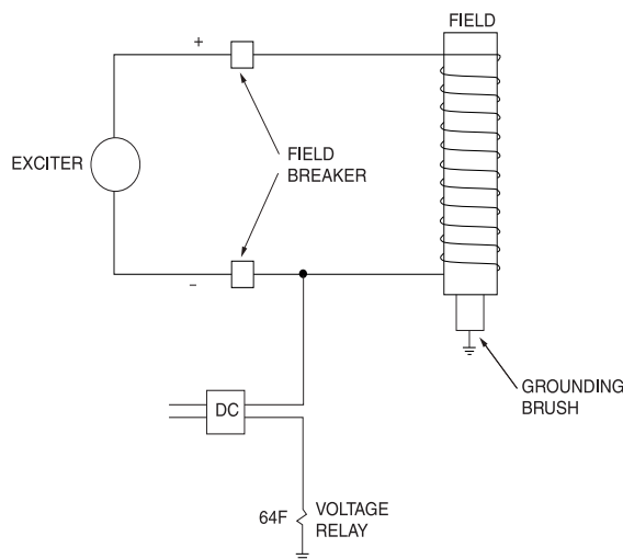
Figure 12-22—Field ground-fault protection using a dc source
