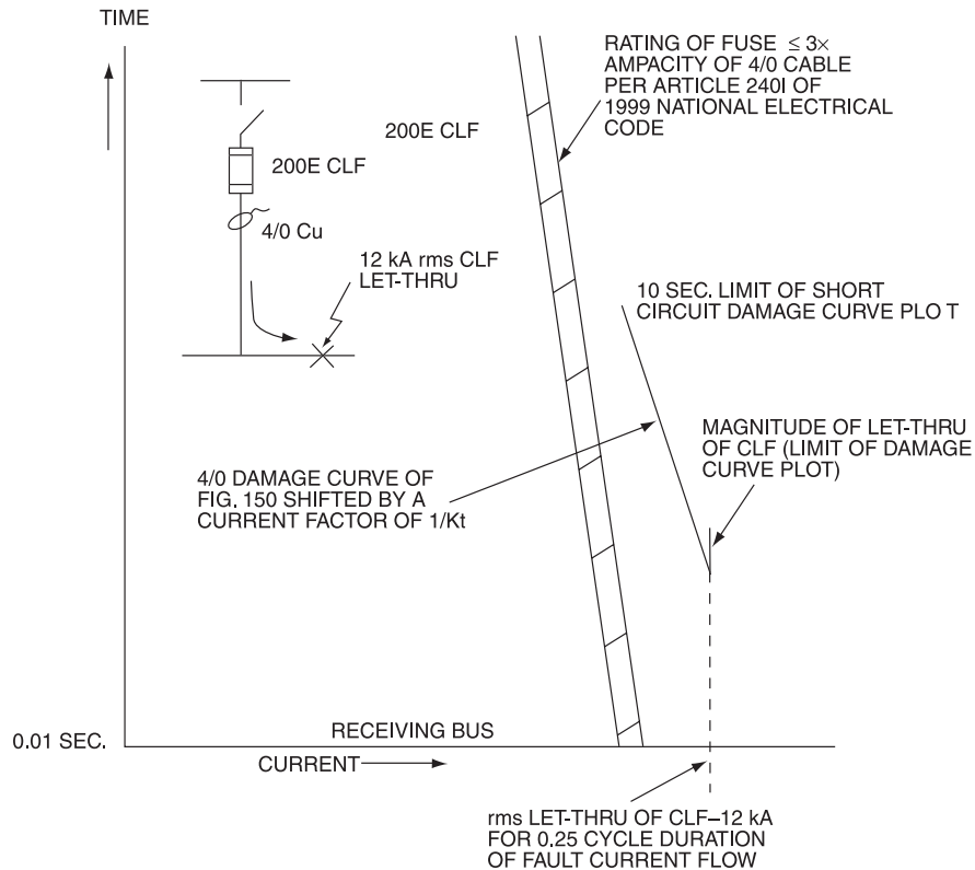
Figure 9-12—Short-circuit protection plot for Example 1
