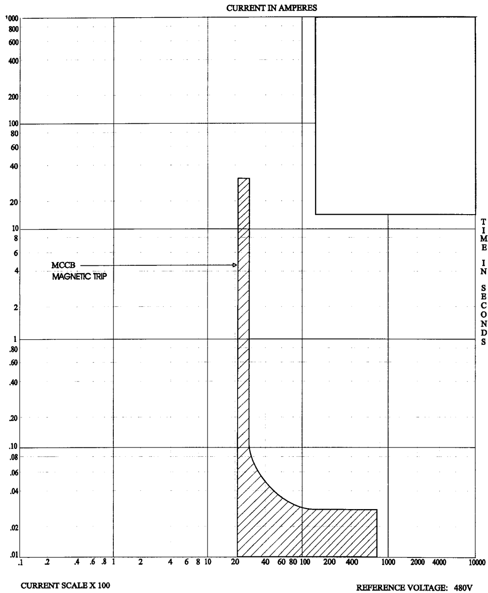
Figure 15-10—Magnetic-trip MCCB operating characteristic
