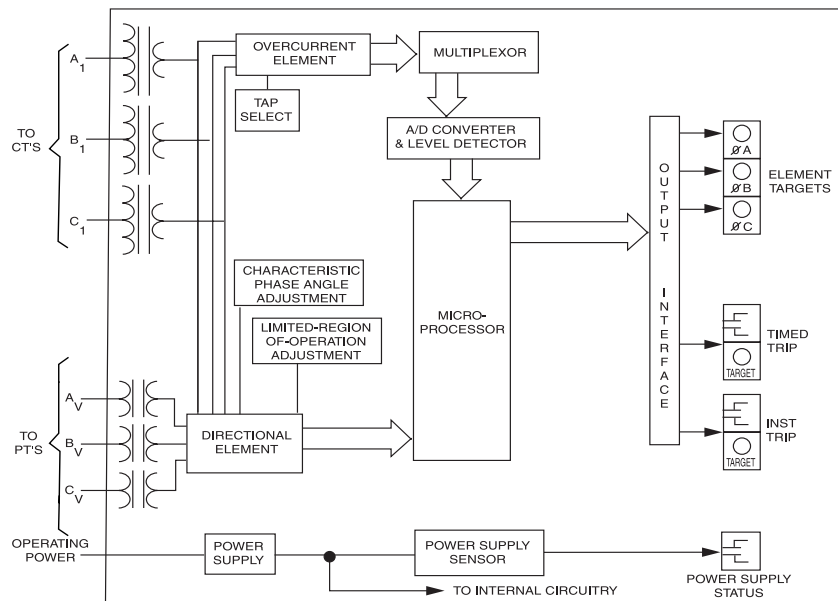
Figure 4-25—Block diagram of a static directional overcurrent relay
