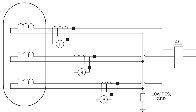
Figure 12-14—Self-balancing protection scheme
