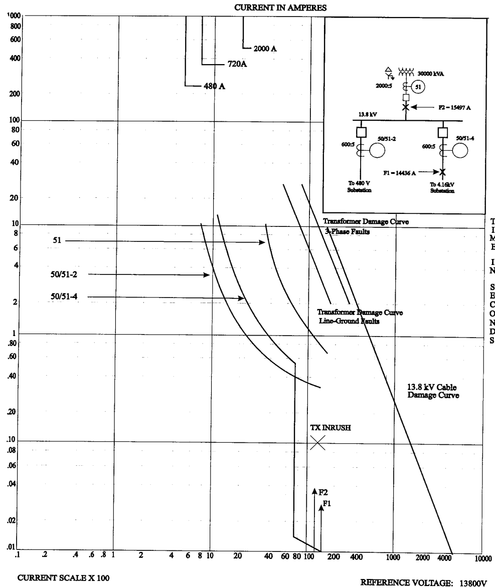
Figure 15-22—30 000 kVA transformer secondary main coordination plot
