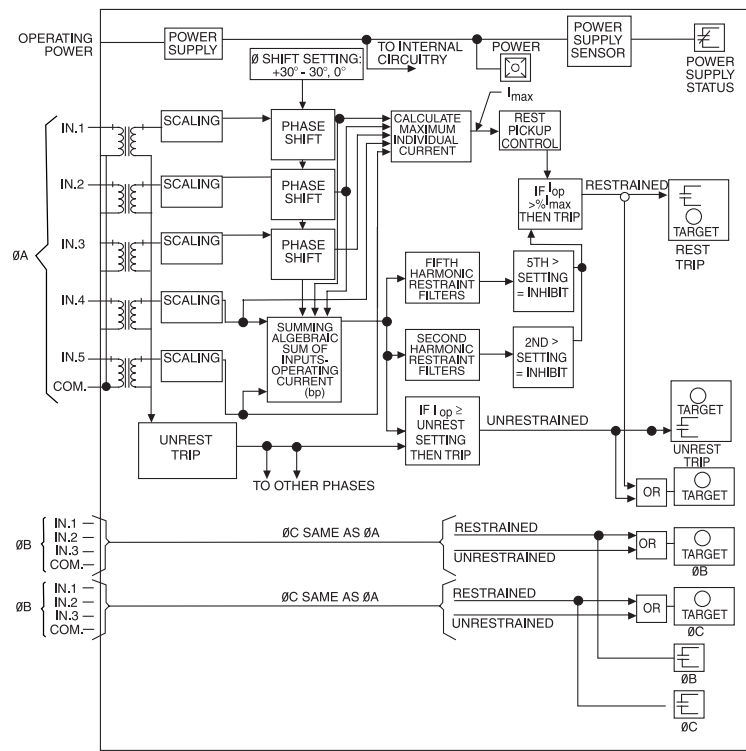
Figure 4-32—Functional block diagram for a static percentage differential relay
