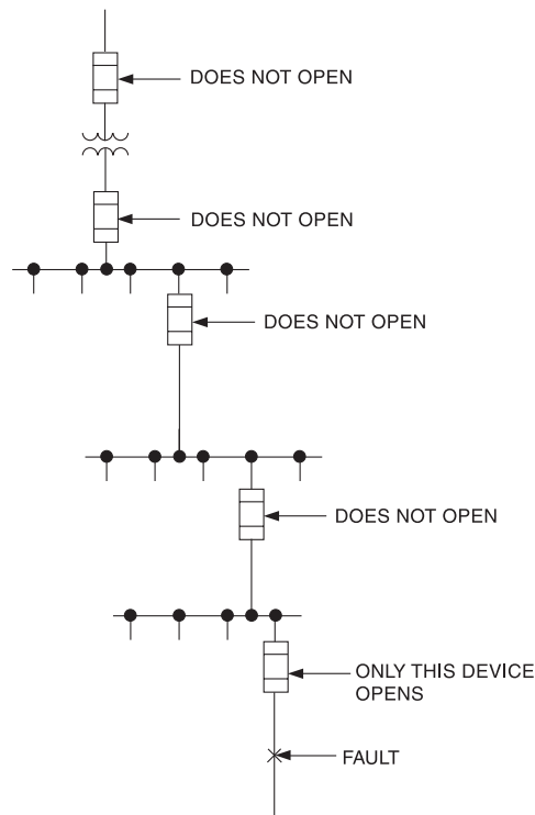
Figure 5-11 — Selective operation of overcurrent protective devices
