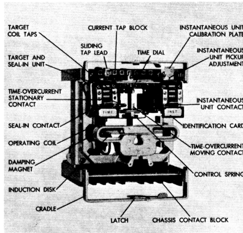
Figure 4-16—Induction disk overcurrent relay with instantaneous attachment (relay removed from drawout case)
