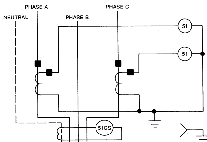
Figure 3-8—Vee- or open-delta-connected CTs
