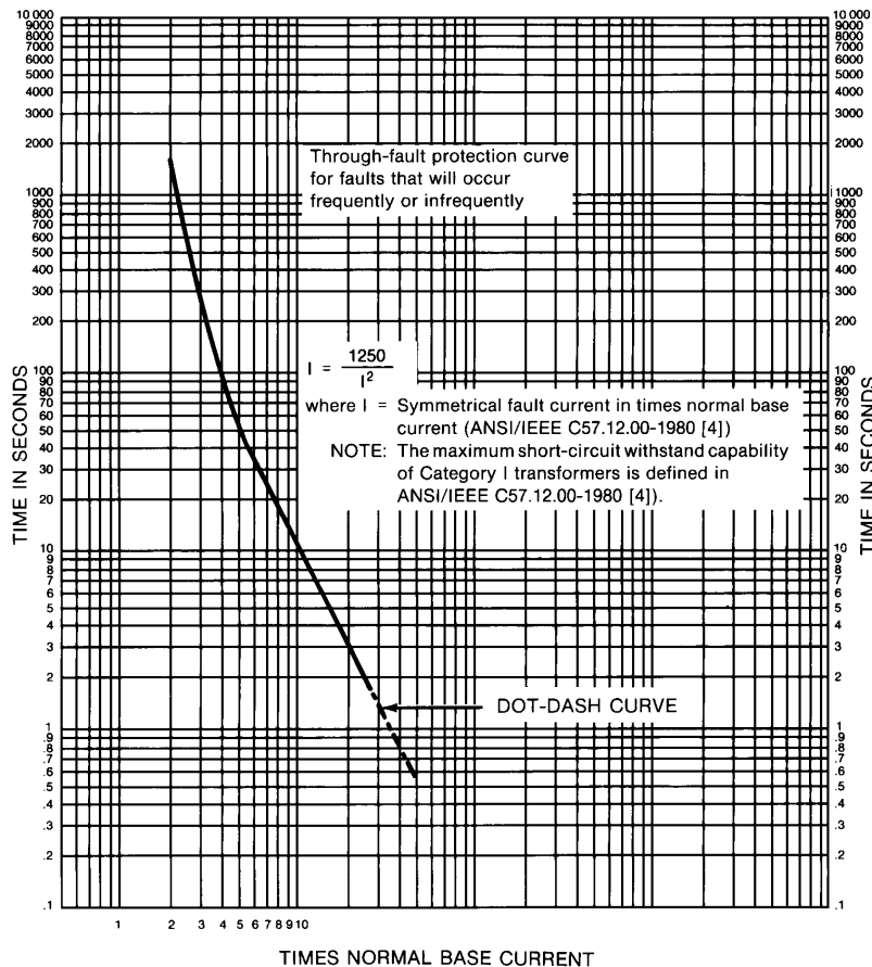
Figure 11-19—Through-fault protection curve for liquid-immersed Category I transformers (5–500 kVA single-phase, 15–500 kVA three-phase)
