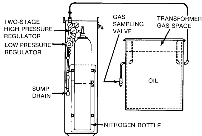
Figure 11-2—Positive-pressure inert-gas assembly, often used on sealed-tank transformers rated 7500 kVA and above and 69 kV and above primary voltage
