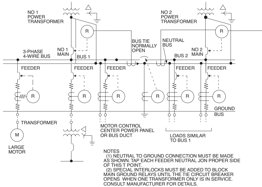
Figure 8-24—Four-wire solidly grounded secondary selective system
