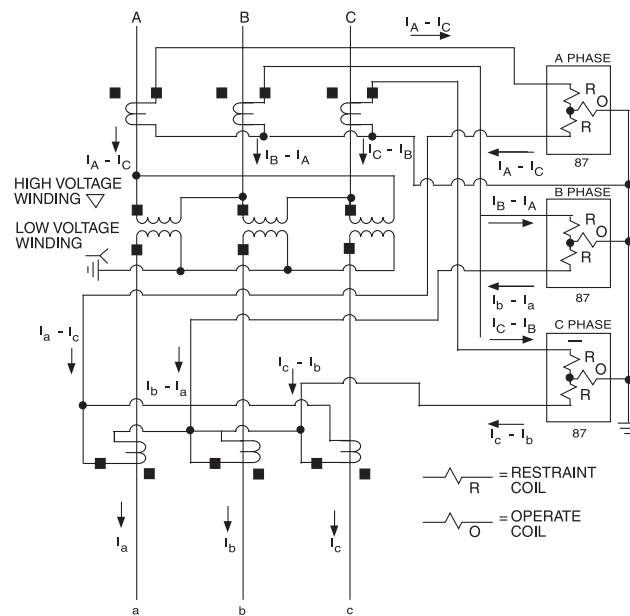
Figure 4-33—Harmonic-restraint percentage differential relay connection diagram for a delta-wye connected transformer
