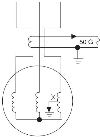
Figure 10-13—Ground-fault overcurrent protection using window CT
