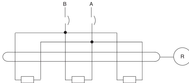
Figure 8-11b—Differential protection multiple loads
