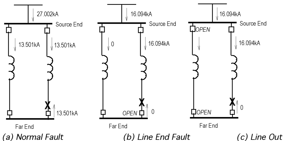
Figure 2-18—Distinctions between normal bus faults, line-end faults, and line-out fault conditions
