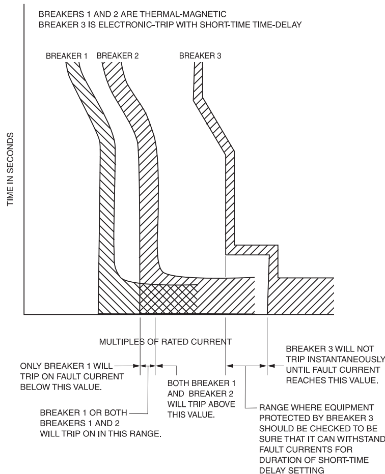
Figure 7-11 — Coordinated tripping by overlapping TCC curves
