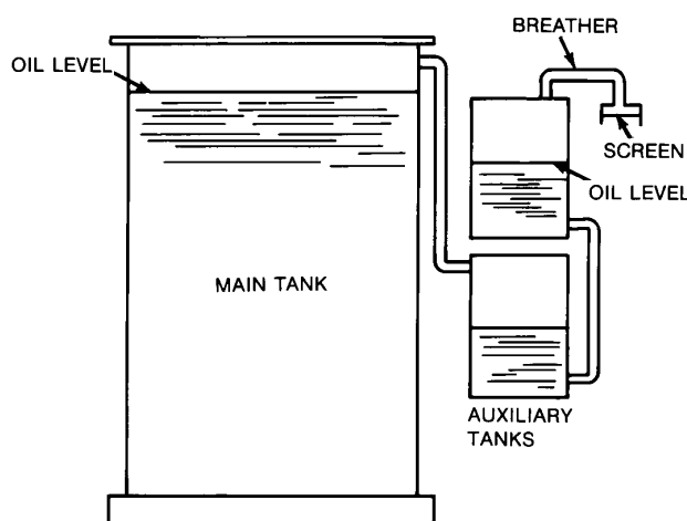
Figure 11-3—Gas-oil seal system of oil preservation
