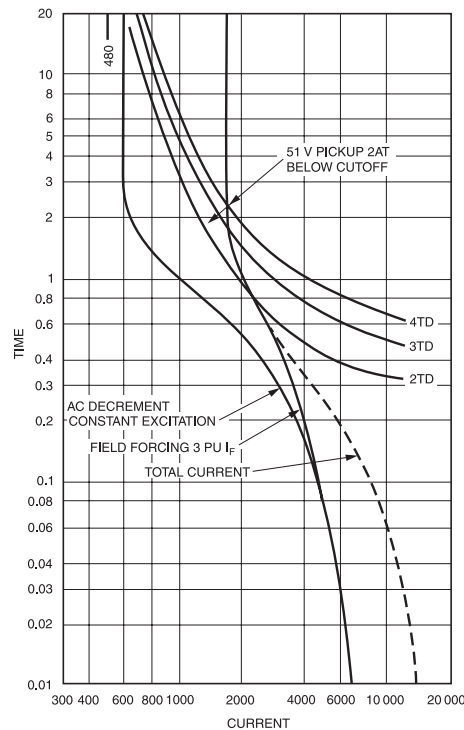
Figure 12-32—Voltage-controlled relay, 19 500 kVA generator, fault-current decrement curves with backup overcurrent relays
