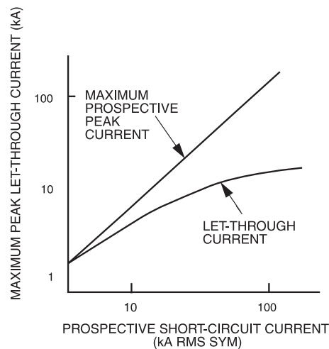
Figure 7-9a—Limited peak let-through current characteristics
