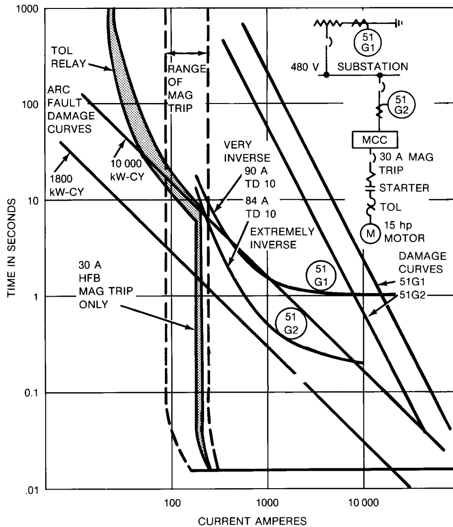
Figure 15-24—Ground-fault protection with 11 kW motor load time-overcurrent relays
