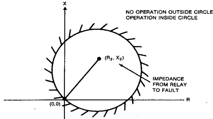
Figure 4-3—R-X diagram for the mho relay
