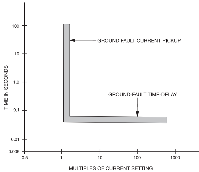
Figure 7-8a—Ground-fault TCC curve ( I^2t OUT) for electronic trip circuit breaker
