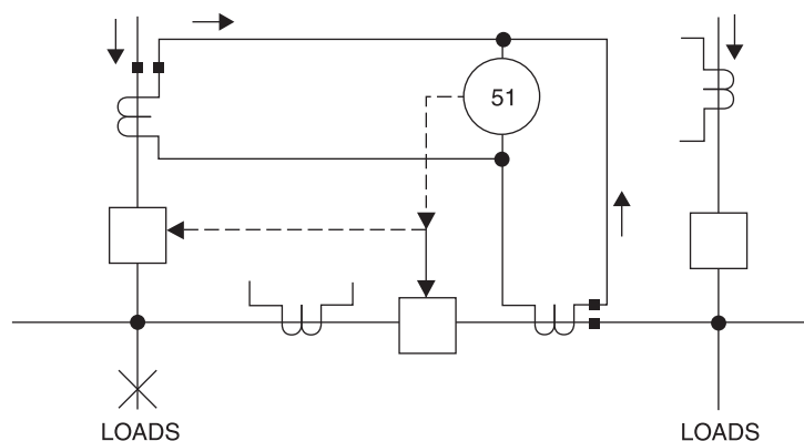
Figure 13-7—Partial differential relaying (three-breaker scheme)
