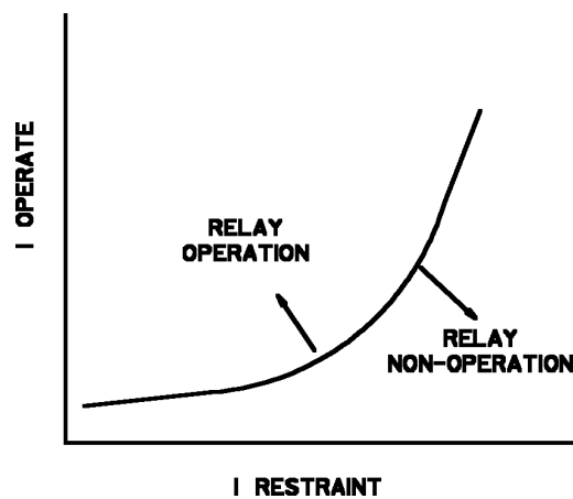
Figure 12-11—Variable slope differential relay
