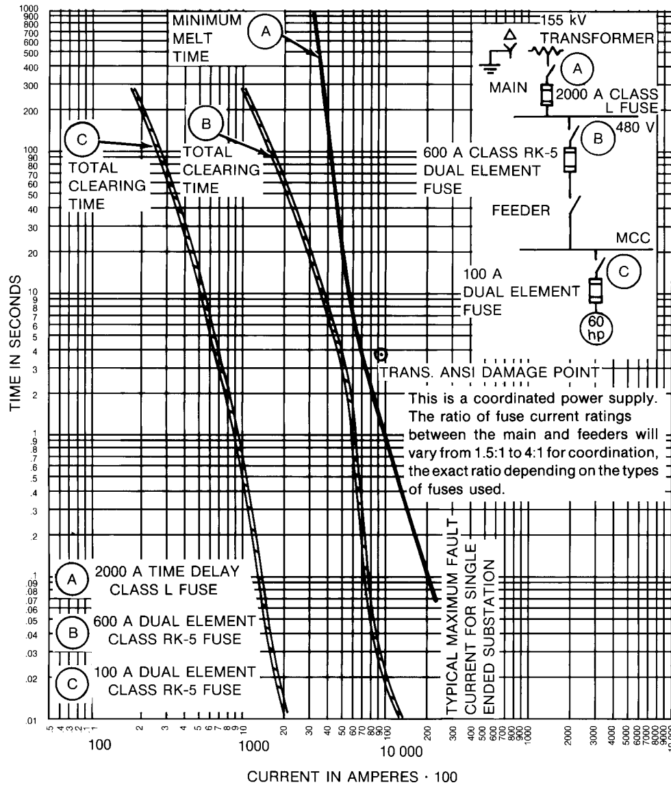
Figure 15-27—Ground-fault TCC curves Example 3
