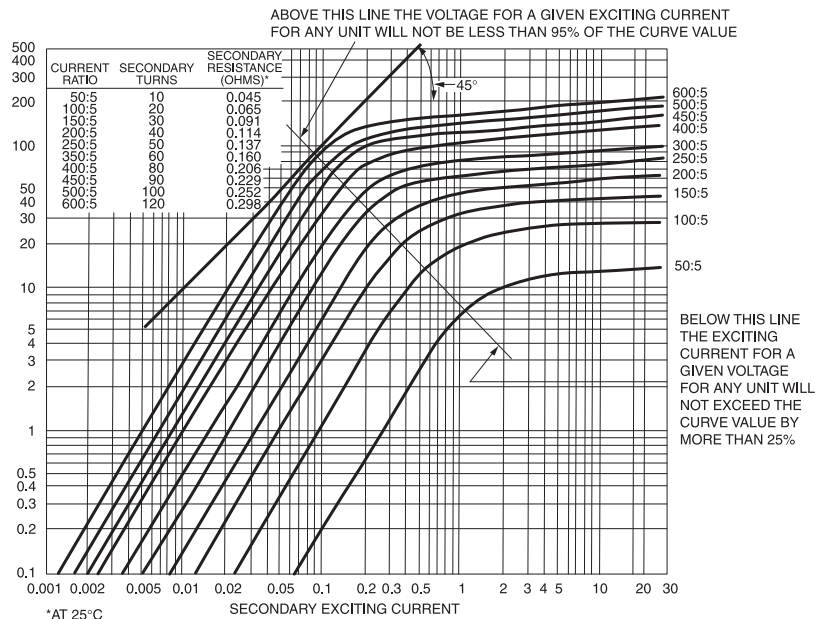
Figure 3-4—Secondary excitation curves for various turn ratios of a specific CT
