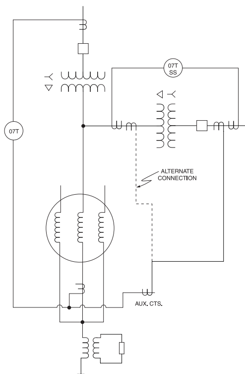
Figure 12-15—Overall differential scheme of generator phase-fault backup protection
