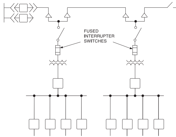
Figure 6-6—One-line diagram of simple radial system
