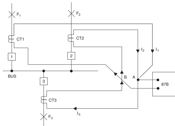
Figure 13-5—Voltage differential relaying
