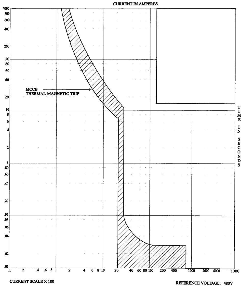
Figure 15-9—Thermal-magnetic MCCB operating characteristic
