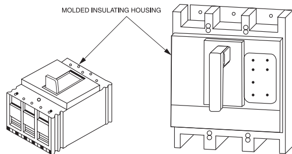
Figure 7-1a—MCCB
