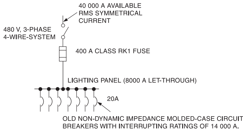
Figure 5-20—Application of fuses to protect molded-case circuit breakers
