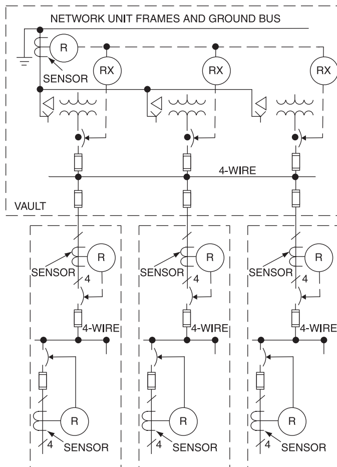
Figure 8-29—Ground-fault protection for typical three-transformer spot network
