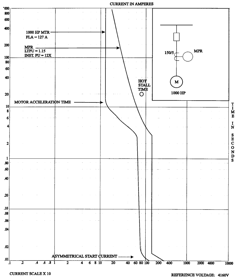
Figure 15-11a—Motor protection using a motor protection relay
