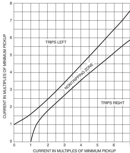
Figure 4-14—Typical current balance relay operating characteristic
