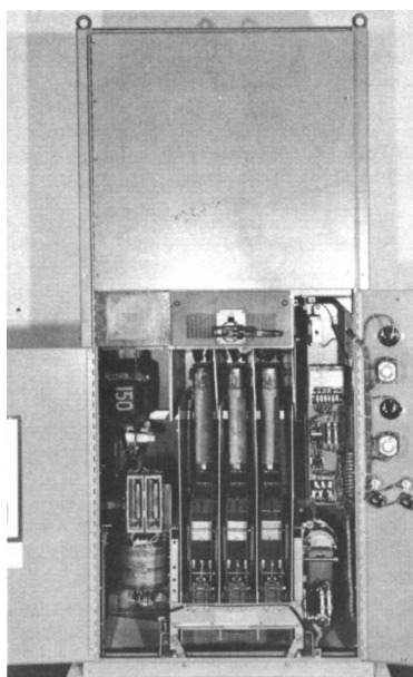
Figure 6-13—High-voltage R-rated fuses in drawout motor starter, rated 180 A
