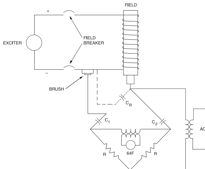
Figure 12-24—Field ground-fault protection using pilot brushes
