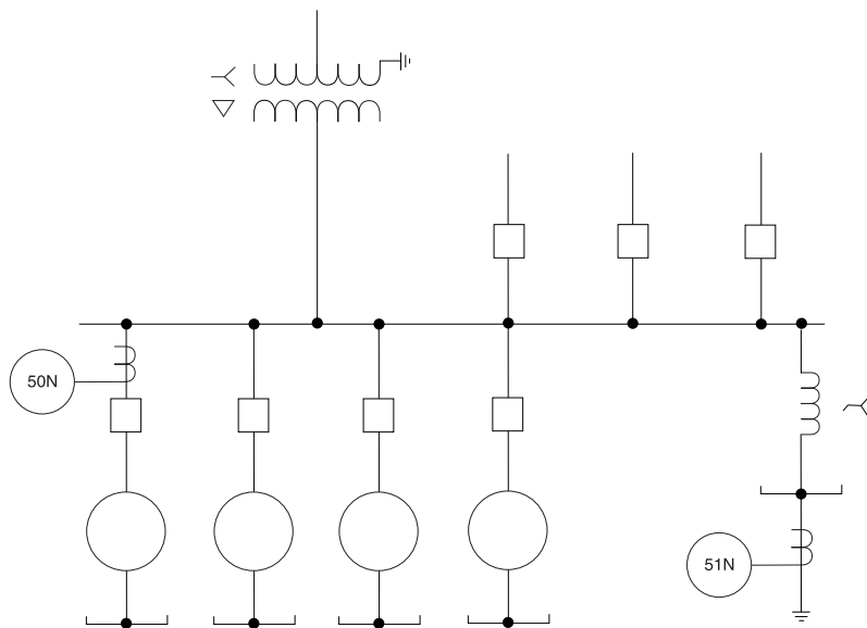
Figure 12-21 — Ground-fault protection with zigzag grounding bank
