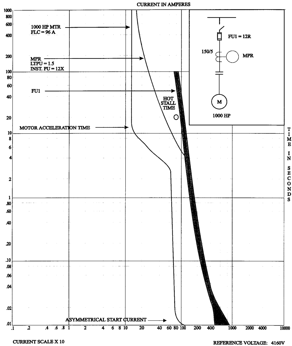
Figure 15-11b—Motor protection using a motor protection relay in combination with a fuse
