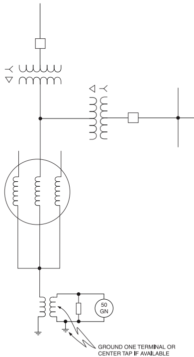
Figure 12-17—Generator ground-fault protection for high-impedance-grounded generator
