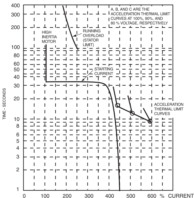
Figure 10-2—Typical time-current and thermal limit characteristic curves
