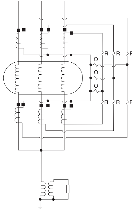
Figure 12-12—Percentage differential relay connection for six-bushing wye-connected generator
