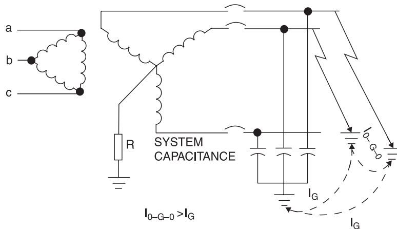
Figure 8-4b—High-resistance grounding with phase-to-ground-to-phase fault
