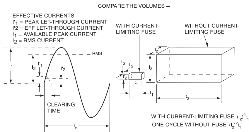
Figure 5-2—Graphic representation of I^2t
