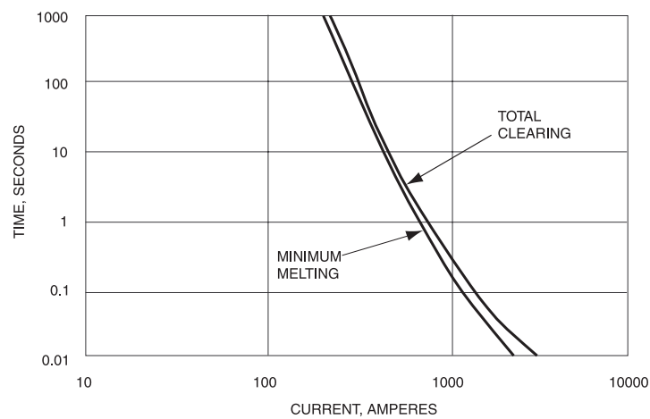
Figure 6-2— Typical TCC curves for a current-limiting fuse
