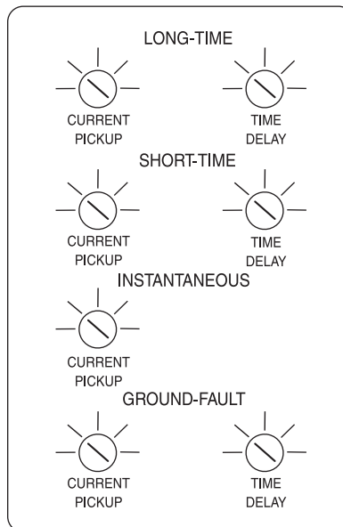
Figure 7-5—Electronic trip unit with long-time, short-time, instantaneous, and ground-fault adjustments
