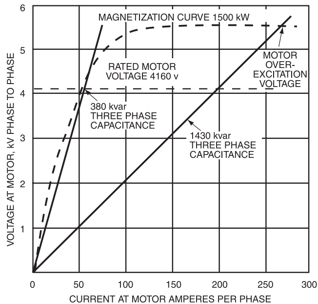
Figure 10-20—Excess shunt capacitance from utility line, which is likely to overexcite a large high-speed motor
