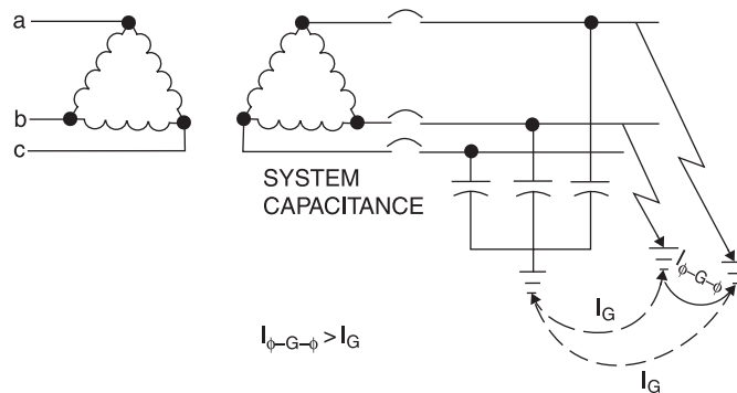
Figure 8-5b—Ungrounded system with phase-to-ground-to phase fault
