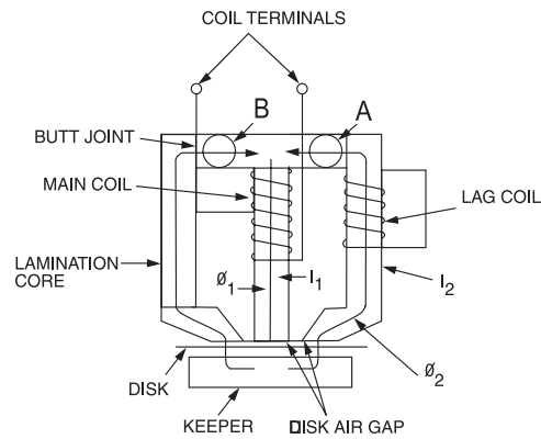
Figure 4-17—Elementary induction disk relay
