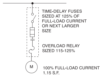
Figure 5-24—Application of time-delay fuses for typical motor circuit
