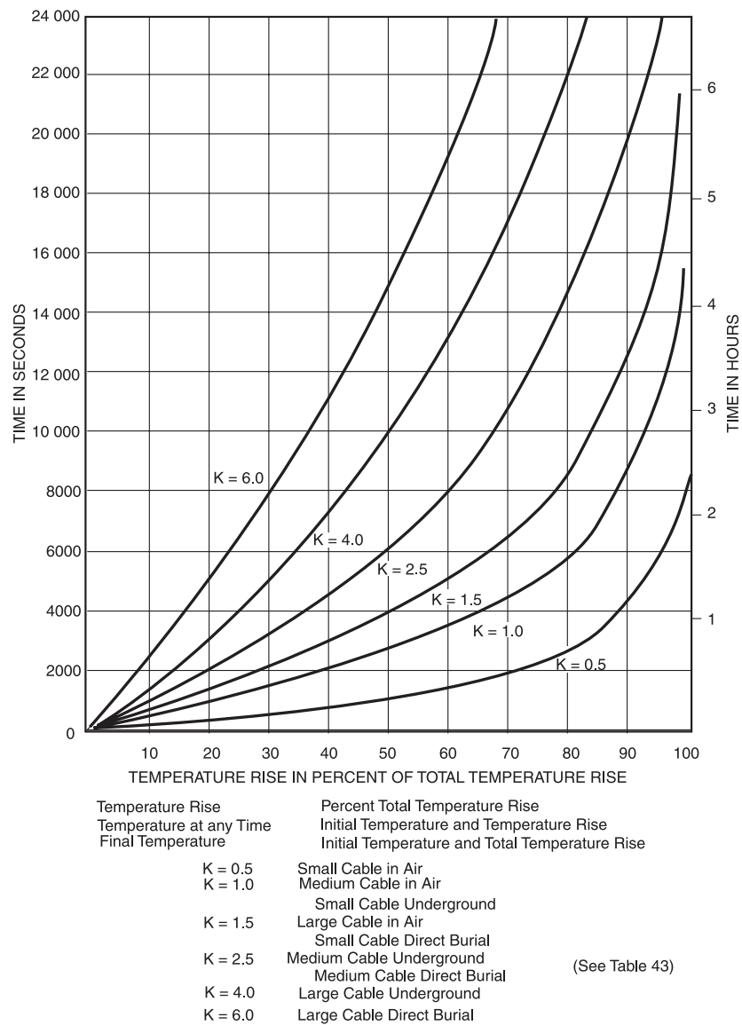
Figure 9-16—Rate of temperature rise due to current increase
