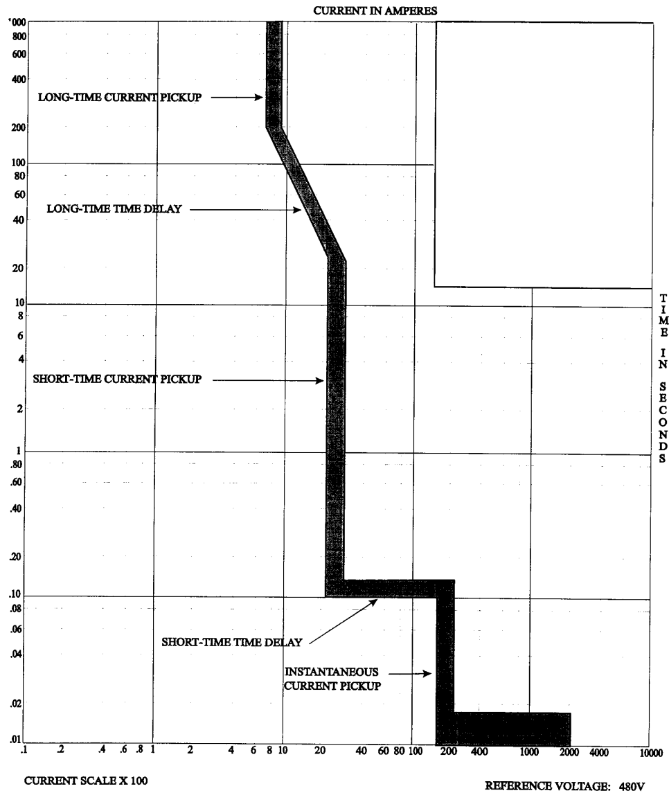
Figure 15-8—Typical electronic low-voltage circuit breaker trip characteristic
