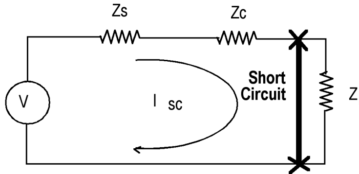
Figure 2-2—Equivalent circuit used to calculate short-circuit current
