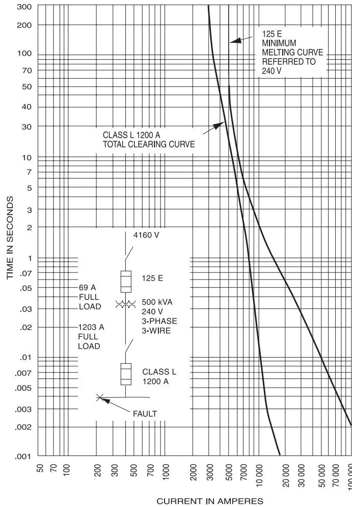
Figure 5-16—Typical coordination study of primary and secondary fuses showing selective system
