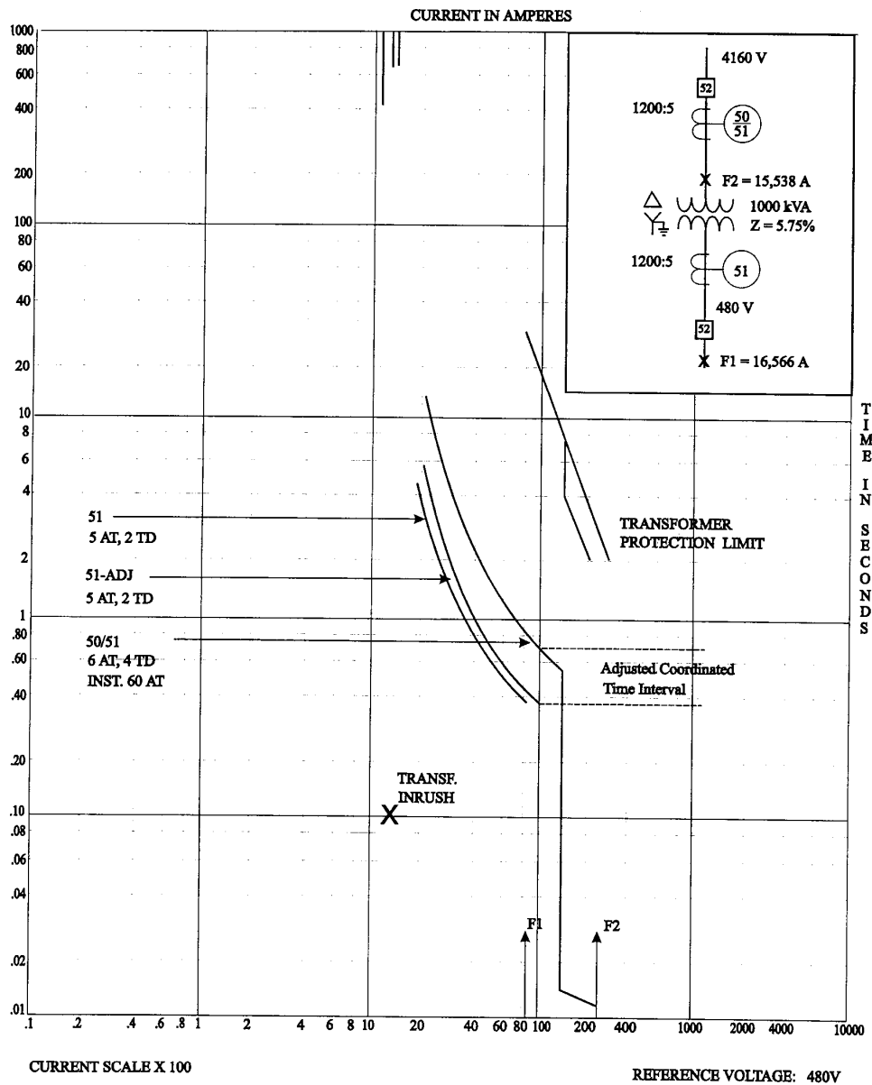
Figure 15-4a—Coordination plot for transformer primary protection using protective relay
