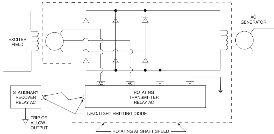
Figure 12-25—Field ground-fault protection for brushless machines
