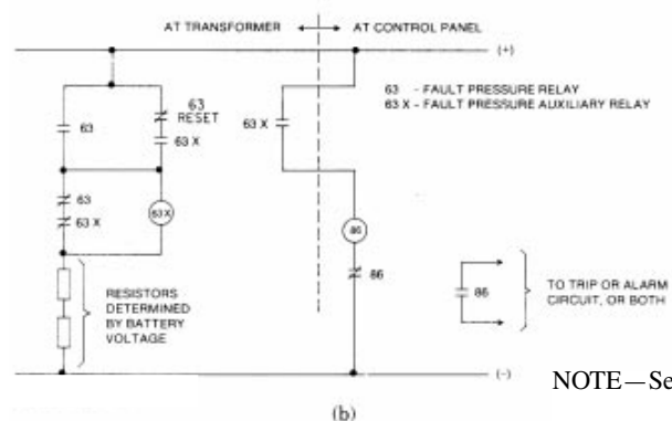
Figure 11-12—Fault pressure relay schemes (a) Auxiliary relay at control panel (b) Auxiliary relay at transformer with manual reset
