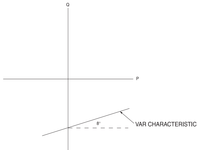
Figure 4-11—Var relay operating characteristic in the complex power plane
