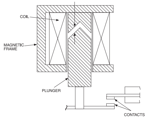
Figure 4-19—Solenoid (or plunger) instantaneous relay
