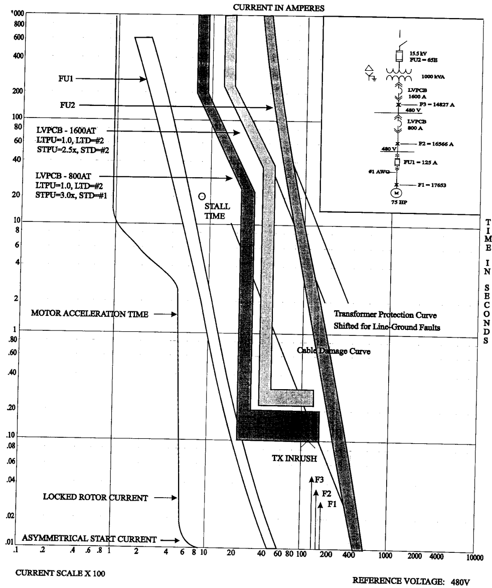
Figure 15-17—1000 kVA transformer primary fuse coordination plot
