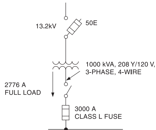
Figure 5-22—Sizing of low-voltage fuses for transformer secondary protection
