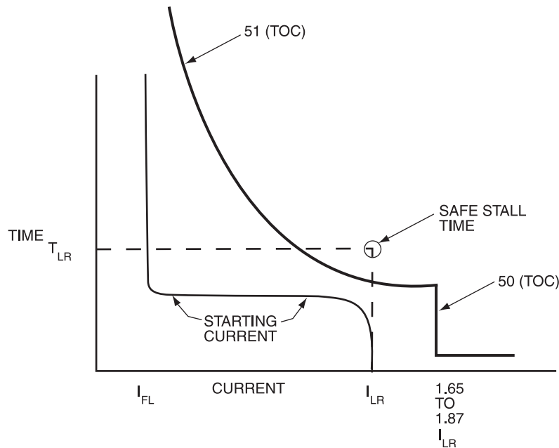
Figure 10-5—Conventional overcurrent relay protection of motor
