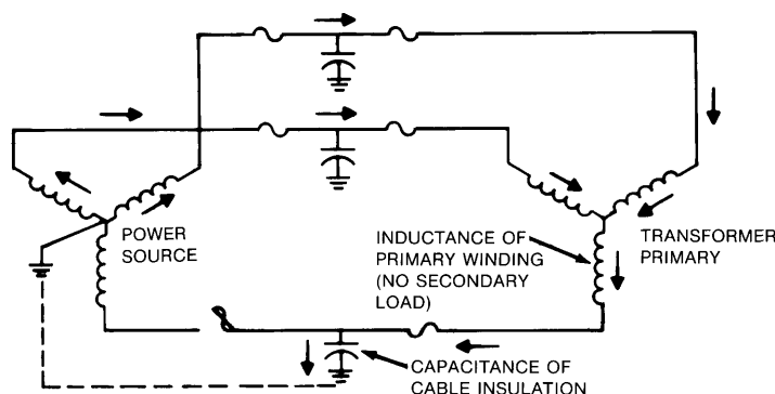
Figure 11-31—One-line diagram showing current flow that may result in ferroresonance
