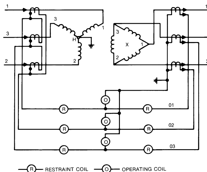
Figure 11-26—Typical schematic connections for percentage differential protection of a wye-delta transformer
