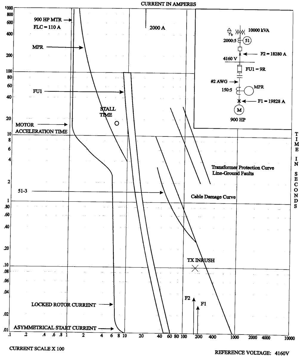
Figure 15-19—10 000 kVA transformer secondary main coordination plot
