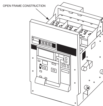
Figure 7-1b—LVPCB
