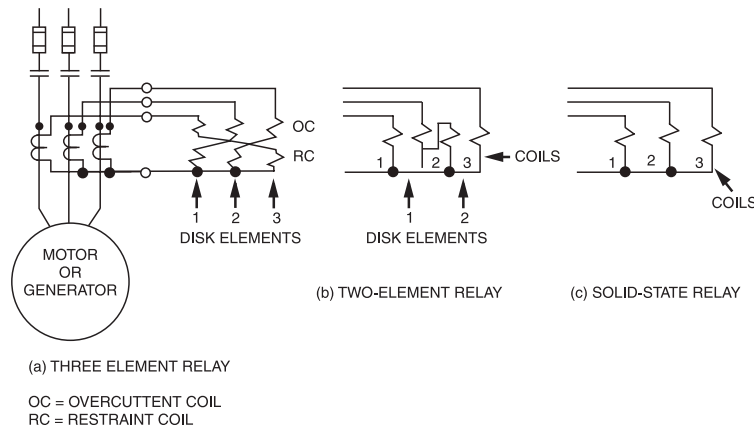
Figure 4-13—Current balance relay connection diagrams
