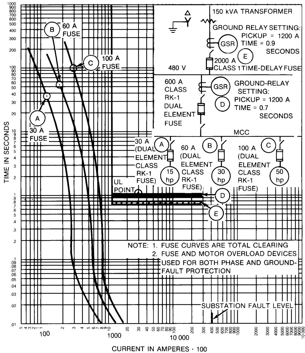
Figure 15-26—Ground-fault TCC curves Example 2
