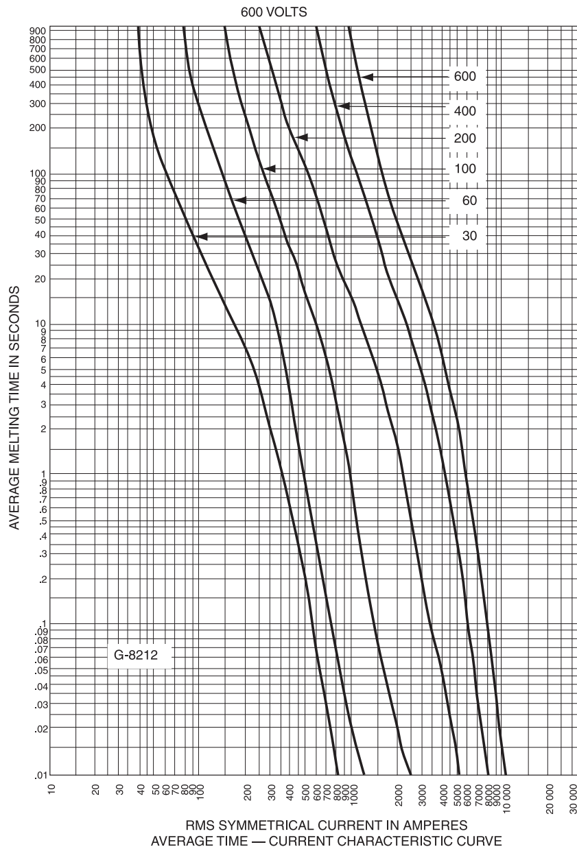
Figure 5-13—Time-delay fuses, Class RK-5
