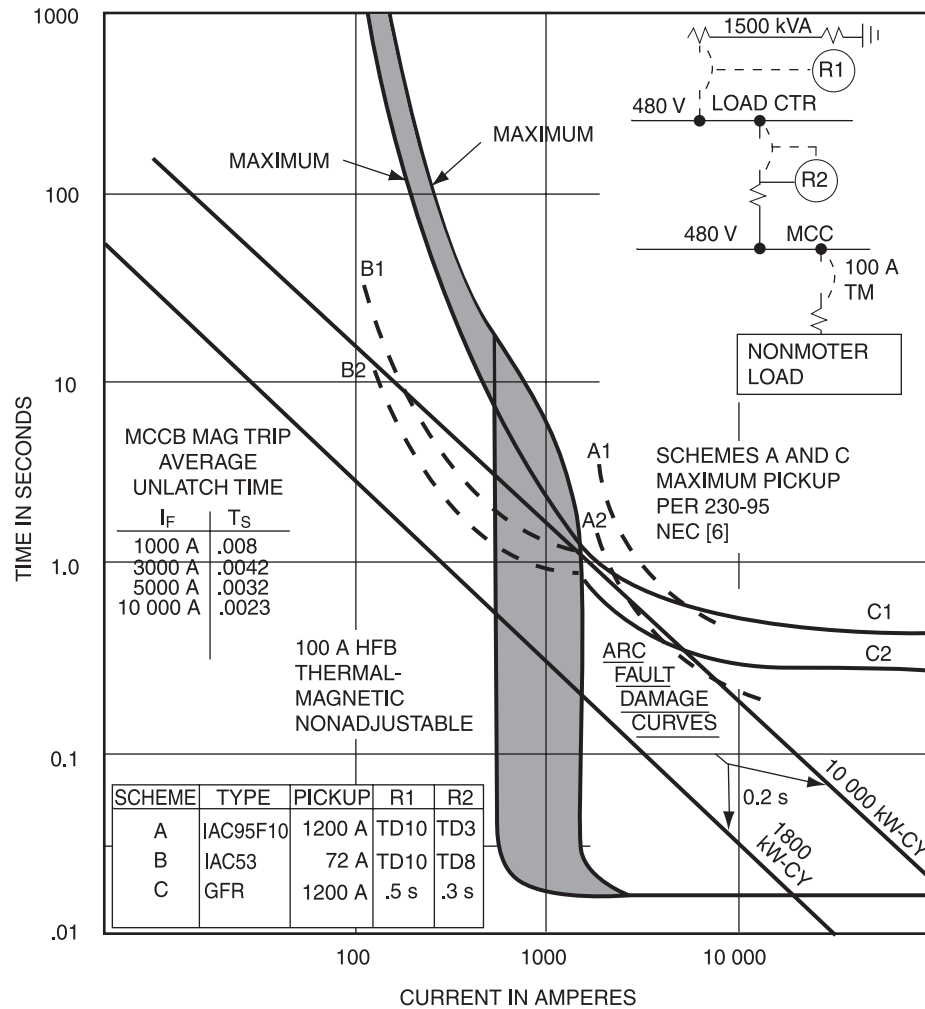
Figure 8-15b—Minimum ground-fault protection for a nonmotor circuit
