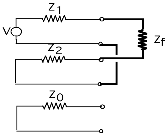
Figure 2-10—Sequence interconnections for a phase-to-phase fault not involving ground
