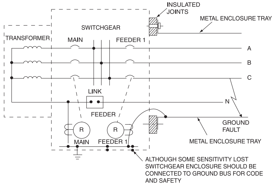
Figure 8-10—Ground-return relay scheme
