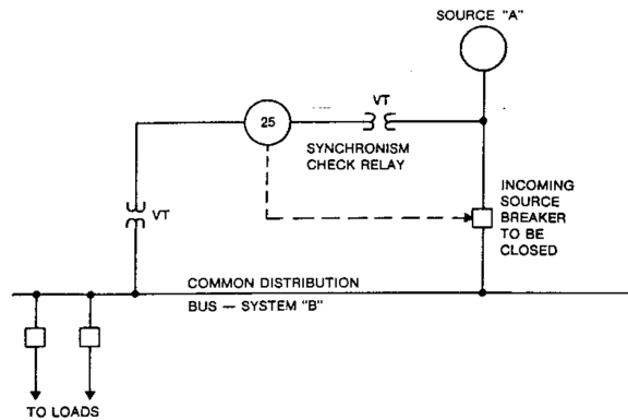
Figure 4-6a—Application of synchronism check relay to connect two systems together
