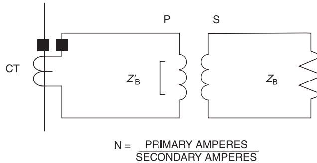
Figure 3-10—Auxiliary CTs
