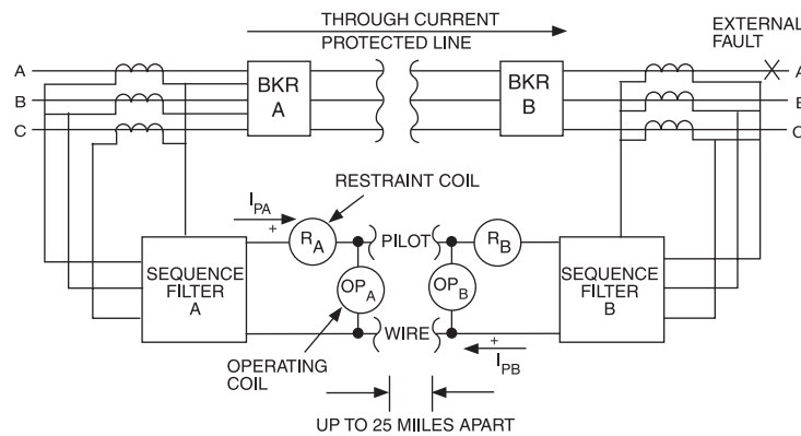
Figure 4-35—Simplified connections for a pilot wire differential relay
