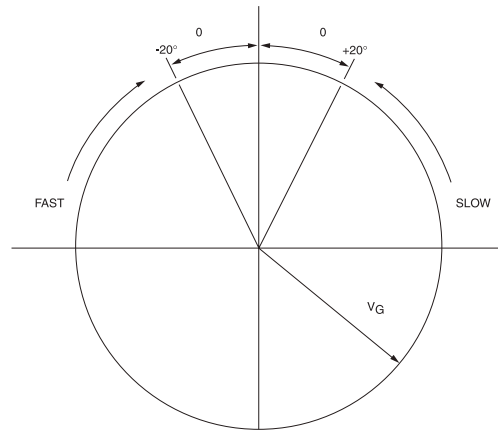
Figure 4-6d—Application of synchronizing relay
