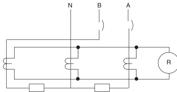
Figure 8-11a—Differential protection center-tapped loads
