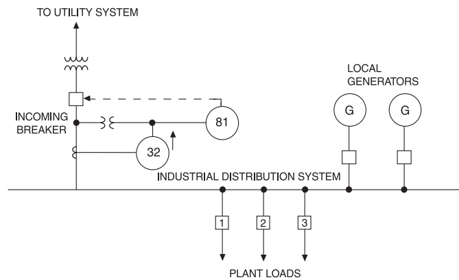
Figure 4-27c—Tripping incoming breaker for power outflow to external loads
