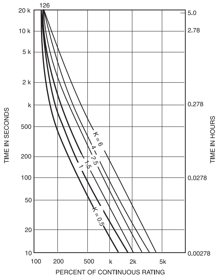
Figure 9-17a—Emergency overload current percent of continuous rating, EPR-XLP cable, insulated, 40 °C ambient temperature
