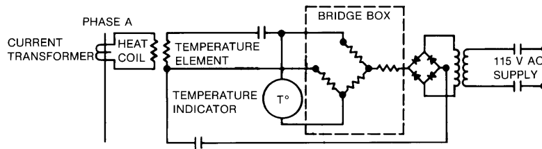
Figure 11-16—Hot-spot temperature indicator, which utilizes Wheatstone bridge method to determine transformer temperature
