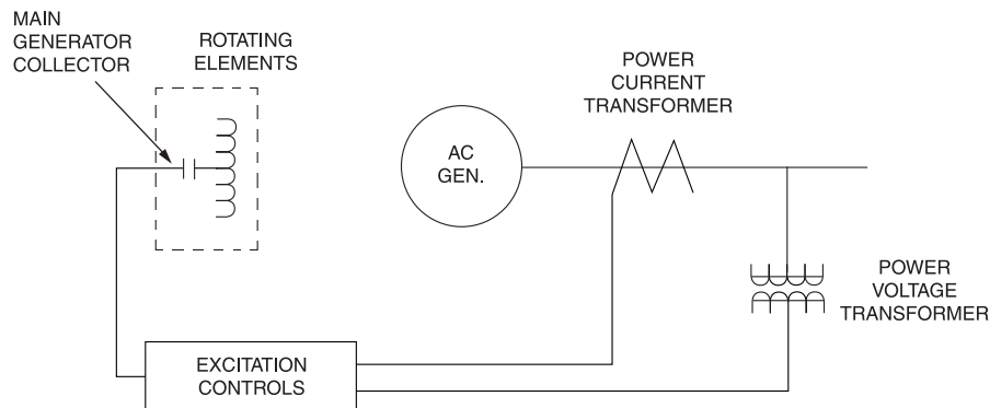
Figure 12-7—System with static exciter
