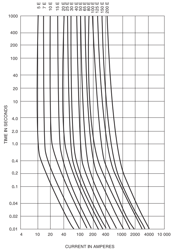
Figure 6-8—Typical minimum-melting TCC curves for high-voltage current-limiting power fuses
