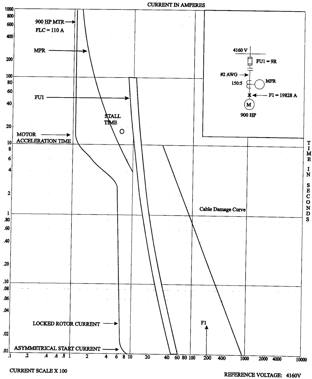
Figure 15-18—4160 V-680 kW motor protection coordination plot
