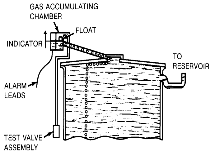
Figure 11-9—Gas-detector relay, which accumulates gases from top air space of transformer (used only on conservator tank units)
