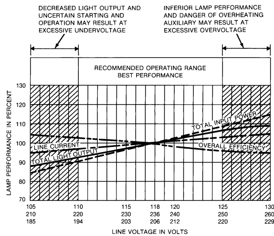
Figure 14-2—Fluorescent lamp performance as affected by voltage
