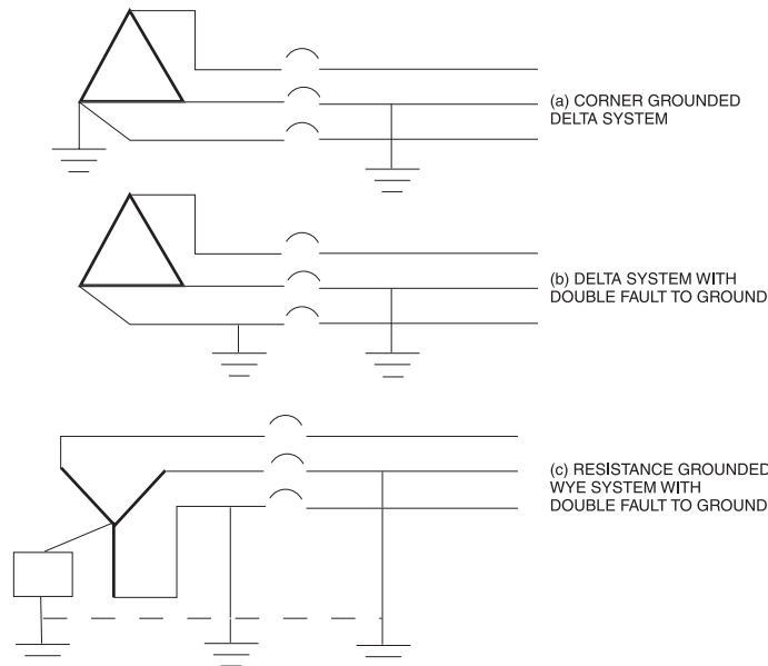
Figure 7-13—Systems requiring special consideration for single-pole faults
