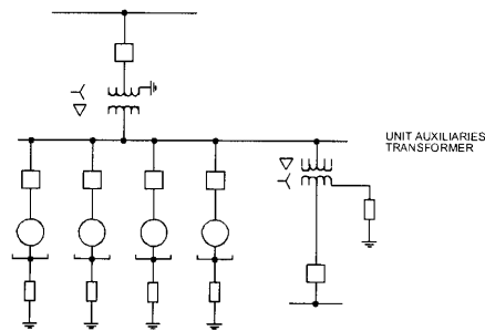
Figure 12-2—Generators sharing a transformer
