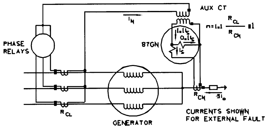
Figure 12-19—Generator ground differential protection using product relay
