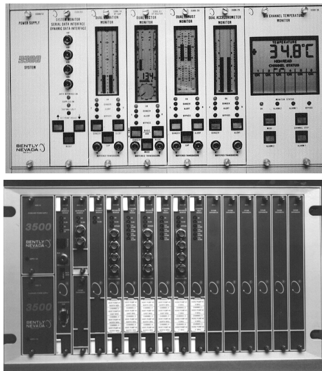
Figure 10-18—Monitoring system panels
