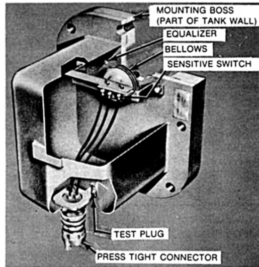
Figure 11-11—Sudden gas-pressure relay mounted on transformer tank above normal oil level
