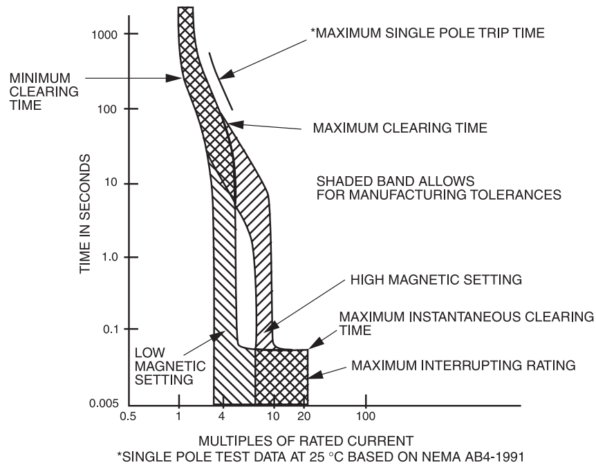
Figure 7-6—Typical TCC curve for a three-pole 600 A frame size MCCB in open air at rated temperature, usually 40 °C
