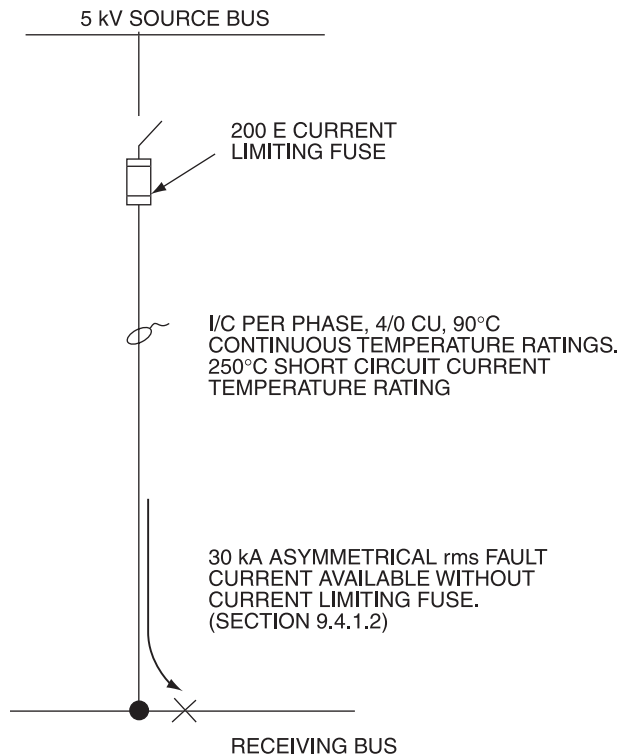
Figure 9-10—One-line diagram for Example 1
