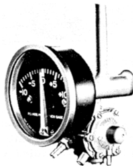
Figure 11-7—Pressure vacuum gauge (which indicates internal gas pressure relative to atmospheric pressure) with bleeder valve (which allows pressure to be equalized manually)
