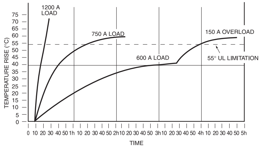
Figure 9-23—Time-temperature curves of 100%, 125%, and 200% loads on a 600 A rated low-impedance busway (31-mm- \times -57-mm aluminum bar per phase)
