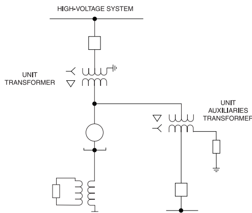
Figure 12-3—Unit generator-transformer configuration
