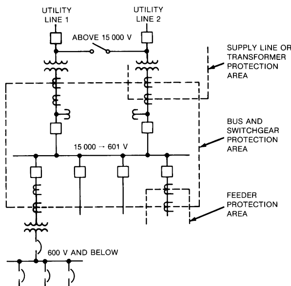
Figure 13-1—Single-bus scheme with bus differential relaying
