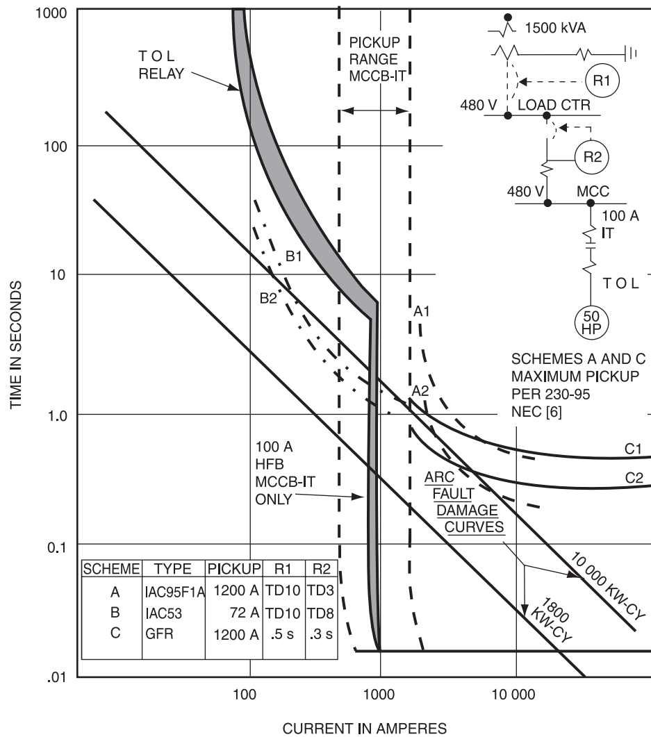
Figure 8-15c—Minimum ground-fault protection for a motor circuit
