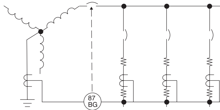
Figure 8-11c—Ground-differential scheme bus and transformer
