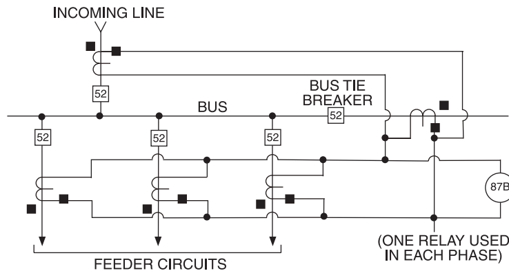
Figure 4-34—High-impedance differential relay used in bus protection, one phase shown
