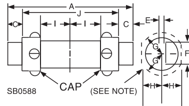
KNIFE-BLADE TYPE CARTRIDGE FUSE – 61-600 A
