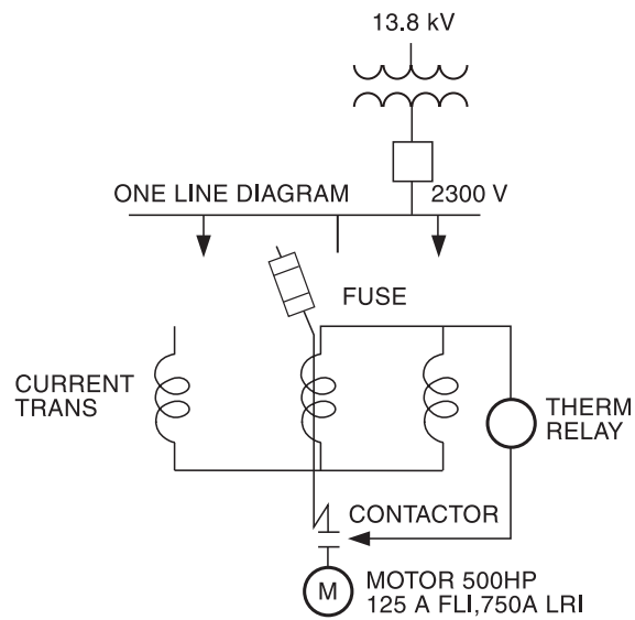
Figure 6-14—One-line diagram of motor branch circuit and connected devices
