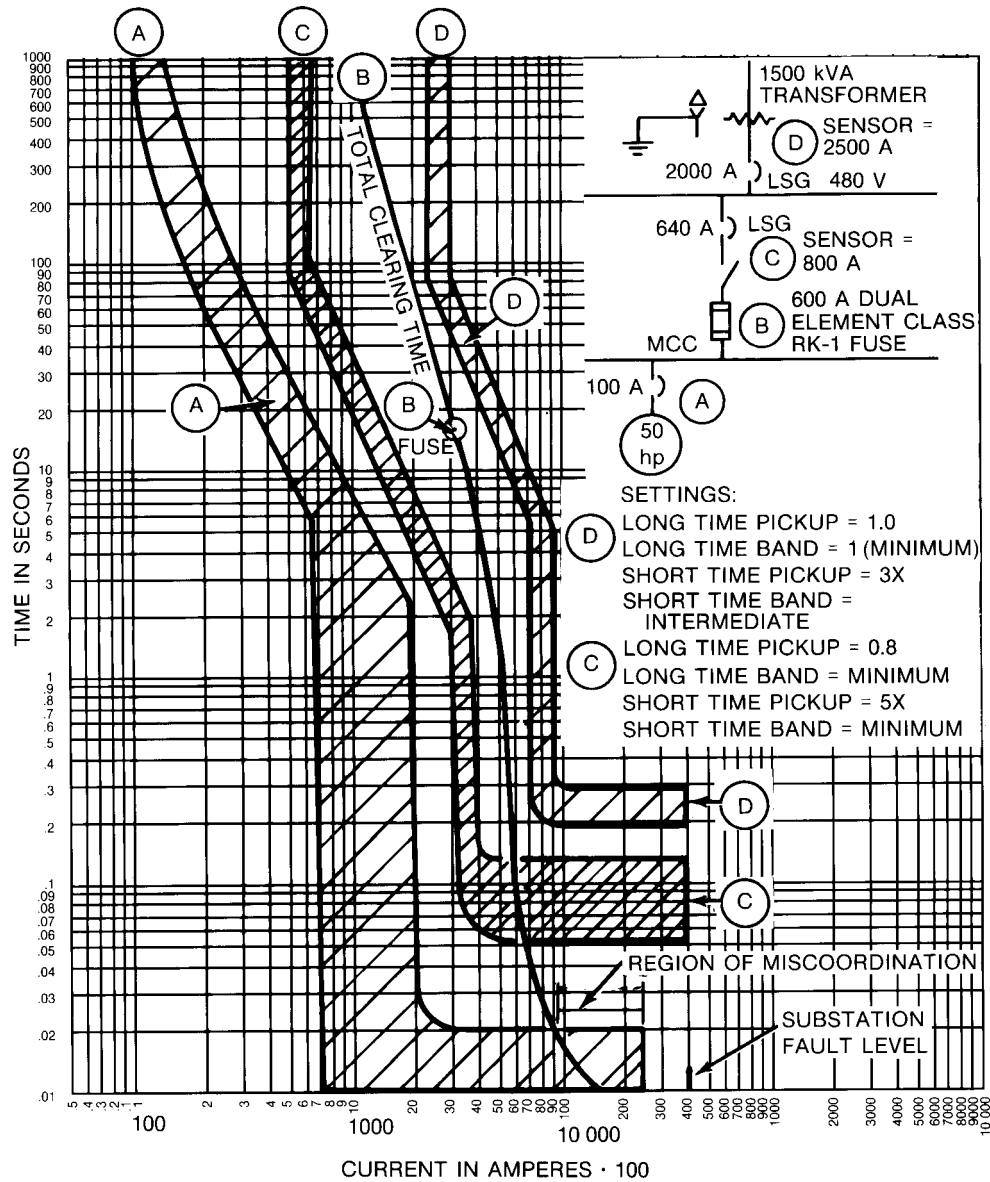
Figure 15-28—Phase-fault TCC curves Example 1
