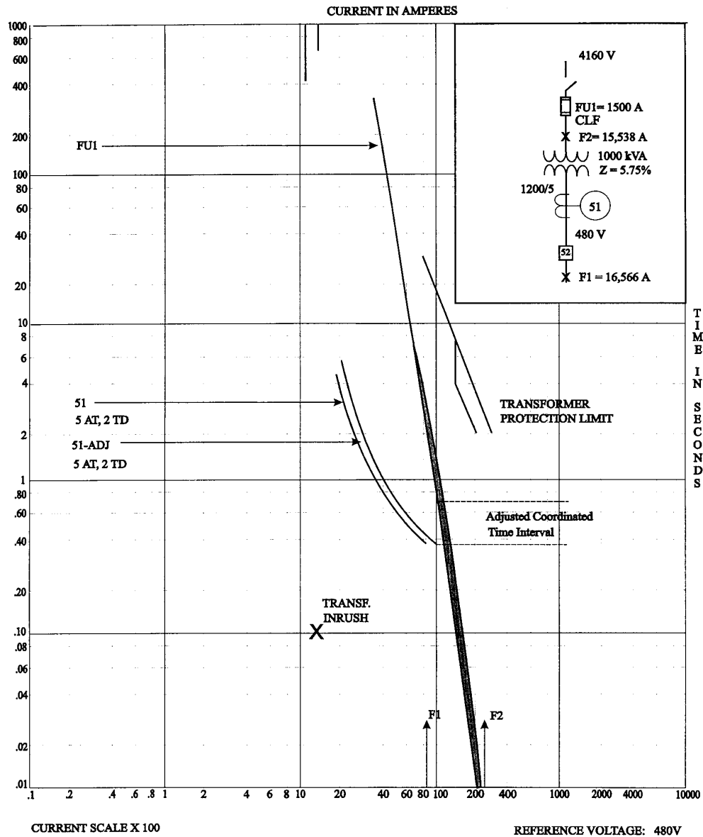
Figure 15-4b—Coordination plot for transformer primary protection using fuse
