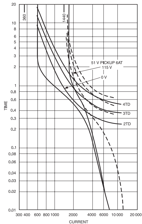
Figure 12-33— Voltage-restrained relay, 19 500 kVA generator, fault-current decrement curves with backup overcurrent relays
