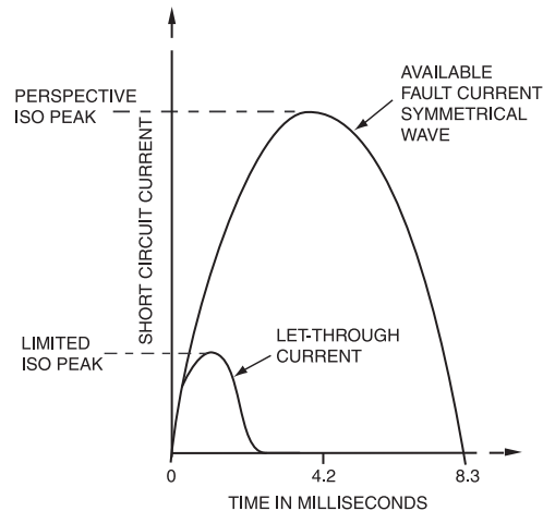
Figure 7-2—Current-limiting waveform (fault initiation at t = 0 and V maximum)
