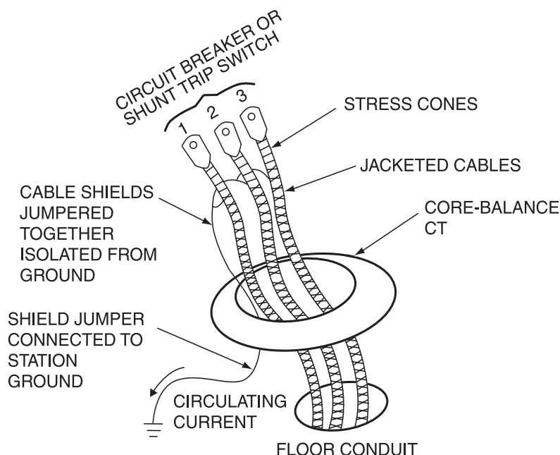
Figure 8-9b—Physical installation of a core-balance CT for shielded cable termination
