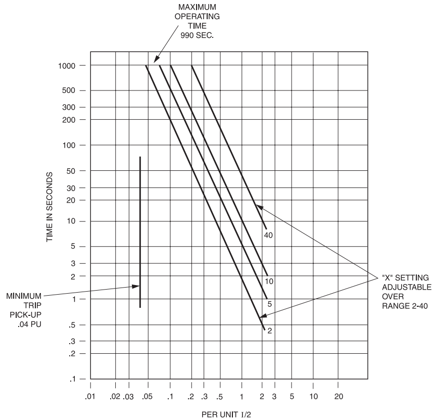
Figure 12-29—Characteristics of static negative-sequence overcurrent relay showing generator I_2^2t limits
