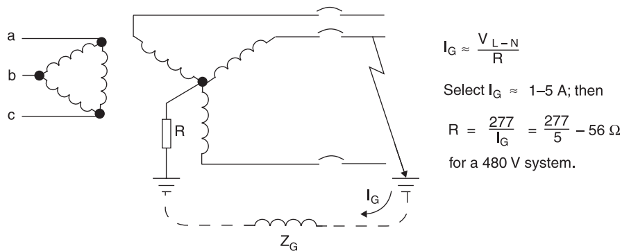
Figure 8-4a—High-resistance grounding (may use ground relays to alarm on first fault, trip on second fault)
