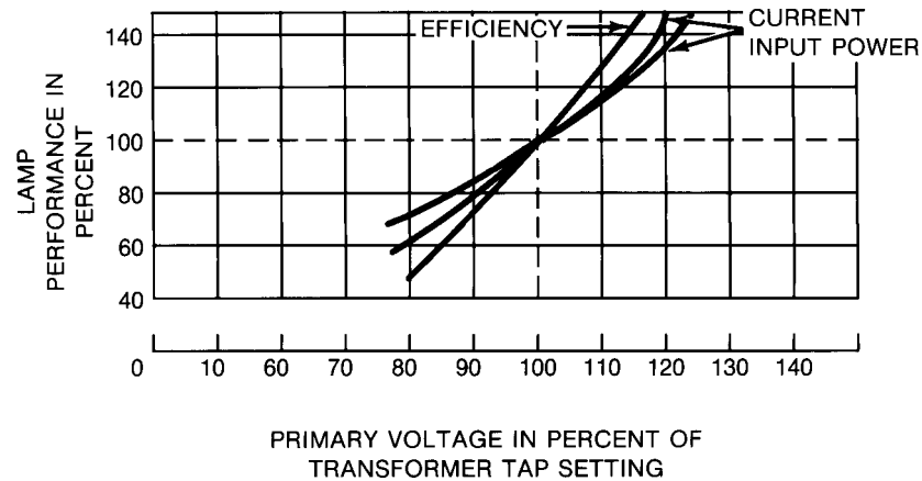
Figure 14-3—Mercury lamp performance as affected by voltage (120 V basis)
