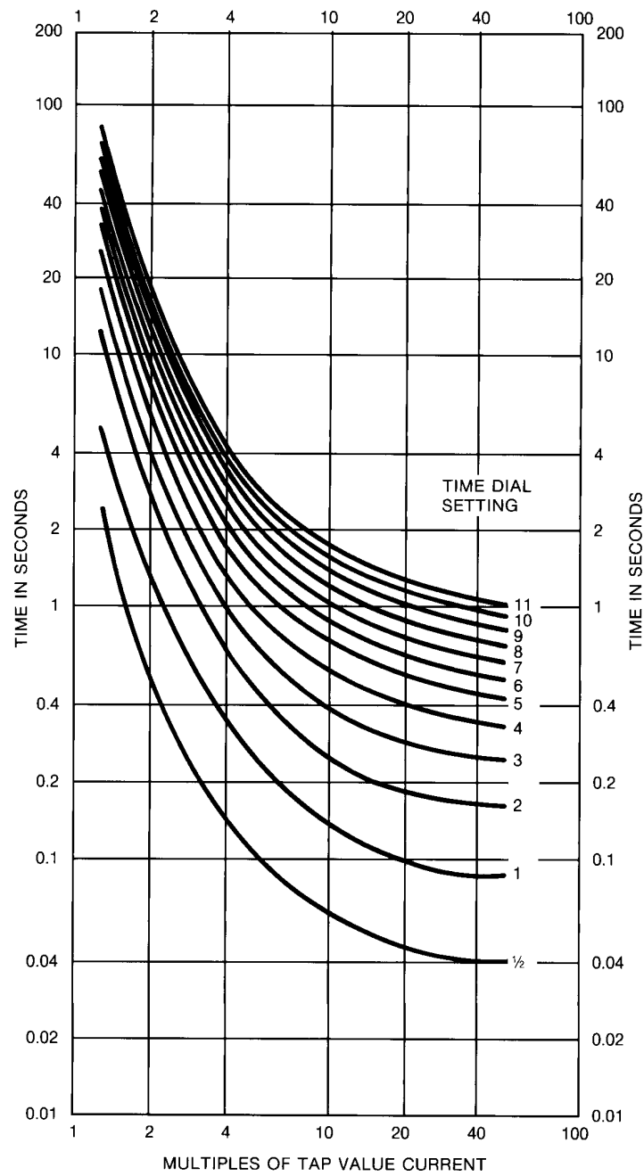
Figure 15-6—Typical time-current curves for very inverse-time relay
