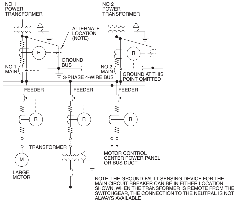
Figure 8-23—Four-wire solidly grounded system with dual supply
