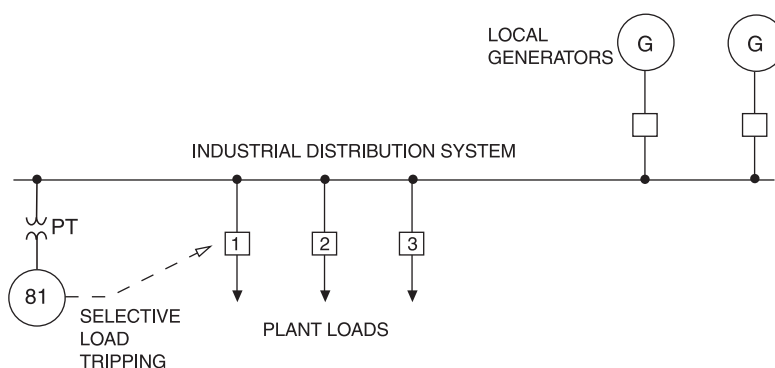
Figure 4-27a—Load-shedding scheme for system with only local generation
