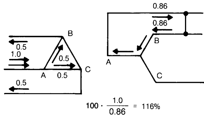
Figure 15-1—Currents in delta-wye grounded transformer for secondary phase-to-phase faults
