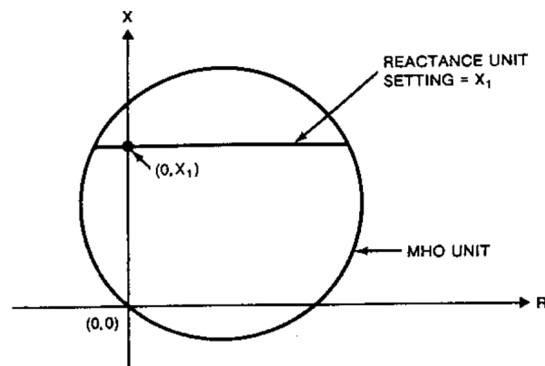
Figure 4-4a—R-X diagram for mho relay being applied as a loss-of-field relay for a synchronous generator
