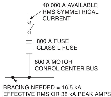
Figure 5-19—Example for determining bus-bracing requirements of 800 A motor-control center
