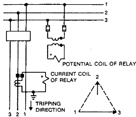
Figure 4-10—Directional power relay connection diagram
