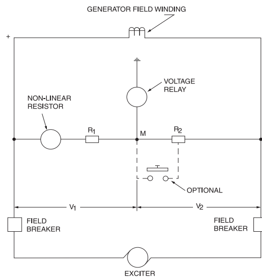
Figure 12-23—Field ground-fault protection using a voltage divider
