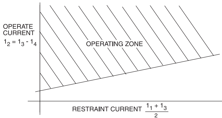
Figure 4-31b—Typical operating characteristic of a variable percentage restraining differential relay
