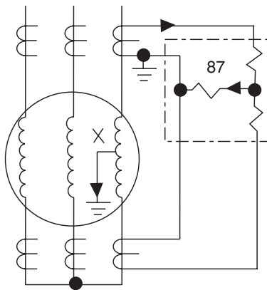
Figure 10-10—Conventional phase differential protection using three percentage differential relays (one shown)
