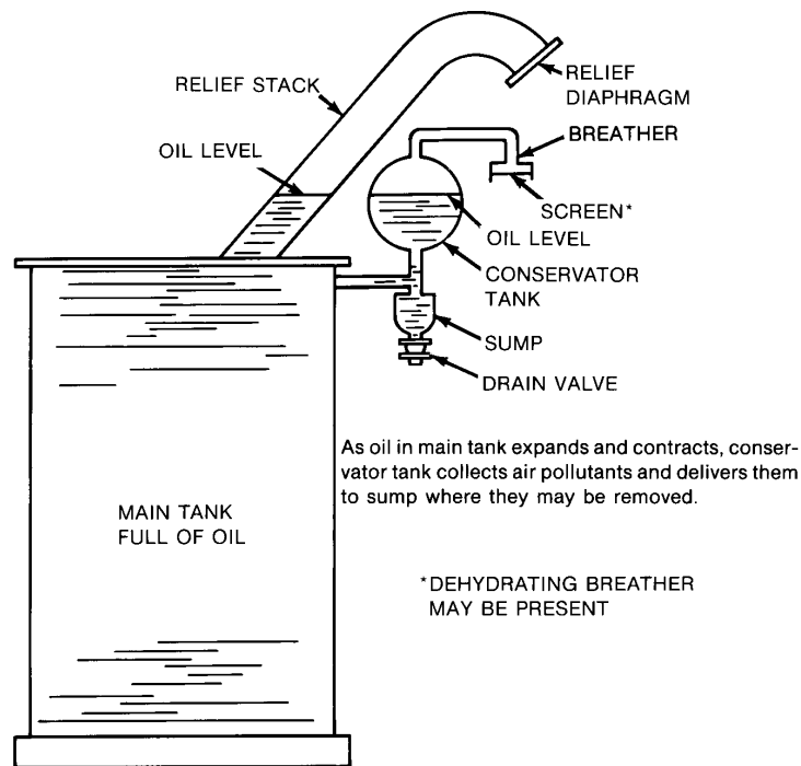
Figure 11-4—Conservator tank oil-preservation system
