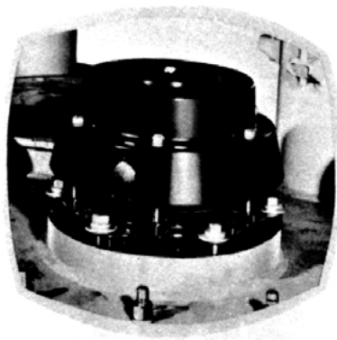
Figure 11-8—Pressure-relief device, which limits internal pressure to prevent tank rupture under internal fault conditions
