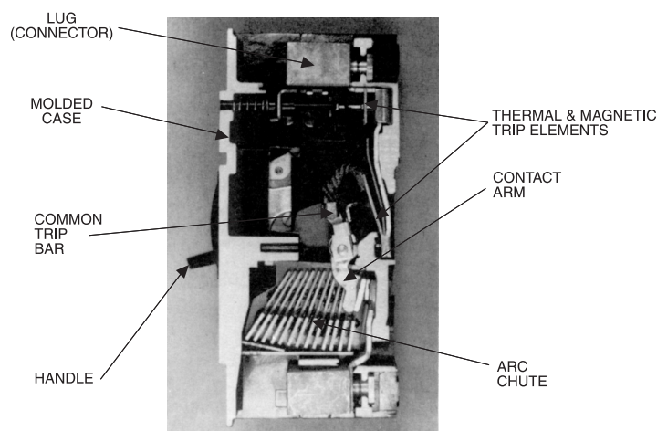
Figure 7-3—Thermal-magnetic trip MCCB
