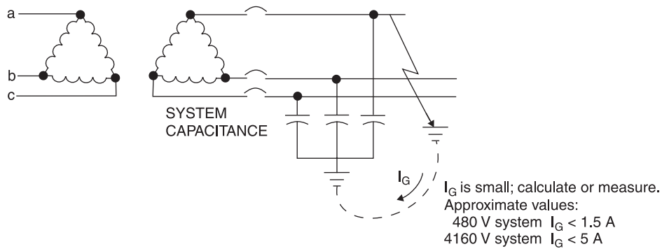
Figure 8-5a—Ungrounded system (uses bus ground detector to alarm and has potential for possible overvoltage problem)
