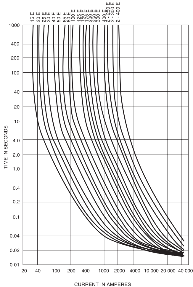
Figure 6-11—Typical total-clearing TCC curves for high-voltage solid-material power fuses (see Figure 6-9)
