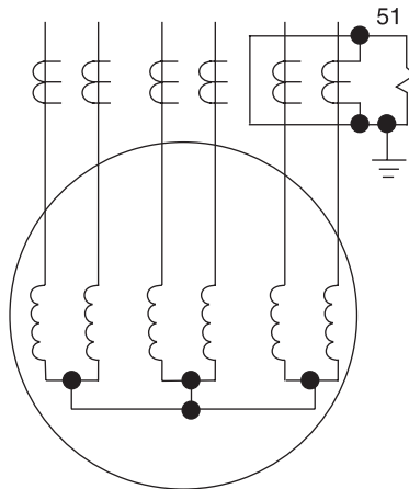
Figure 10-12—Split-phase motor overcurrent protection used with two paths per phase (one relay shown)
