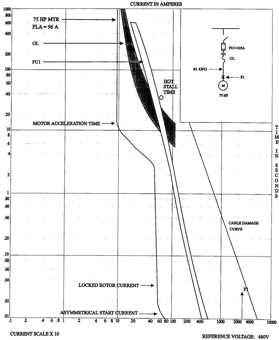
Figure 15-3a—Motor overload coordination plot using combination overload relay and fuse
