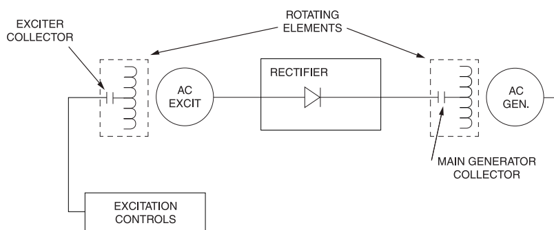
Figure 12-5—System with alternator-rectifier exciter and stationary exciter
