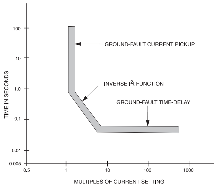
Figure 7-8b—Ground-fault TCC curve ( I^2t IN) for electronic trip circuit breaker
