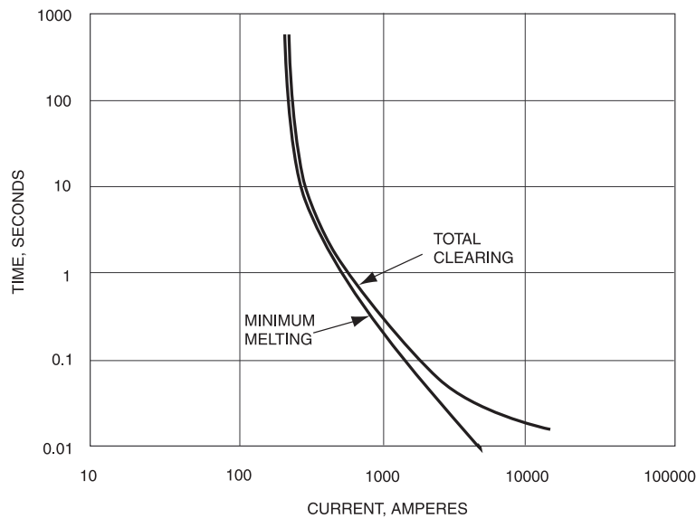
Figure 6-3—Typical TCC curves for an expulsion fuse
