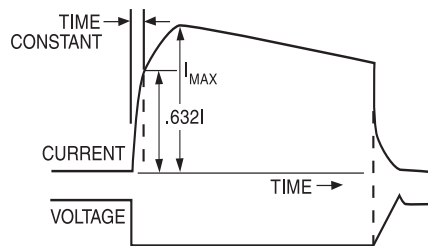
Figure 5-25—Time constant for dc circuits per UL 198L-1995
