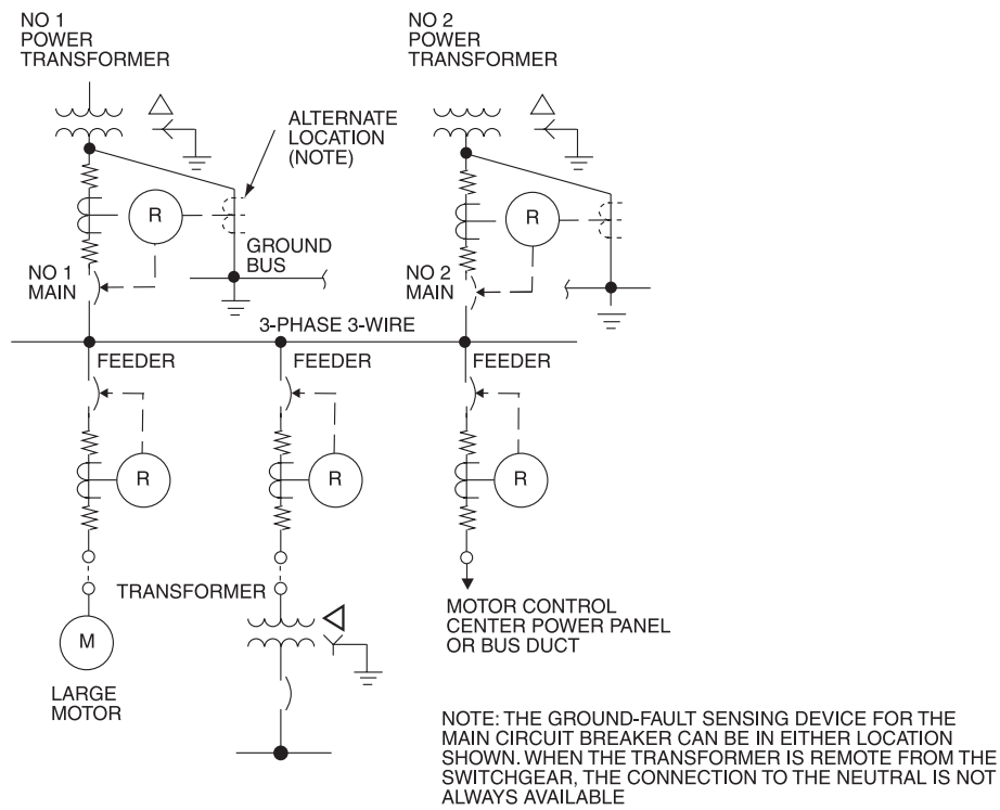
Figure 8-18—Three-wire solidly grounded system with dual supply
