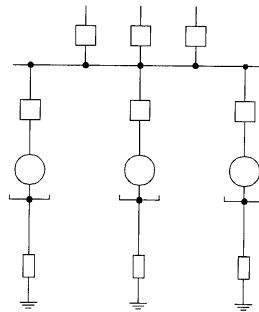
Figure 12-1—Generators connected directly to a distribution system
