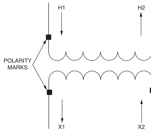
Figure 3-6—CT polarity diagram
