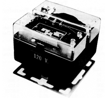
Figure 3-11 — Typical VT
