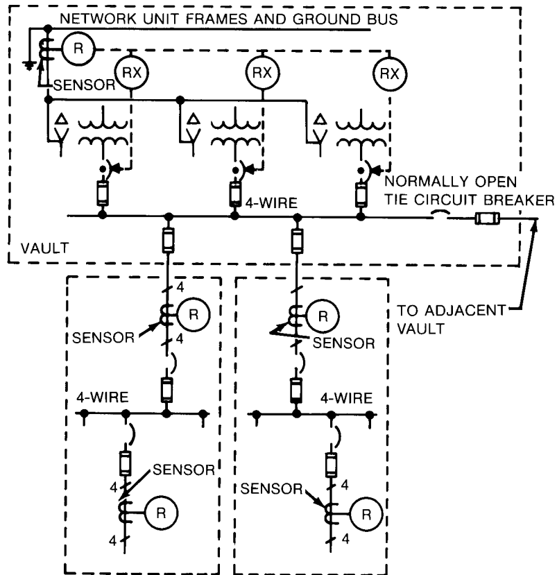
Figure 8-31 — Ground-fault protection for sectionalized vault bus spot network
