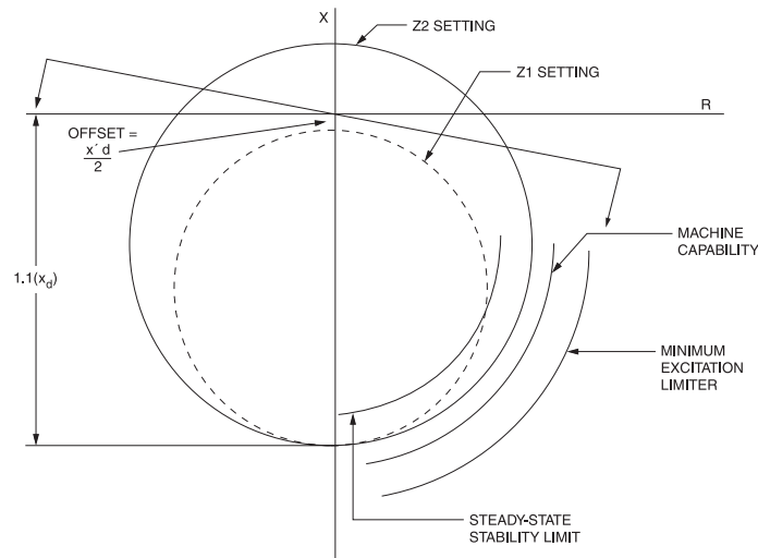
Figure 12-27—Loss-of-excitation protection using impedance, directional, and undervoltage units
