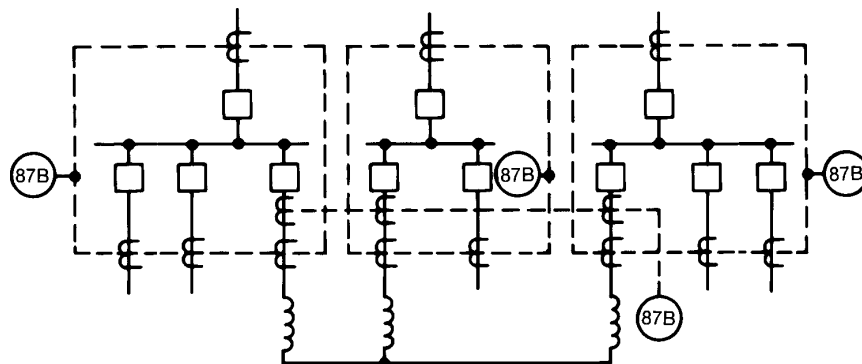
Figure 13-4—Synchronizing-bus scheme with bus differential relaying
