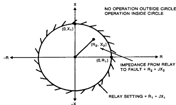
Figure 4-2—R-X diagram for the generic impedance relay
