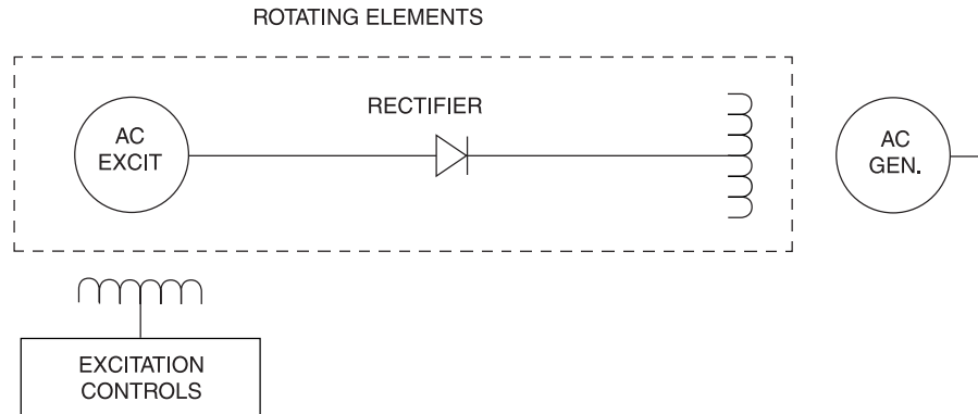
Figure 12-6—System with alternator-rectifier exciter and rotating rectifiers (brushless exciters)
