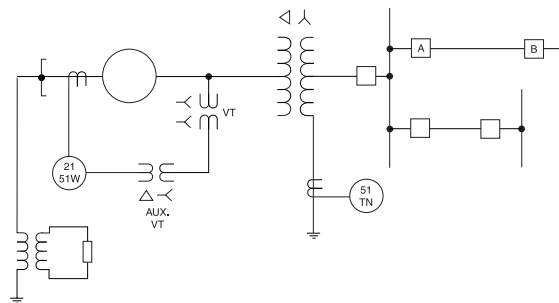
Figure 12-30—Application of system backup relays for unit generator-transformer arrangement
