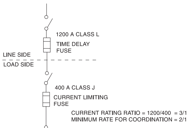
Figure 5-15—Typical application of selective coordination (see Table 5-1)
