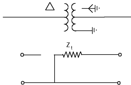
Figure 2-7b—Zero-sequence equivalent circuit for delta-wye-grounded transformer
