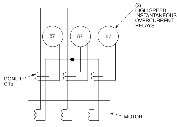
Figure 4-28b—Differential protection of a motor using donut CTs and overcurrent relays
