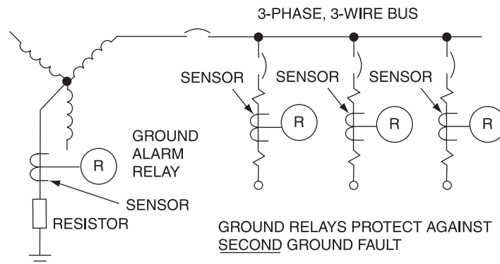
Figure 8-27—High-resistance-grounded system that continues operation on first ground fault while ground relays protect against second ground fault
