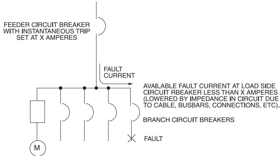
Figure 7-12—Coordinated tripping due to impedance in circuit
