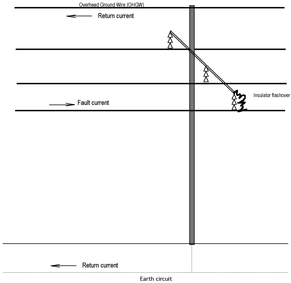
Figure 2-6a—Illustration of insulation flashover on open wire line showing return current flowing through OHGW of transmission line and through earth
