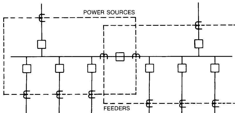
Figure 13-2—Sectionalized-bus scheme with bus differential relaying
