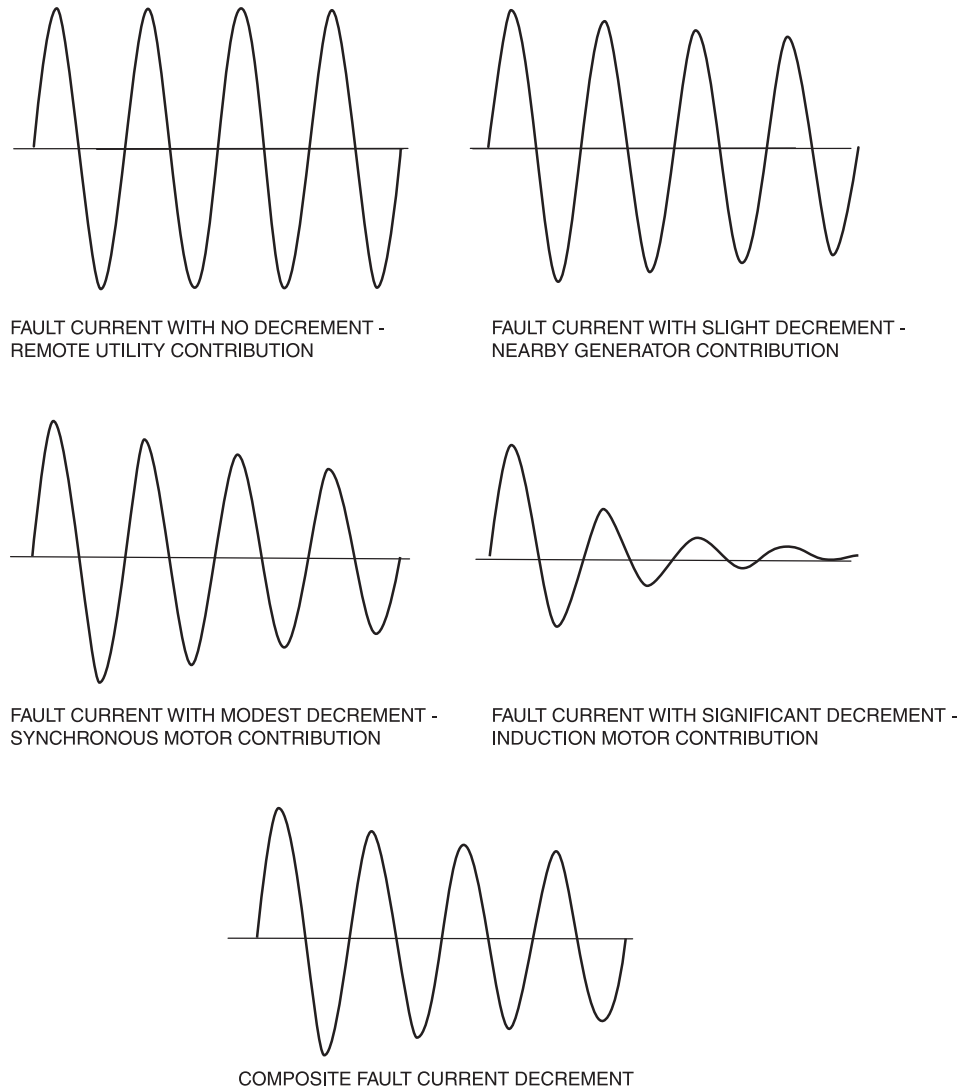
Figure 2-3—Generic components of fault current categorized according to decrement
