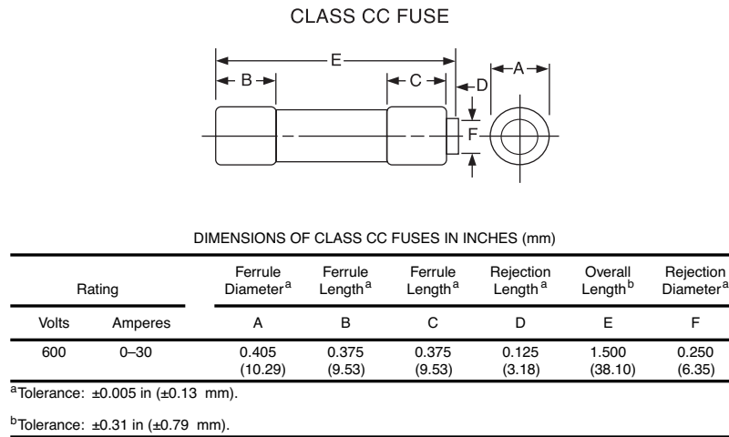
Figure 5-9—Class CC fuse dimensions
