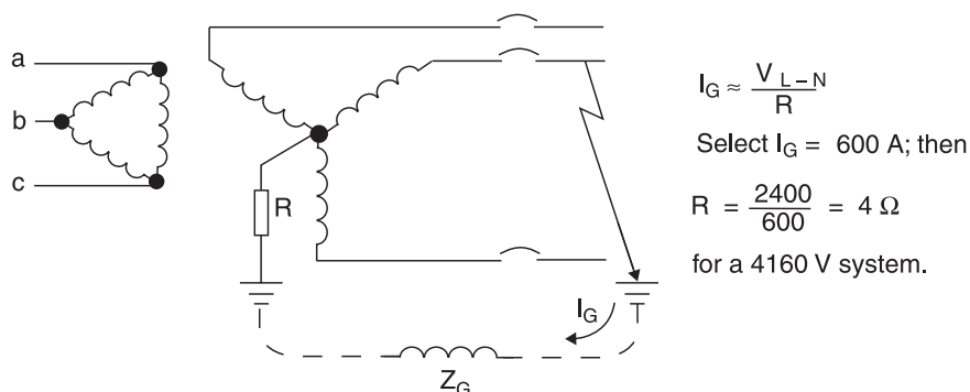
Figure 8-3—Low-resistance grounding (uses ground relays to trip)
