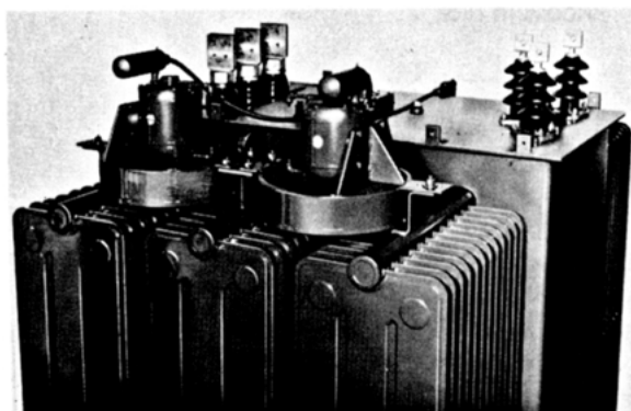
Figure 11-17—Forced-air fans, normally controlled automatically from a top oil temperature or winding temperature relay
