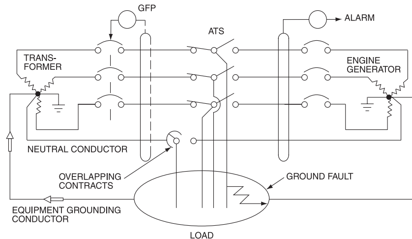
Figure 8-16—Emergency power systems with ground-fault protection on normal and ground-fault alarm on emergency
