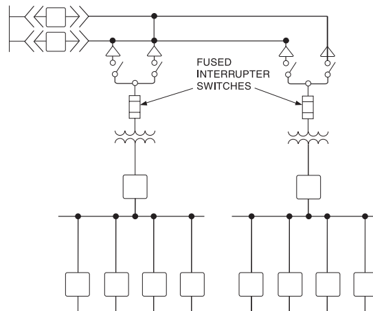
Figure 6-7—One-line diagram of typical primary-selective system
