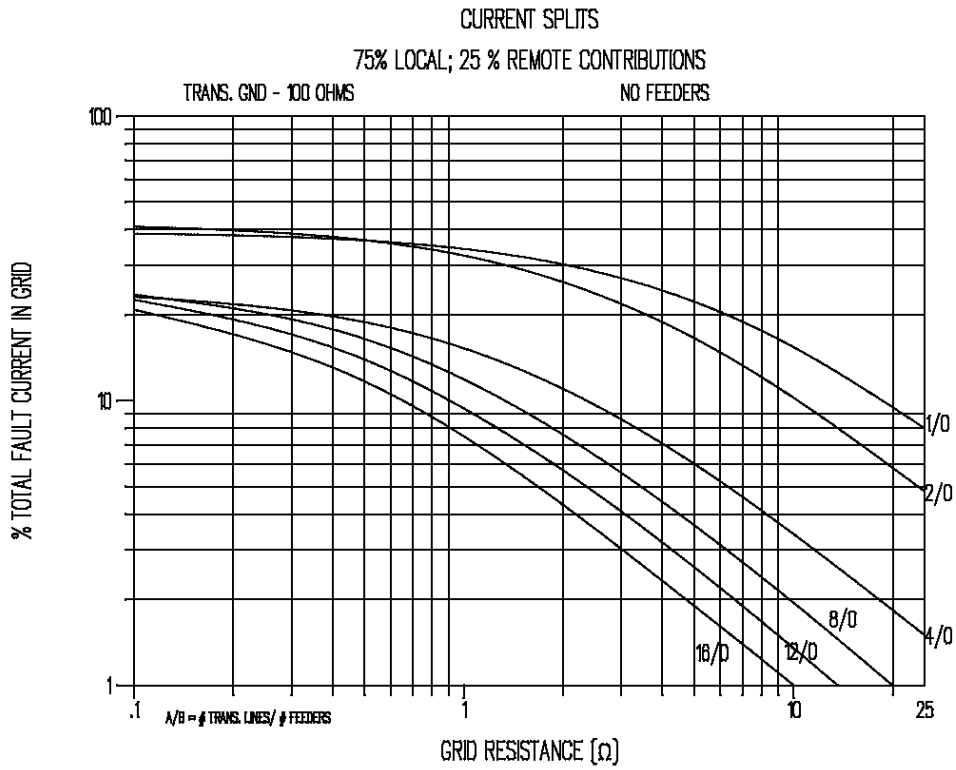
Figure C.22—Curves to approximate split factor S_f
