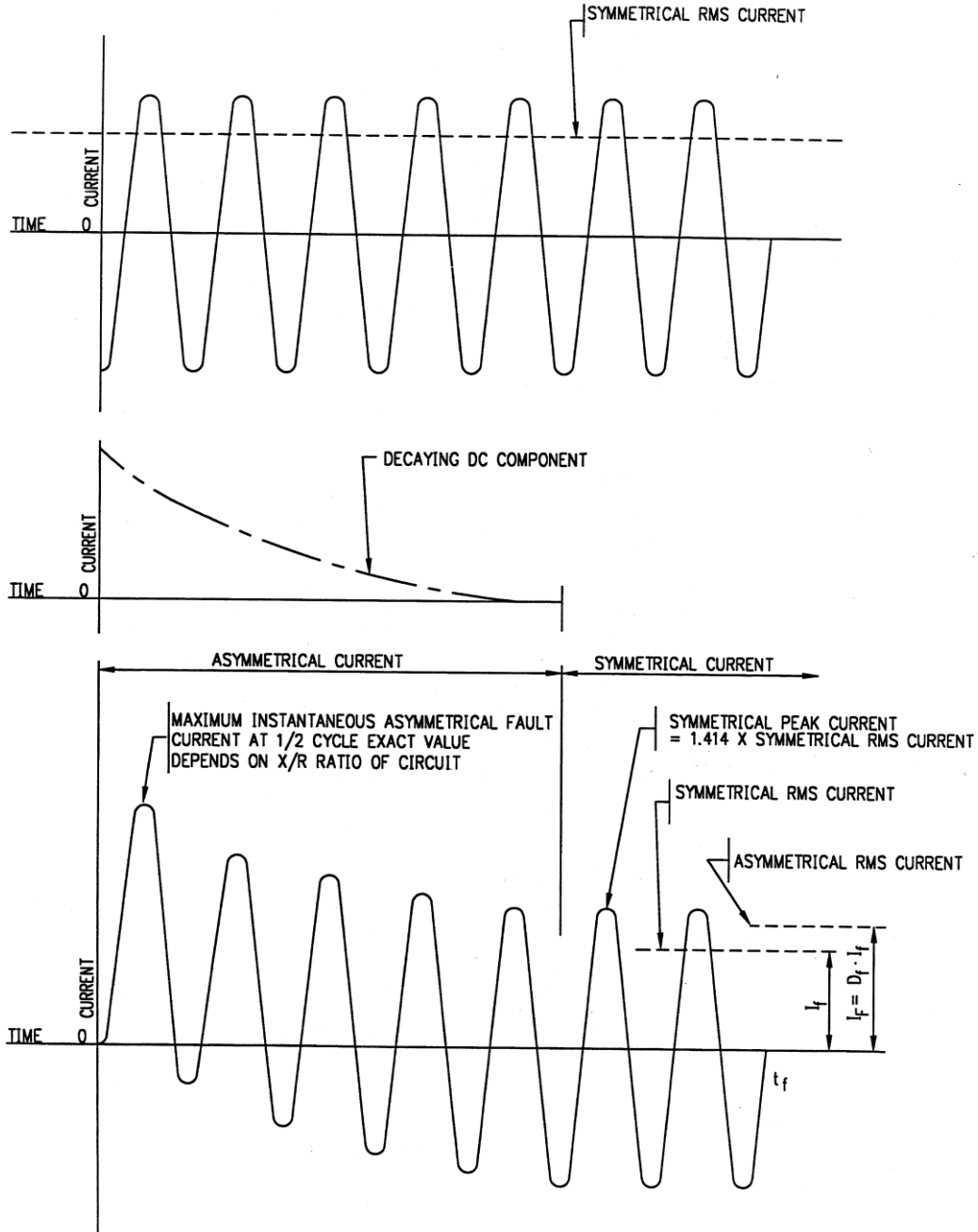
Figure 1—Relationship between actual values of fault current and values of I_F , I_{fb} , and D_f for fault duration t_f
