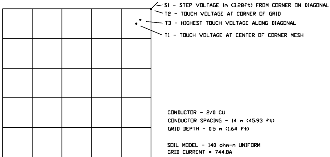
Figure H.3—Grounding system parameters for Grid 1
