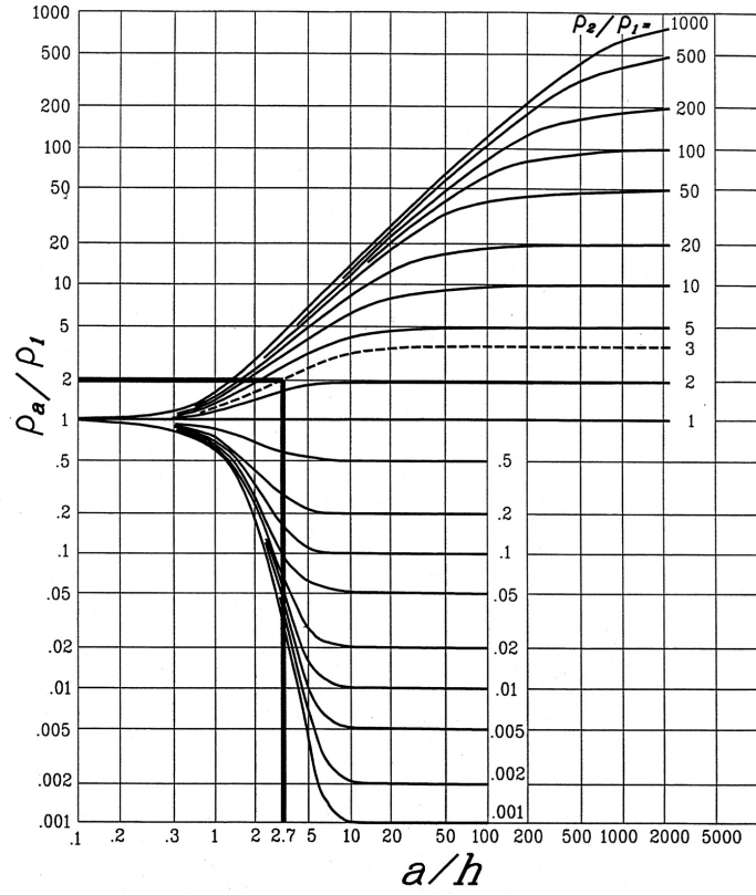
Figure 22—Example of Sunde's graphical method
