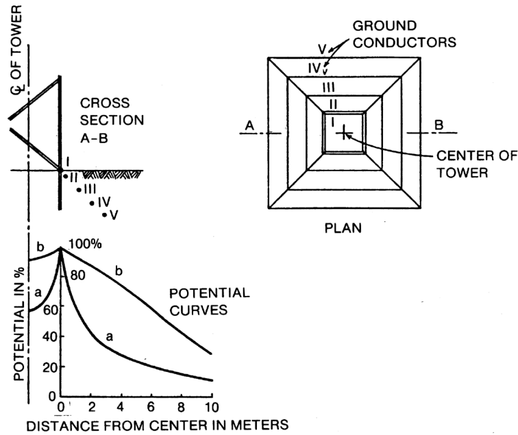
Figure G.10 Potential distribution around a mast in the direction A-B for a mast with ramp (Curve b) and without ramp (Curve a)
