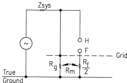
Figure 7—Impedances to touch voltage circuit
