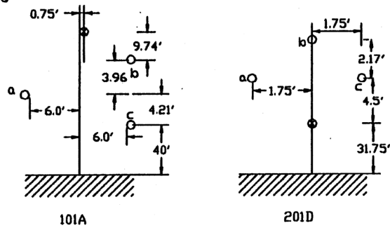
Figure 31—Example system for computation of current division factor S_f
