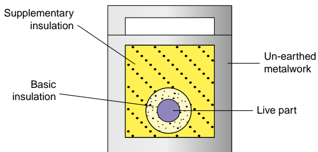
FIGURE 3.5 Class II equipment.
