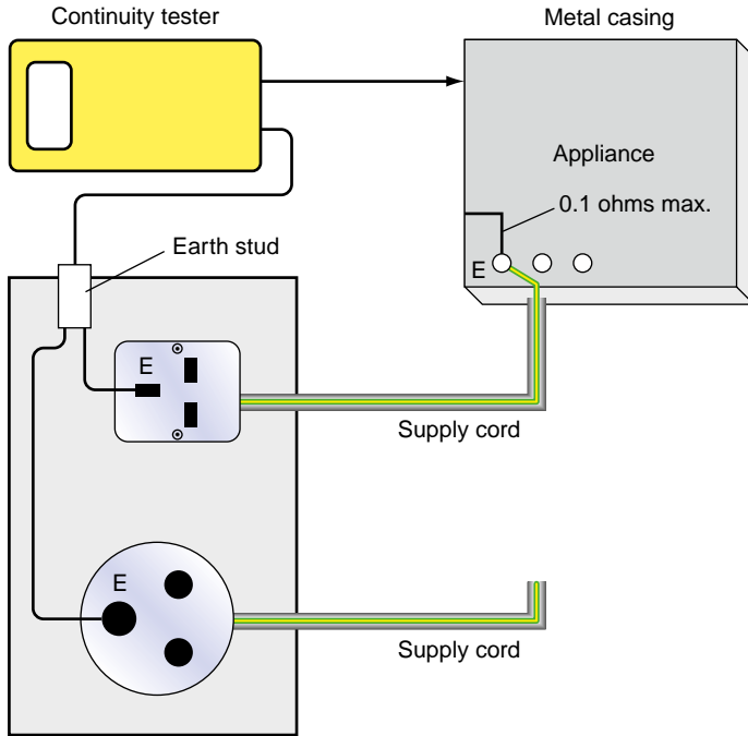
FIGURE 5.3 Typical continuity test box.
