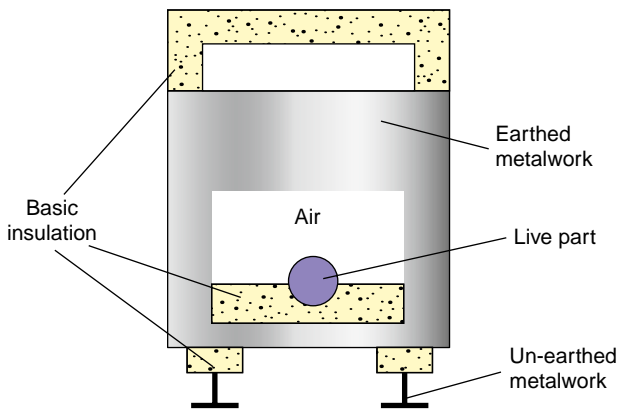
FIGURE 3.2 Class I equipment.
