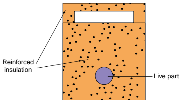
FIGURE 3.4 Class II equipment.
