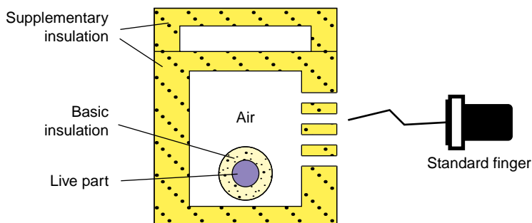
FIGURE 3.6 Manufacturers penetration test.
