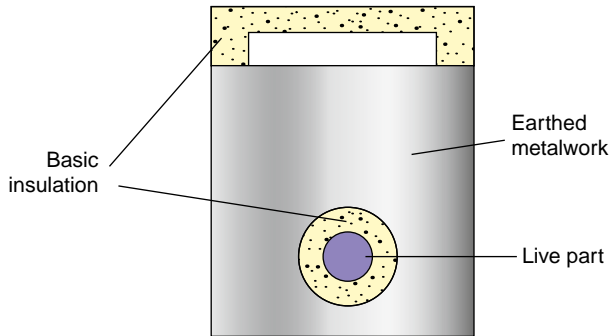
FIGURE 3.1 Class I equipment.
