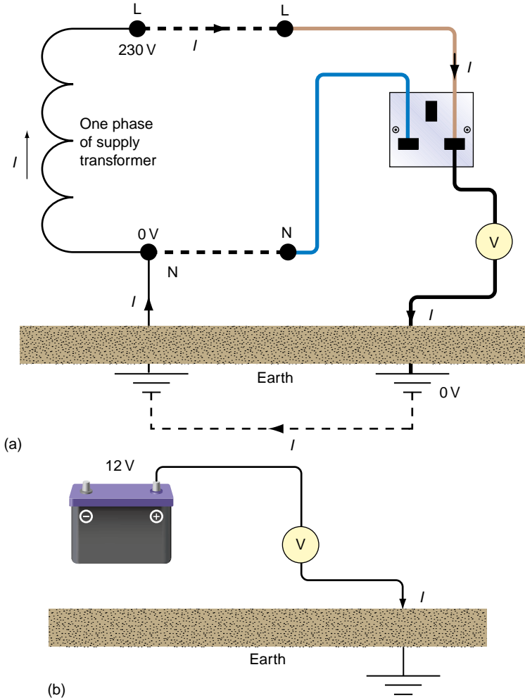
FIGURE A1.2 (a) Return path via Earth; (b) No return path via Earth.
