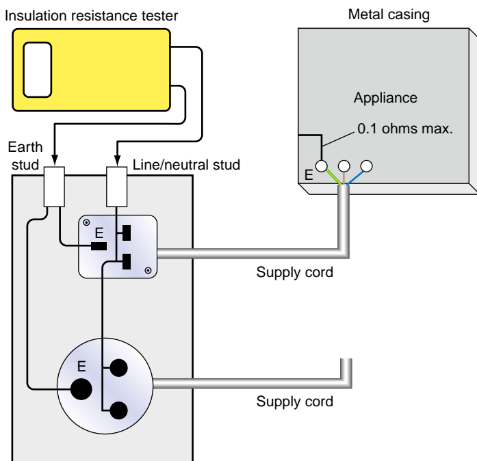
FIGURE 5.4 Typical continuity and insulation test box.
