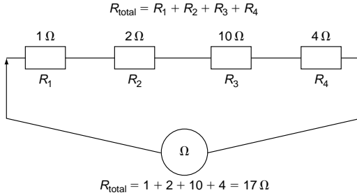
FIGURE A2.1 Resistances in series.
