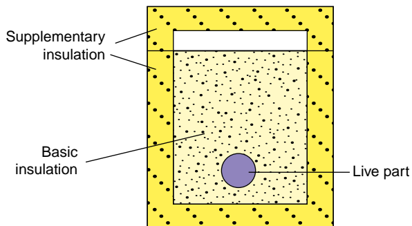
FIGURE 3.3 Class II equipment.
