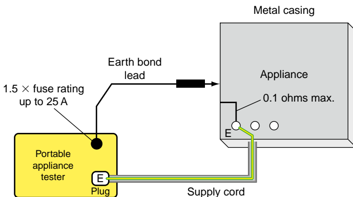
FIGURE 5.1 Continuity test with portable appliance tester.
