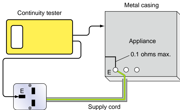
FIGURE 5.2 Continuity test with continuity tester.
